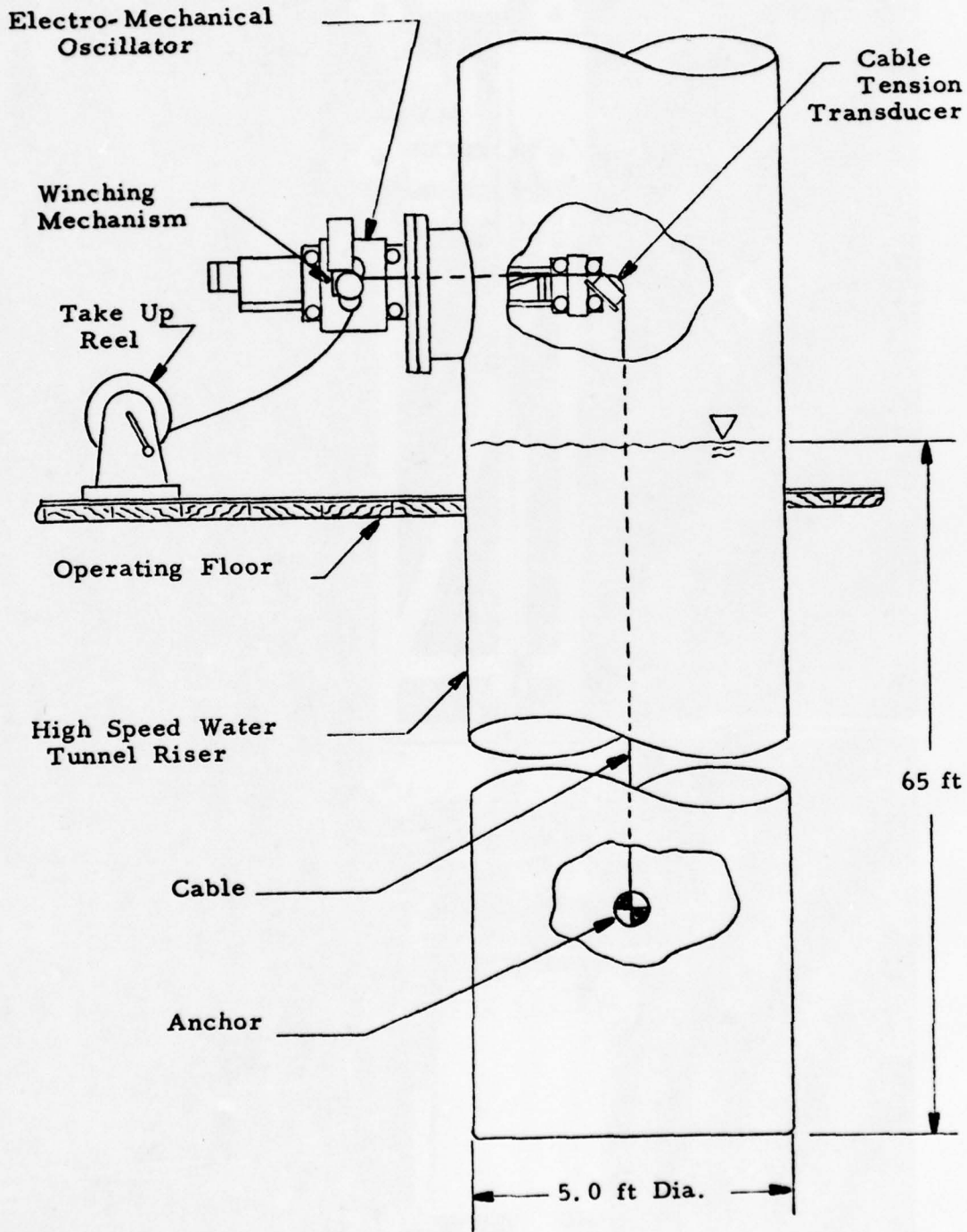
Figure 1. Experimental Arrangement
