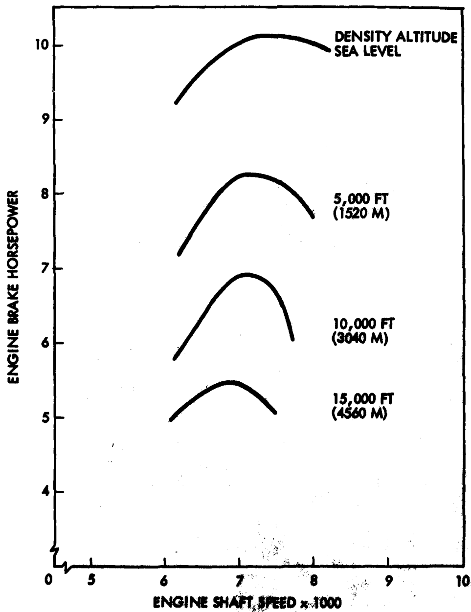
Figure 26. Engine Horsepower - Single Carburetor
