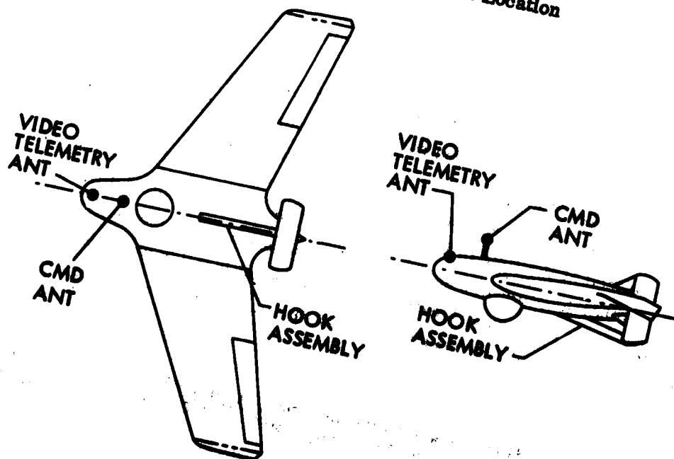
Figure 66. Antenna Location Mod A
