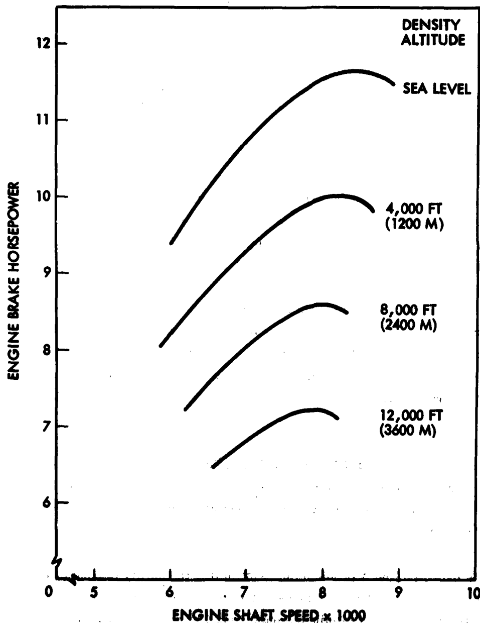
Figure 28. Engine Horsepower - Dual Carburetors
