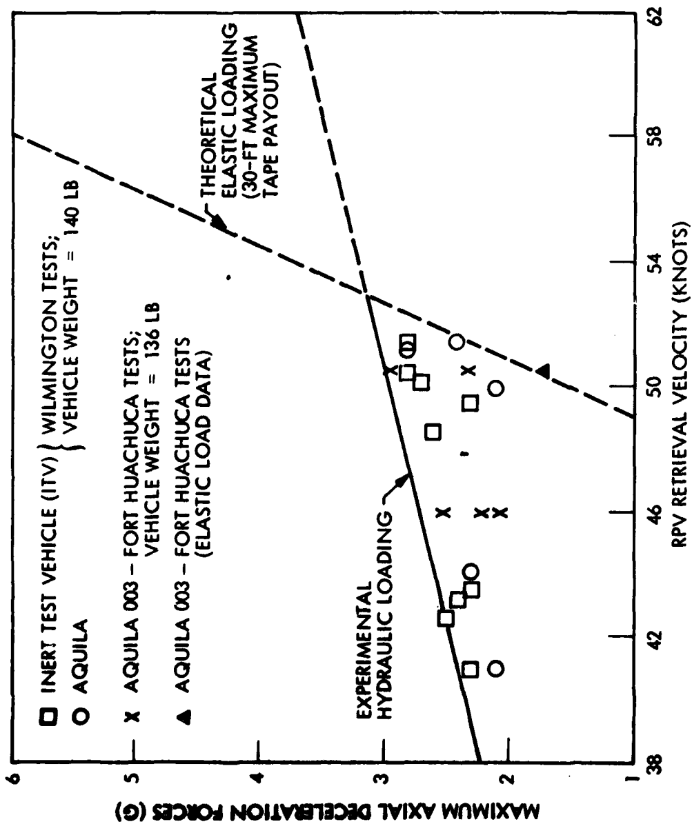
Figure 102. Maximum Axial Deceleration Loads Imposed on RPV by Vertical Barrier
