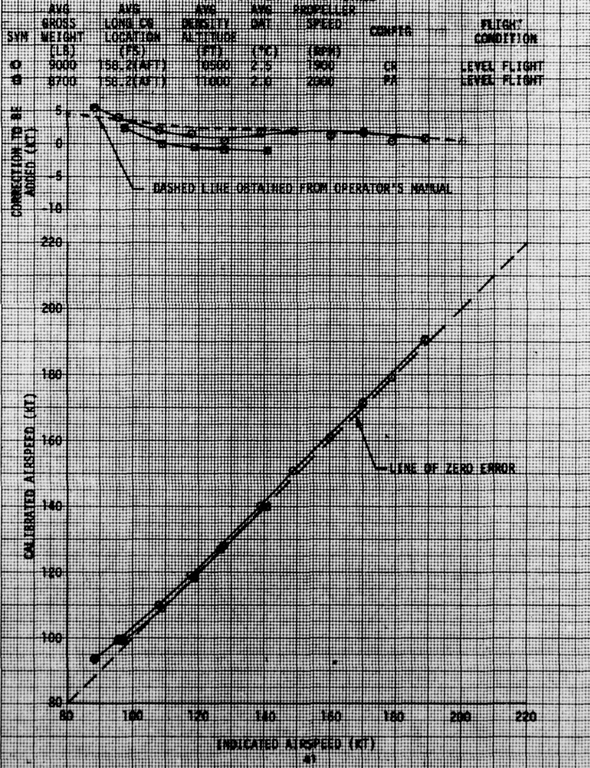
FIGURE 10 AIRSPEED CALIBRATION RU 21W USA S/N 70-15887 SHIP SYSTEM - FACE METHOD
