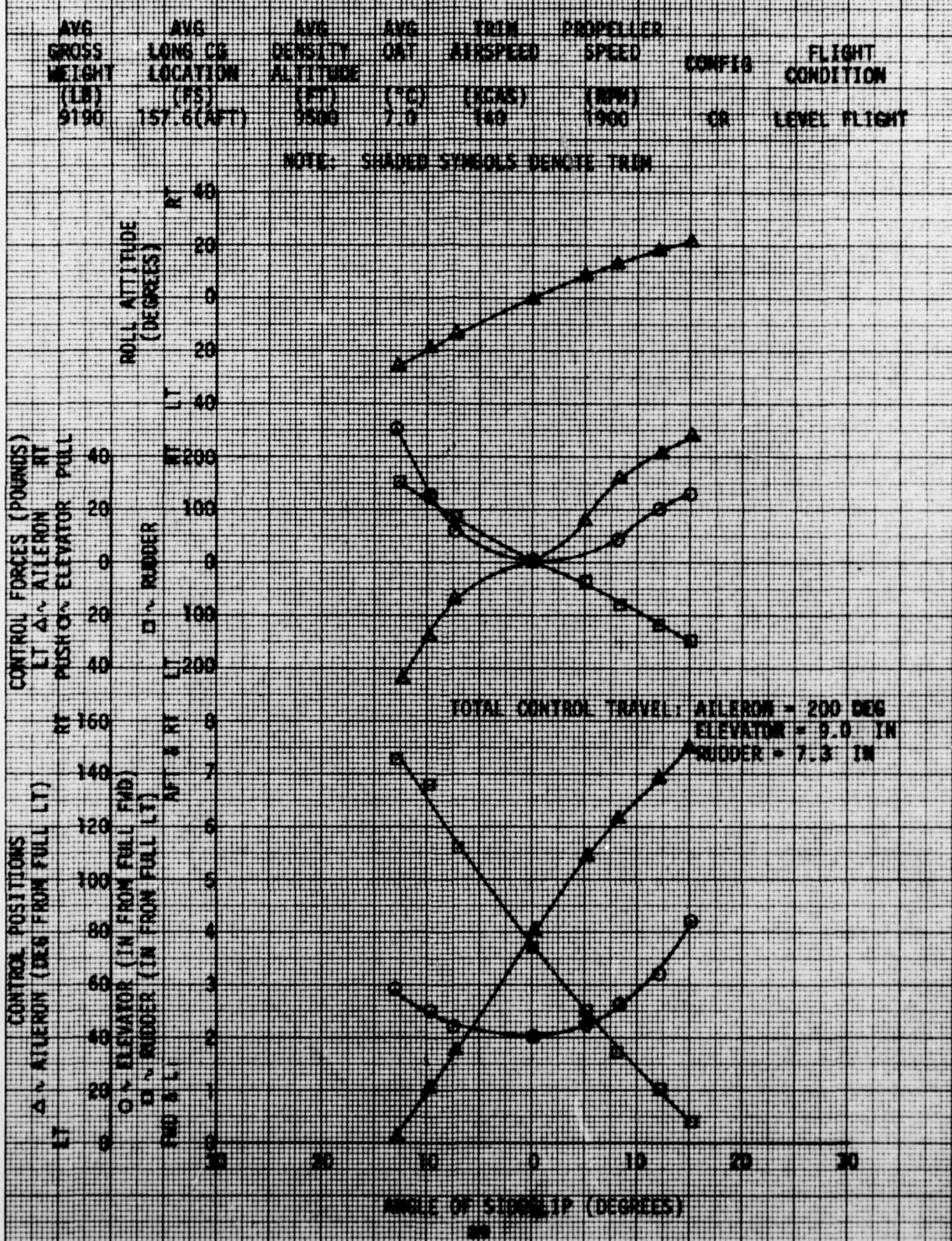
FIGURE 8 STATIC LATERAL-DIRECTIONAL STABILITY WU-21X USA 1/11 70-10007
