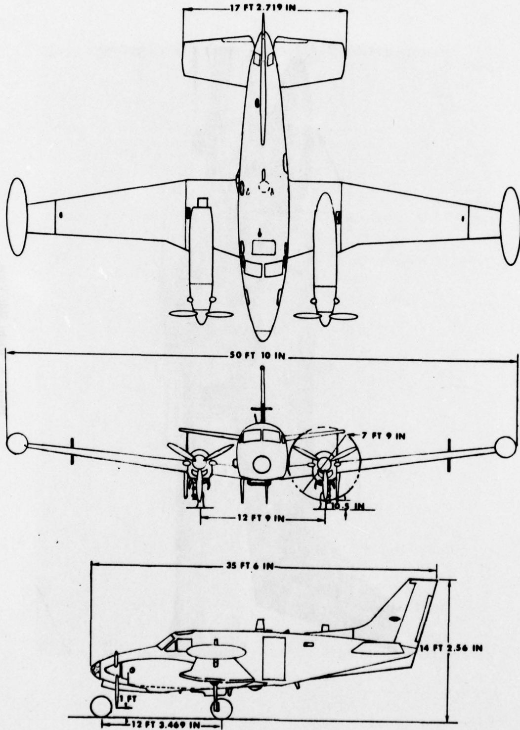
Figure 1. Three View Drawing, RU-21H Guardrail V Airplane
