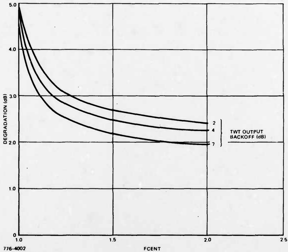
Figure 7-41. Degradation Produced by Hard Limited Transmitters and Phase II TWT at E_b/N_o = 10 dB
