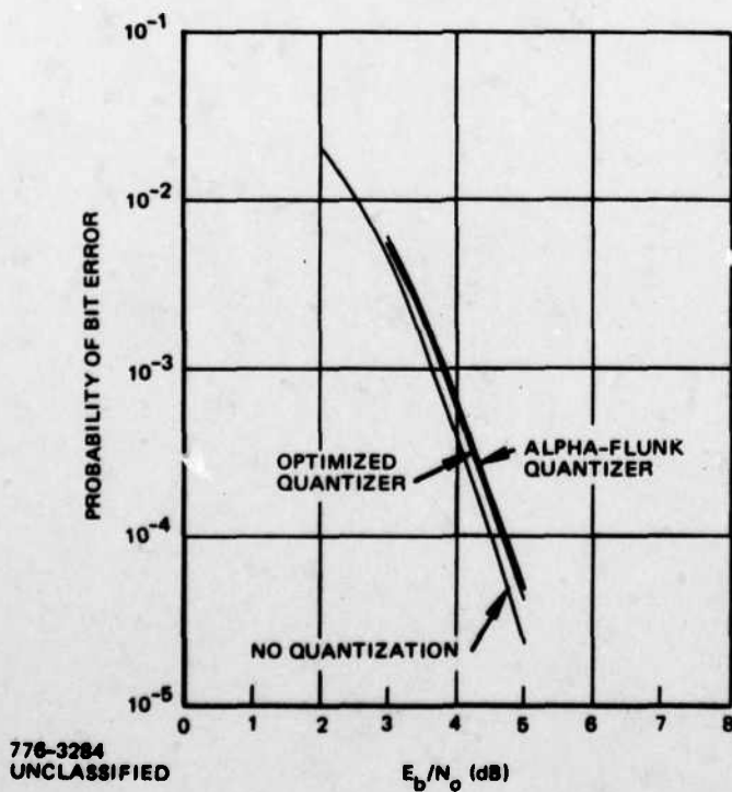
Figure 4-3. Performance of Viterbi Decoder on Ideal Channel With Unquantized Inputs and Inputs Quantized to 3 Bits With Two Different Level Spacings
