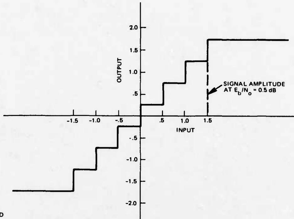
Figure 5-19. Optimum 3-Bit Quantization for Modem Soft Decisions
