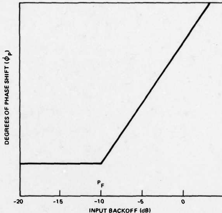
Figure 3-11. Linear AM-PM Conversion Characteristic (PHASE = 3)
