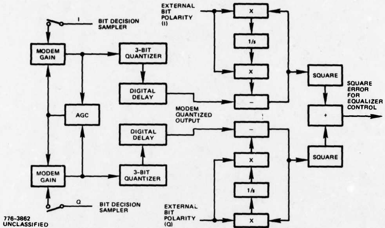
Figure 5-22. Externally-Directed Error With Modem Quantization
