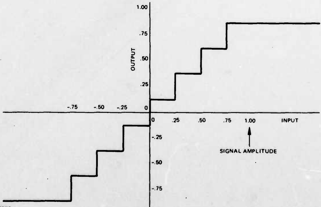
Figure 3-14. 3-Bit Quantization for "Alpha Flunk" Information
