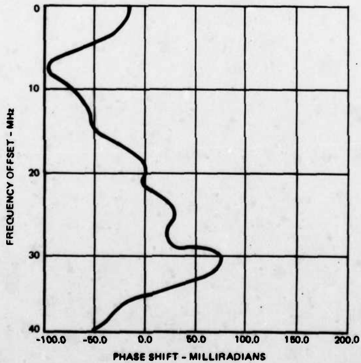
Figure 2-9. Receive Phase Distortion - AN/TSC-54
