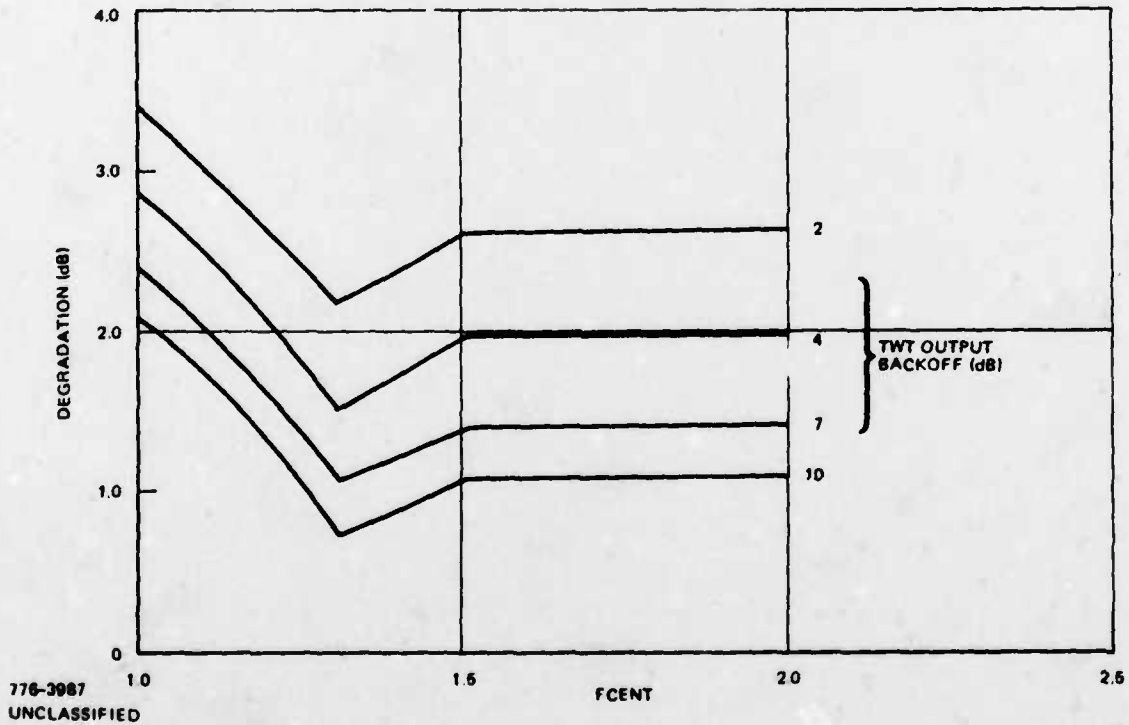
Figure 7-26. Degradation With Equalized Filters at E_b/N_o = 10 dB
