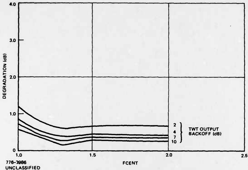
Figure 7-25. Degradation With Equalized Filters at E_b/N_o = 2 dB
