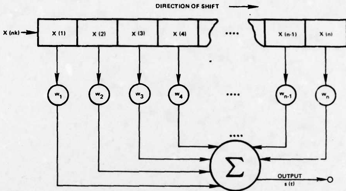
Figure C-1. Transversal Filter
