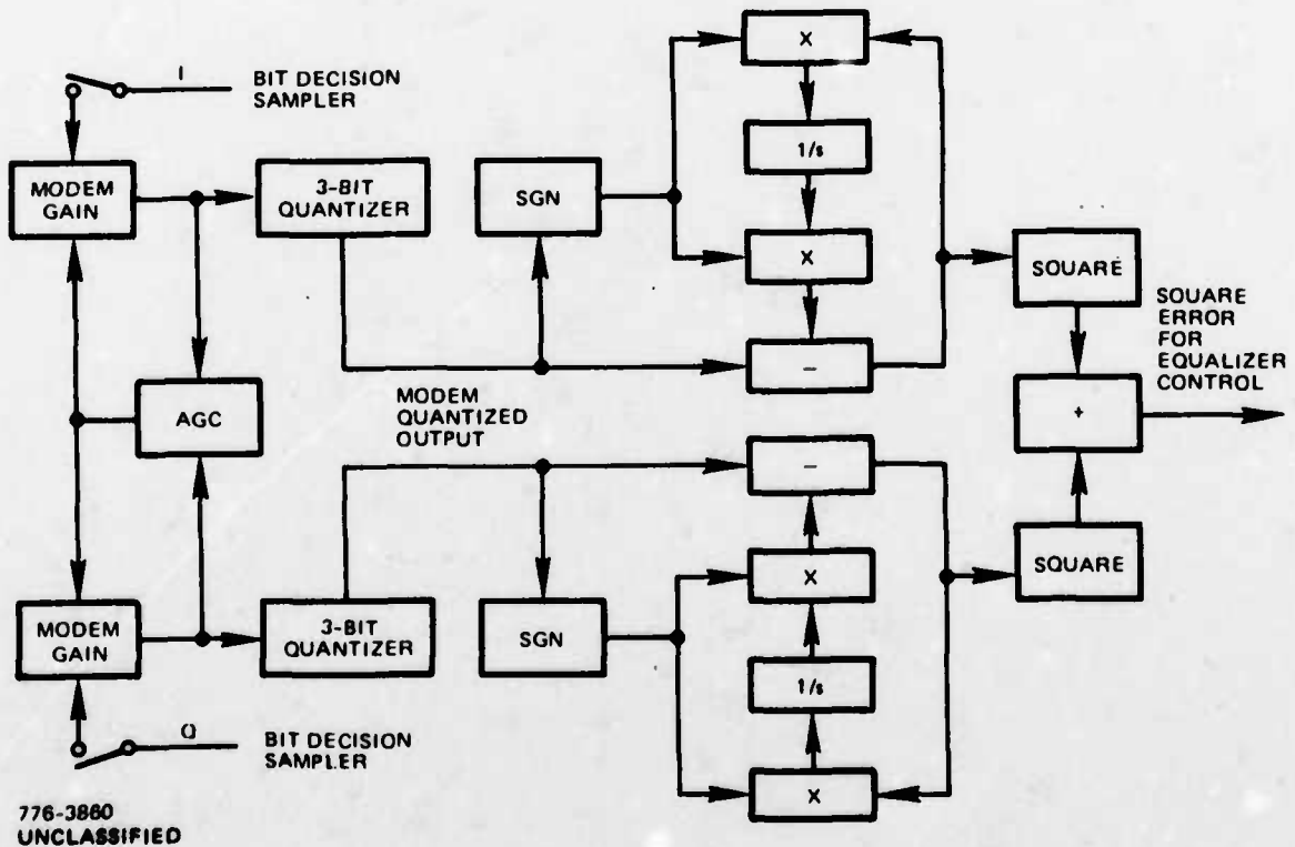
Figure 5-20. Decision-Directed Error With Modem Quantization
