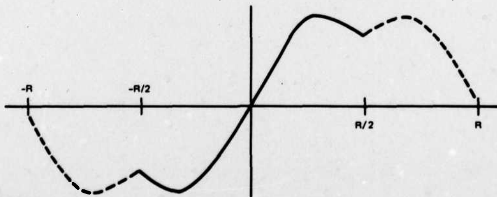
Figure B-12. Representation of an Instantaneous Voltage Transfer Function by a Fourier Series
