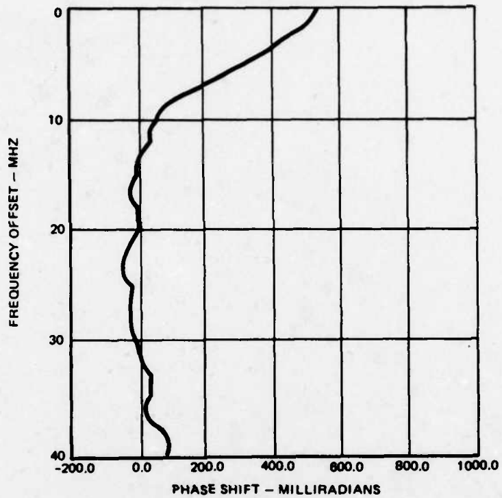
Figure 2-8. Receive Phase Distortion - AN/TSC-54
