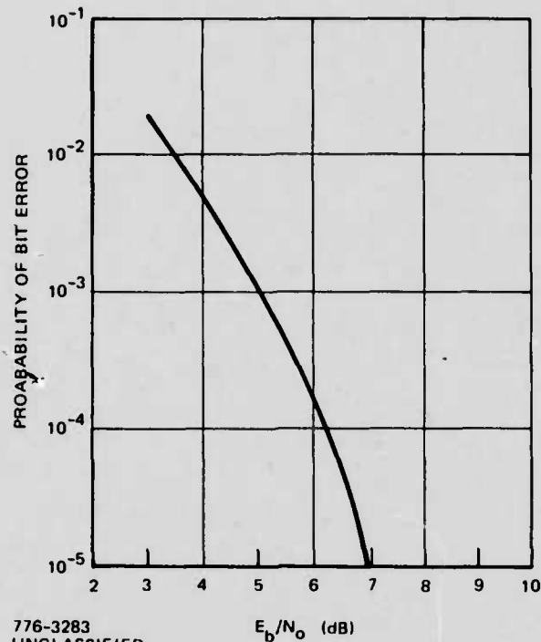
Figure 4-2. Performance of Coding With Filtered Adjacent Channel Signals Each 20 dB Above Center Channel. Channel Spacing FCENT = 2/T_b . Coding Parameters: R = 1/2 , K = 5 , M = 15 , Mode = Serial.
