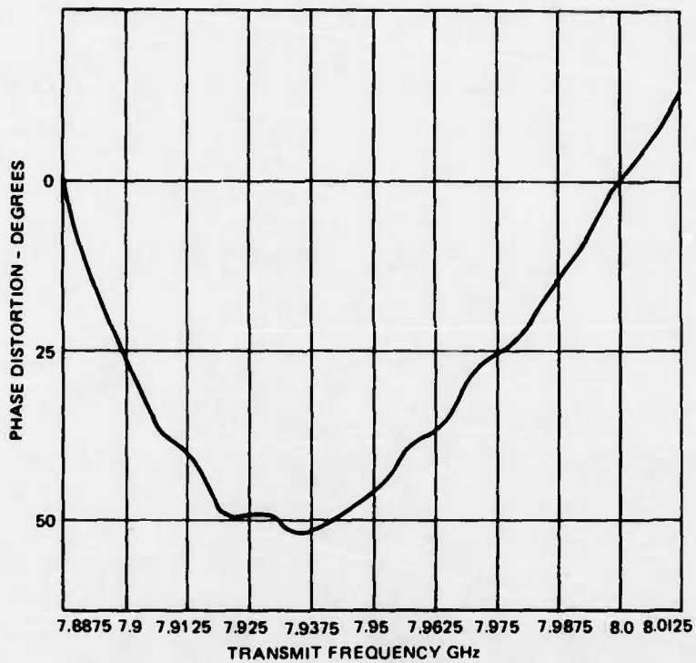
Figure 2-1. Integrated Group Delay Curve - Band 1 of AN/MSC-46 Transmitter
