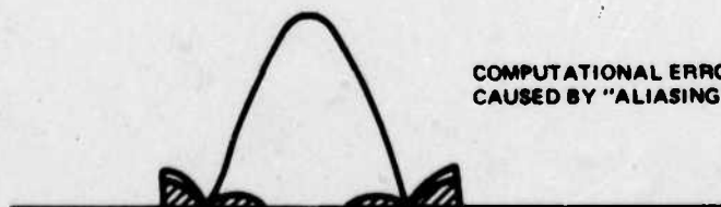
Figure 3-6C. Filtered Signal Spectrum in FFT Representation, Sampling Rate S=3
