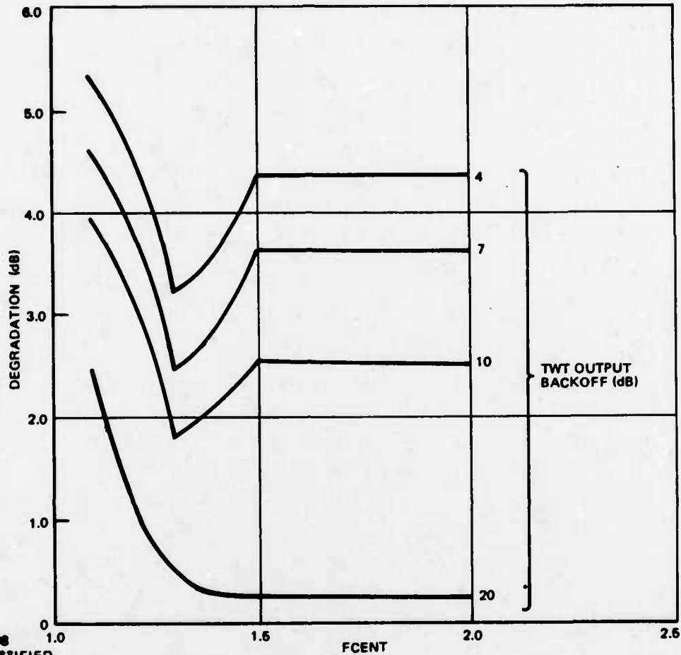
Figure 7-37. Degradation With TWT and Equalized Filters at E_b/N_o = 10 dB
