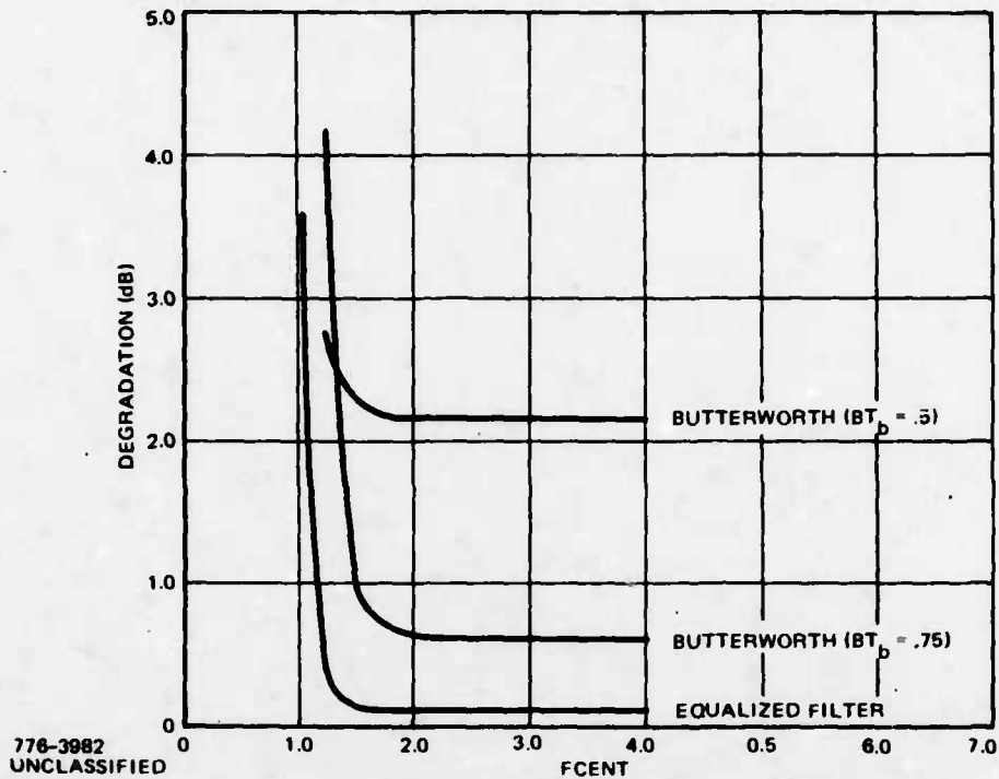
776-3982 UNCLASSIFIED Figure 7-17. System Degradation as a Function of Signal Spacing at E_b/N_o = 10 dB. (Linear Channel, Adjacent Signals +6 dB)
