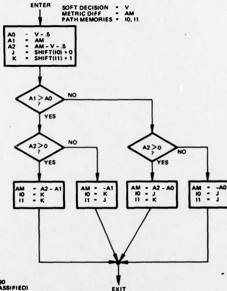
Figure 9-3. Flowchart of Viterbi Algorithm Correction for Duobinary Demodulation
