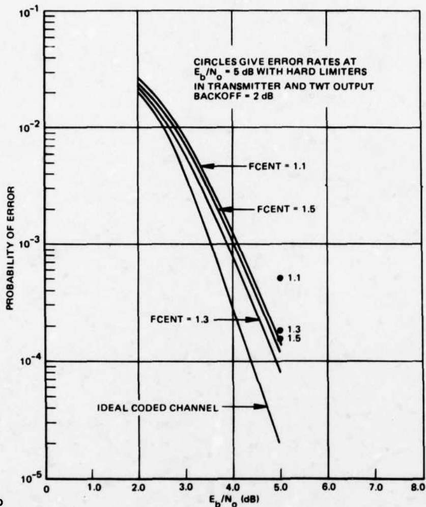
Figure 7-50. Probability of Error Versus E_b/N_0 as a Function of Signal Separation for TWT Output Backoff = 2 dB (Code Rate = 1/2, Equal Signal Levels)
