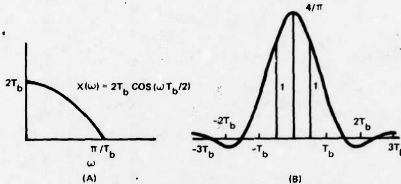
Figure 9-1. (a) Duobinary Filter and (b) Its Impulse Response
