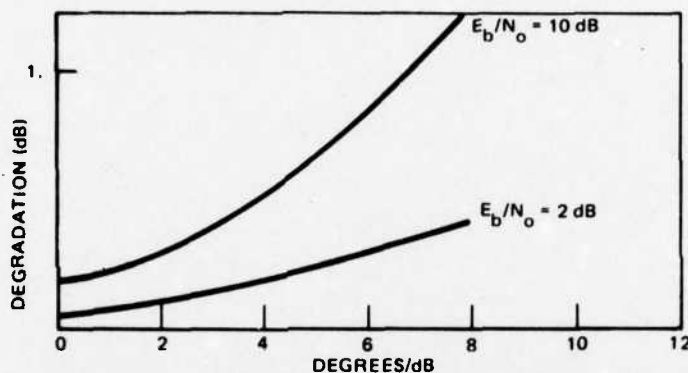
Figure 8-2. Degradation for Single SQPSK Signal as a Function of AM/PM Conversion
