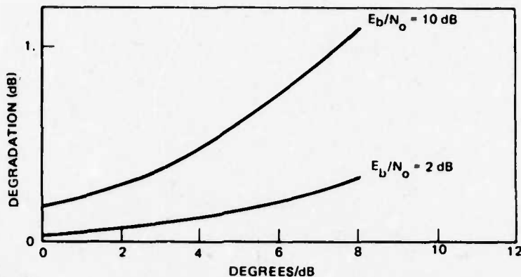
Figure 8-1. Degradation for Single QPSK Signal as a Function of AM/PM Conversion
