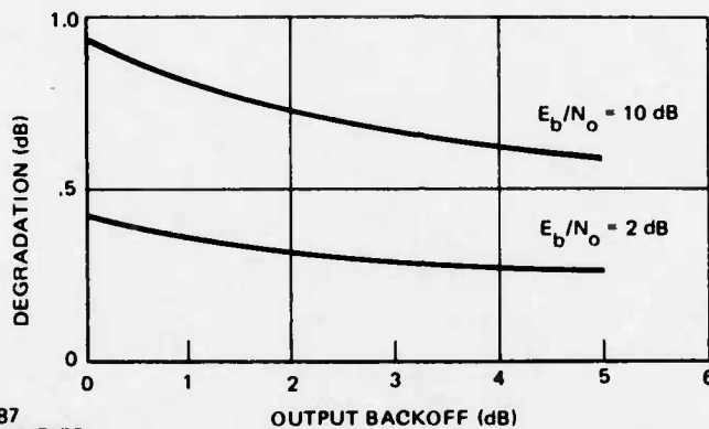
Figure 8-4. Degradation of Single SQPSK Signal With Phase III TWT Backoff
