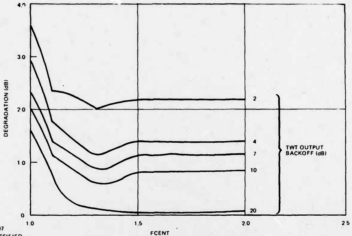
Figure 7-36. Degradation With TWT and Equalized Filters at E_b/N_0 = 2 dB
