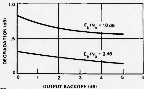
Figure 8-3. Degradation of Single QPSK Signal With Phase III TWT Backoff
