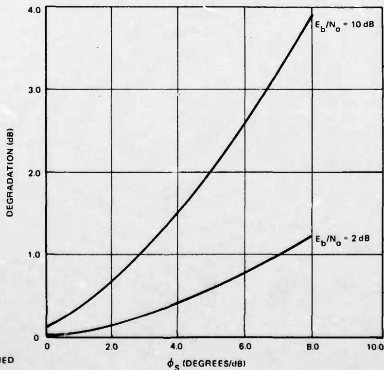
Figure 7-19. Degradation as a Function of Linear AM-PM Conversion for Five Equal Signals (Equalized Filters in Transmitter and Receiver)
