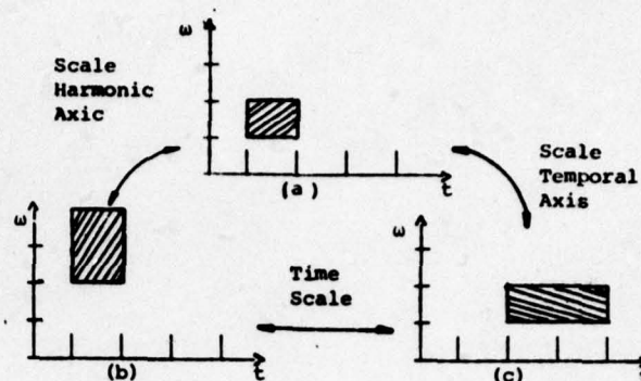
Figure 1. The relationship of axis scaling in the time and spectral domains (a) Original spectral event (b) Harmonically-scaled event (c) Temporally scaled event.
