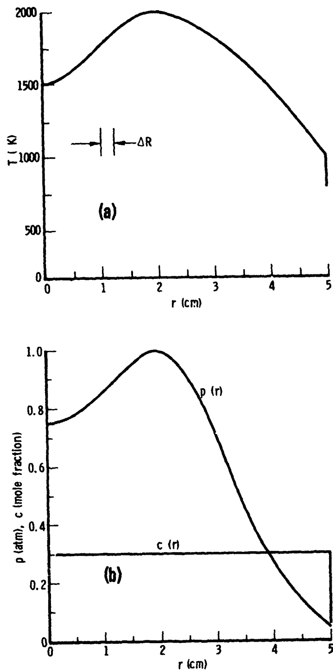
Fig. 33. Radial Profiles for Hypothetical Engine Test Case 1. (a) Temperature; (b) Concentration and pressure.
