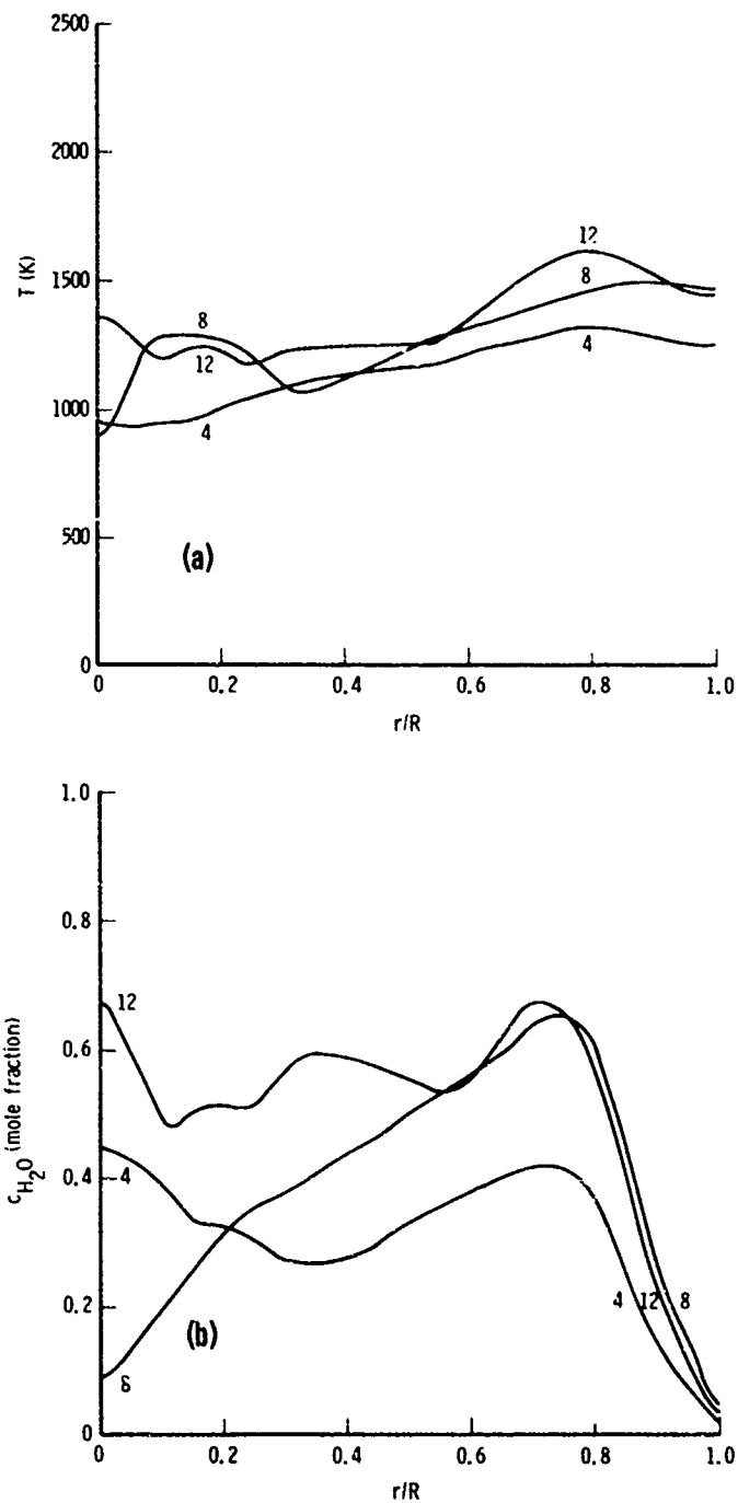
Fig. 84. Transtage Inversion Results for Cases 4, 8 and 12. (a) Temperature; (b) H_2O concentration.
