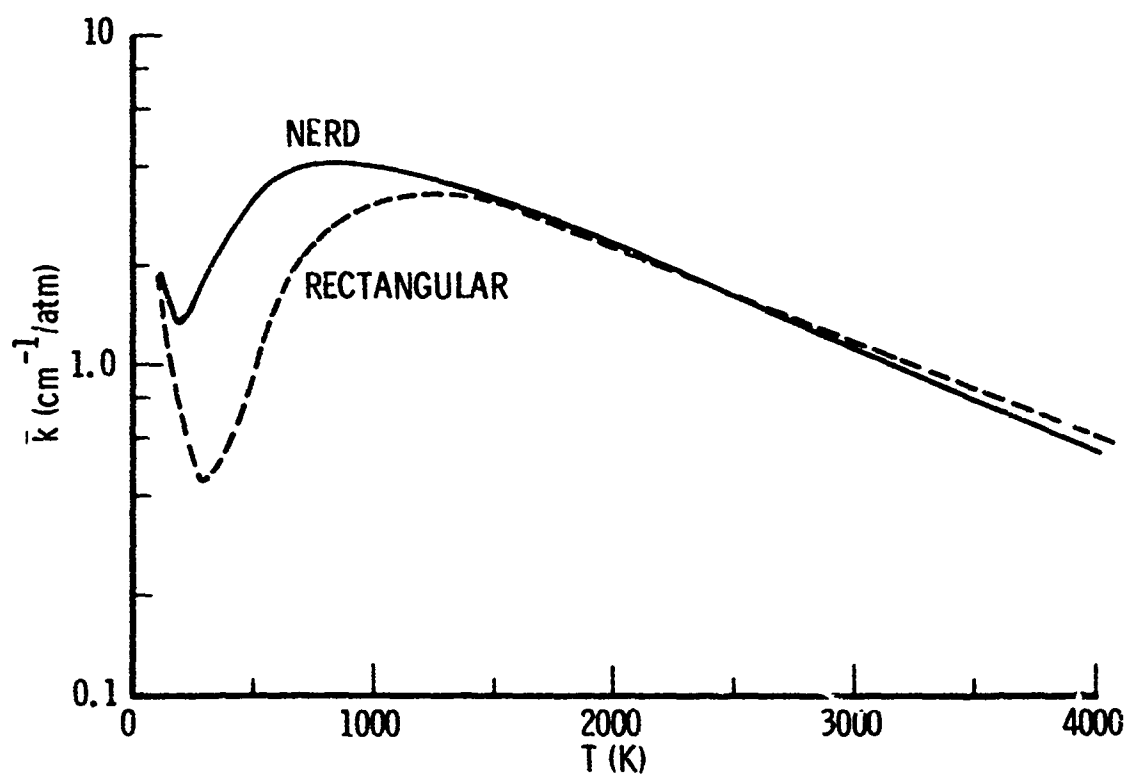
Fig. 12. Absorption Band Model Parameter \bar{k} for \text{CO}_2 Bandpasses
