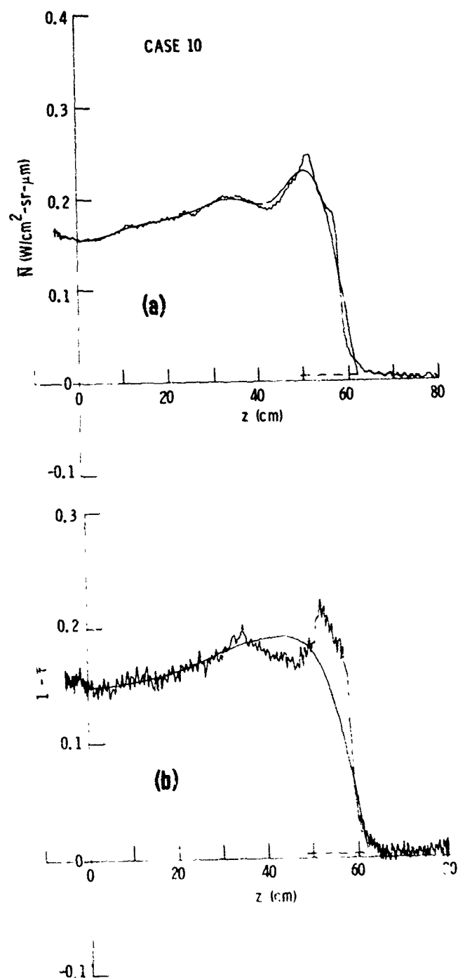
Fig. 73. Transverse E/A Profiles for Transtage Case 10. (a) Raw and smoothed radiance data; (b) Raw and smoothed absorbance data. Dashed lines indicate zero levels.
