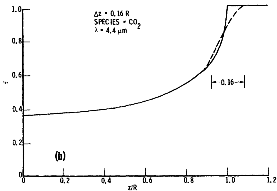
Fig. 62. Convolutions of Transverse E/A Profiles with a Rectangular Field-of-View Slit Function. (a) Radiance; (b) Transmittance.
