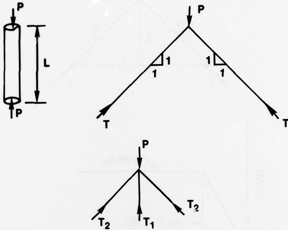
Fig. 3 - Designs using one, two, or three bars
