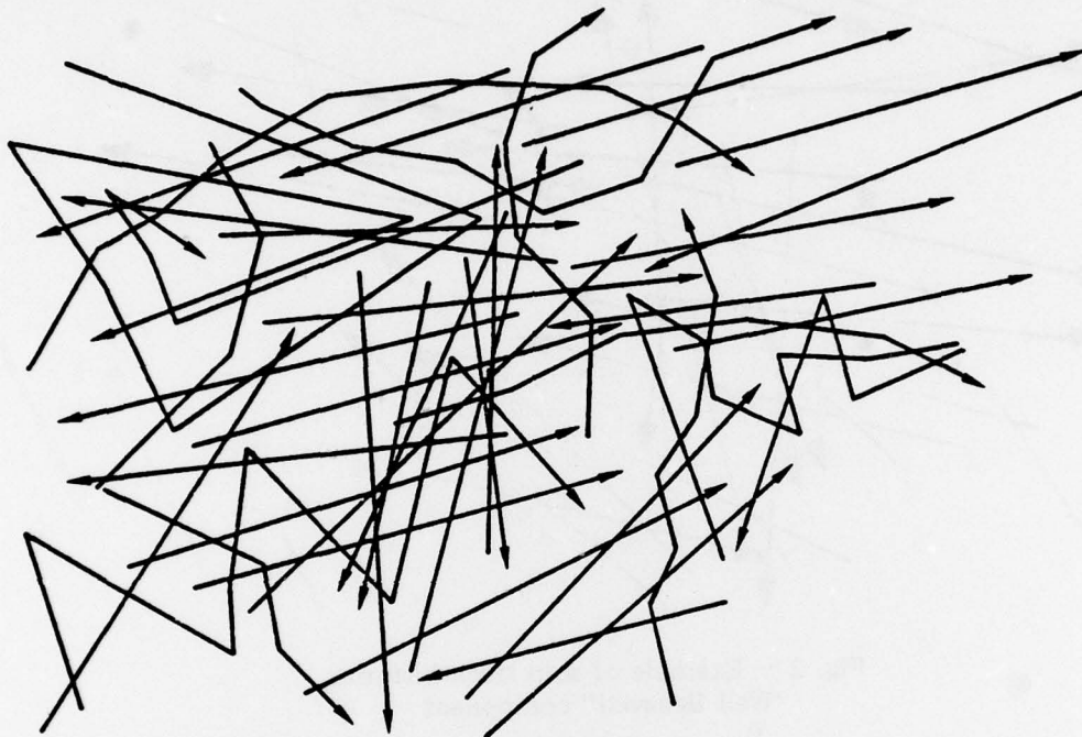
Fig. 1 — Example of ship track histories
