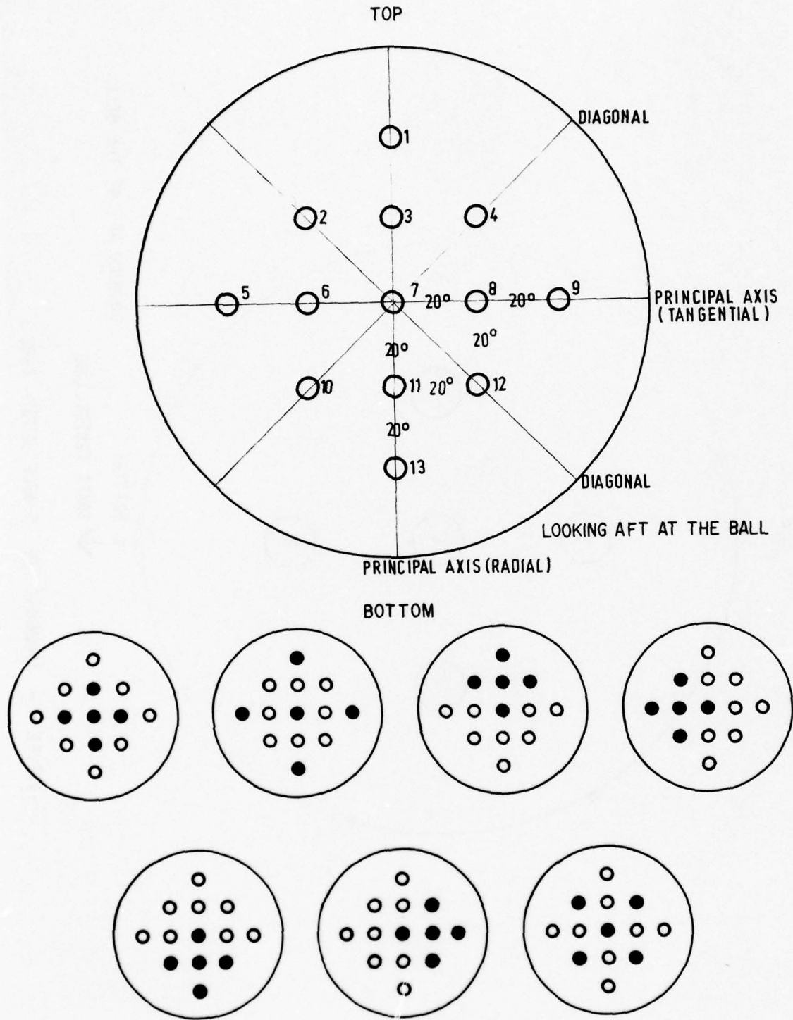
FIGURE 3 — SCHEMATIC OF 13-HOLE PITOT TUBE
