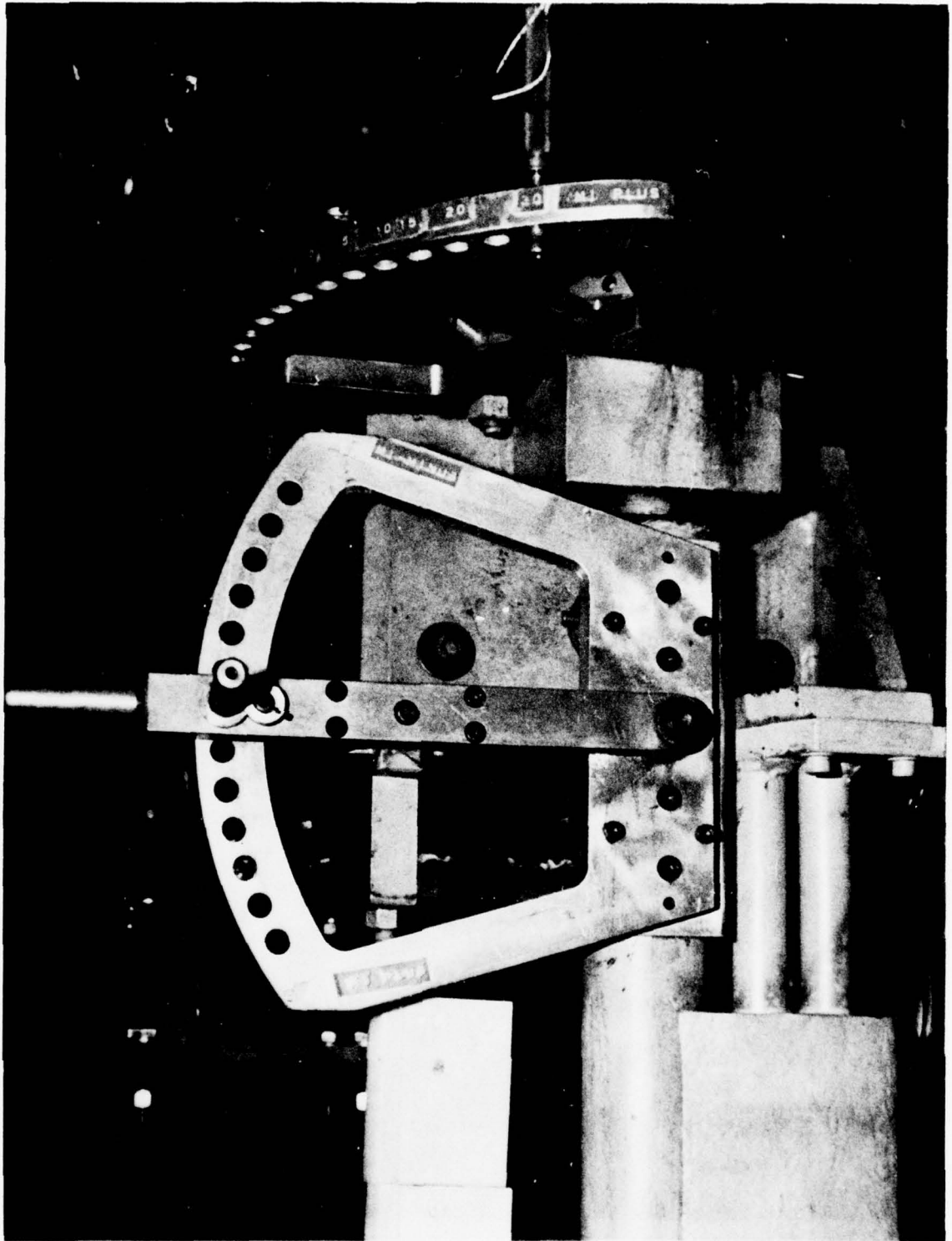
Figure 5 - Calibration Rake Showing Horizontal and Vertical Angular Quadrants
