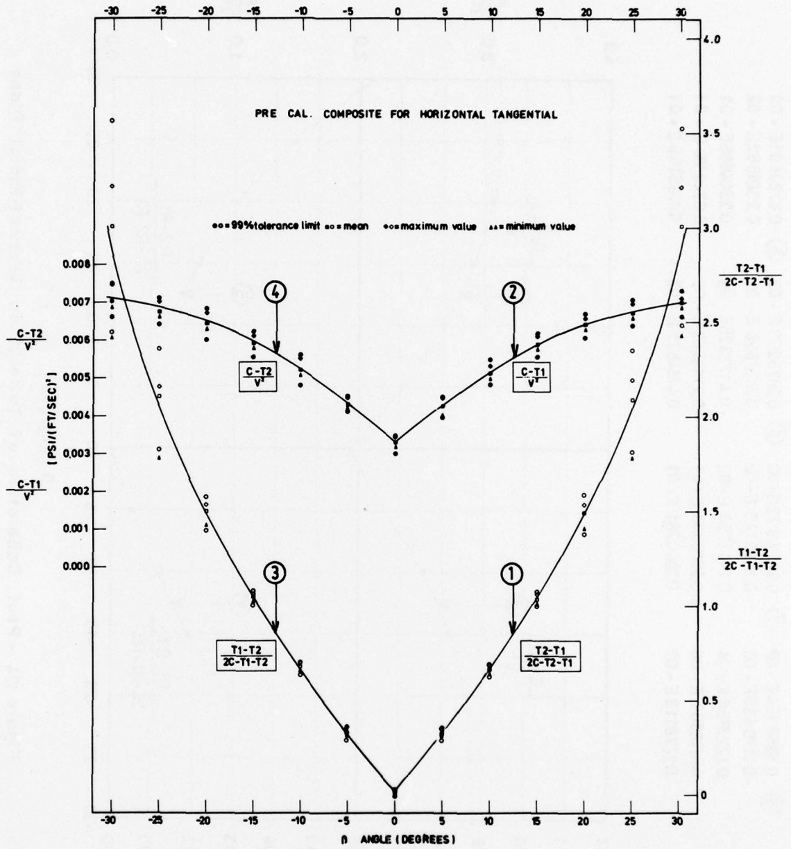
Figure 135 - Pre Calibration Composite for the Horizontal/ Tangential Plane
