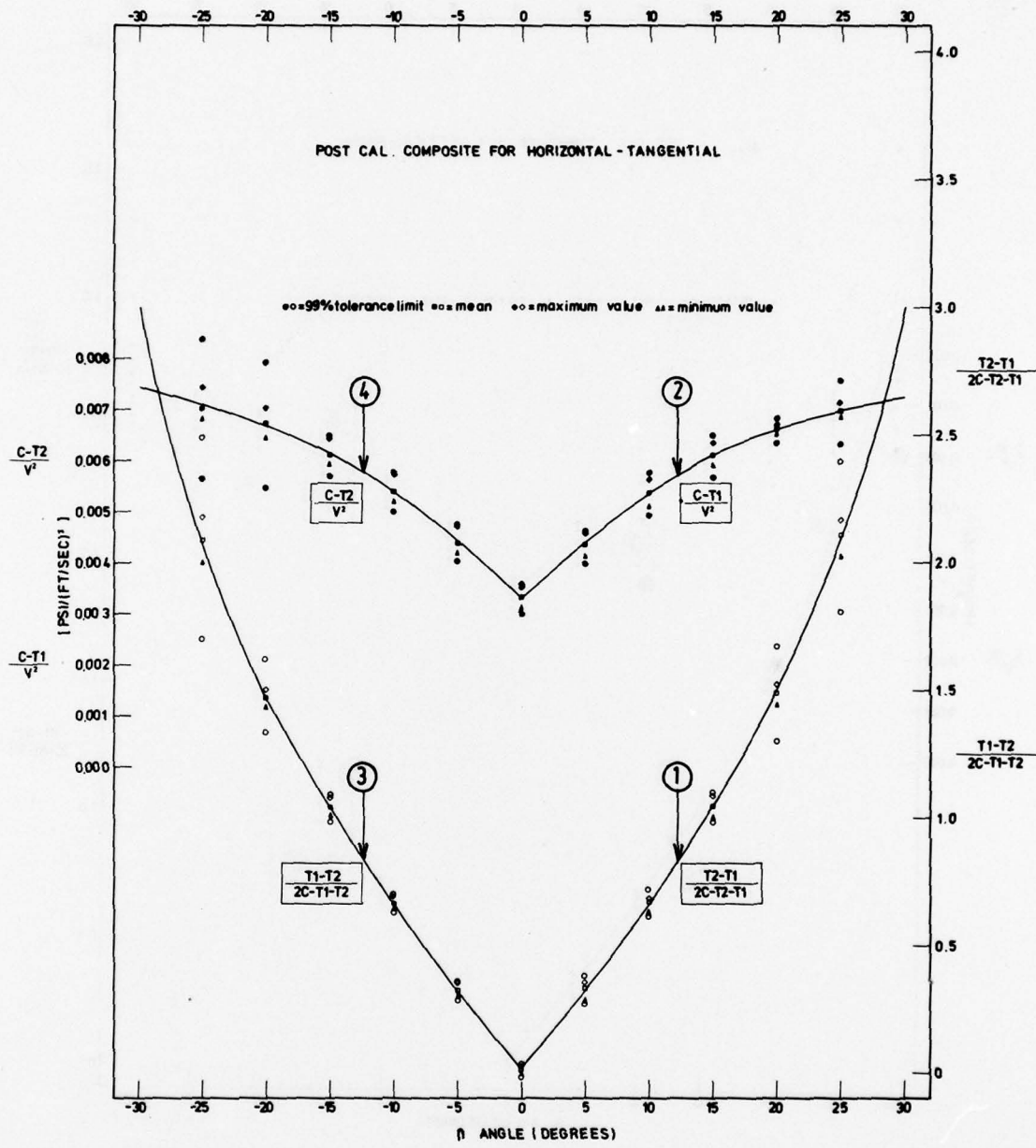
Figure 137- Post Calibration Composite for the Horizontal/Tangential Plane
