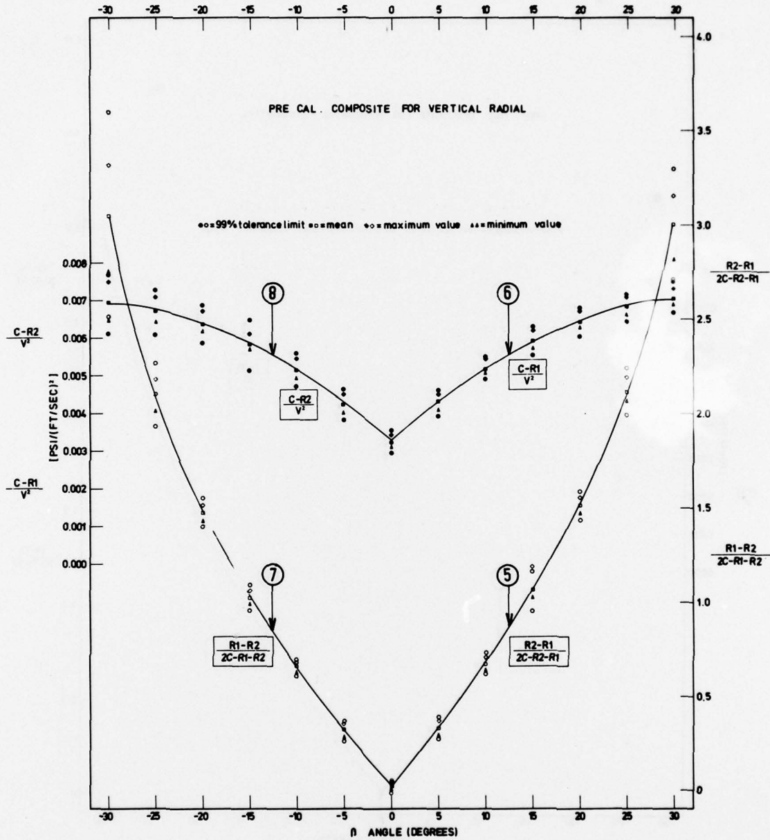
Figure 136-Pre Calibration Composite for the Vertical/Radial Plane
