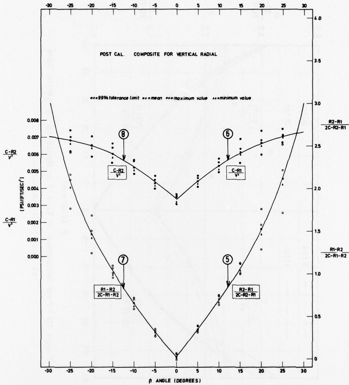
Figure 138 -Post Calibration Composite for the Vertical / Radial Plane
