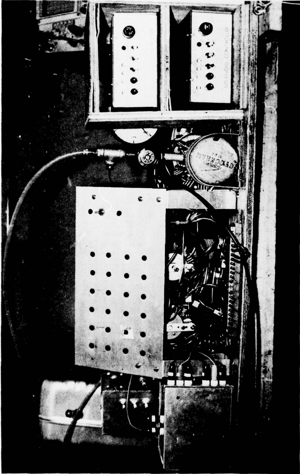
Figure 7 - Scanivalve Pressure Control and Measurement System
