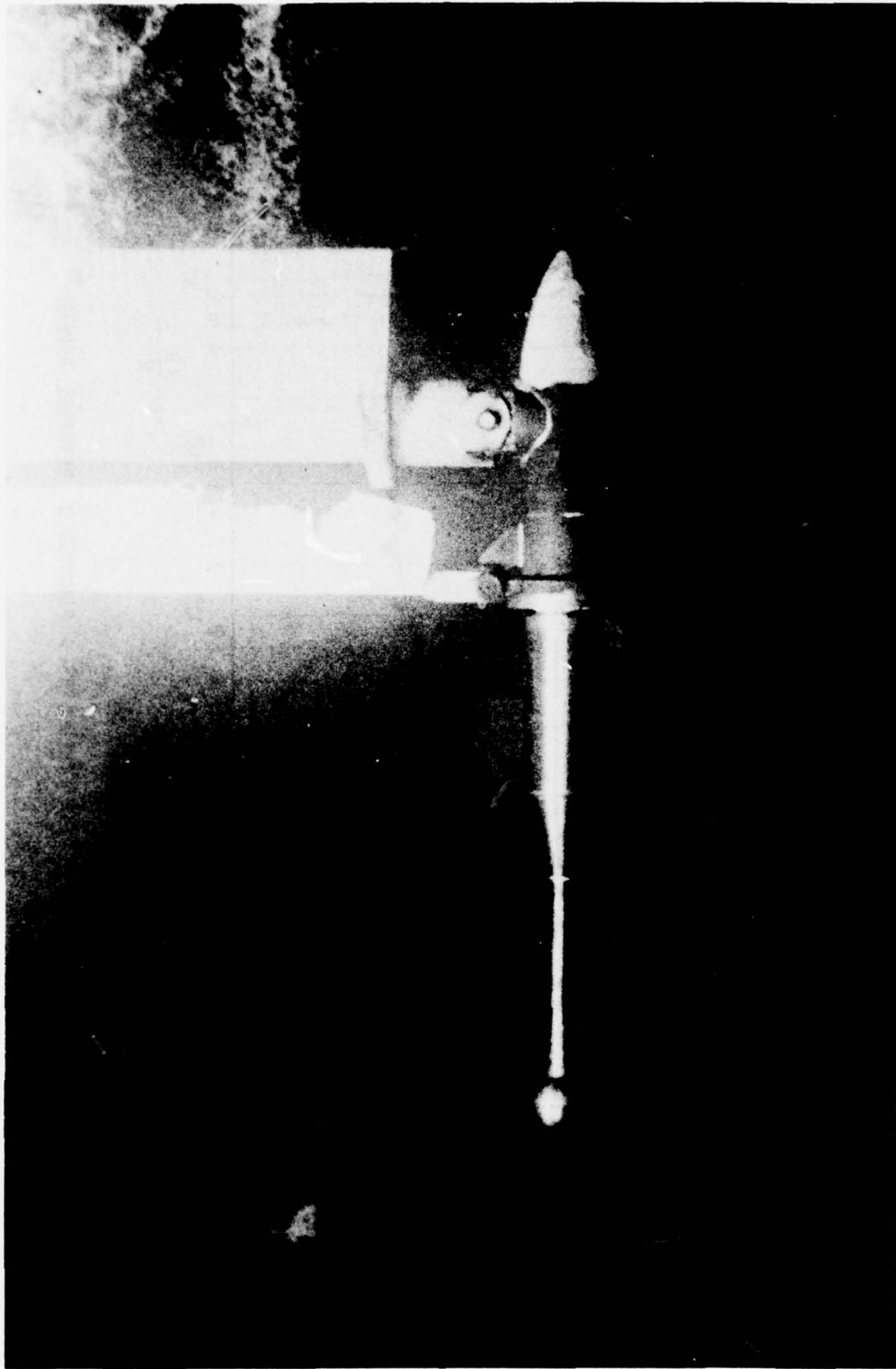
Figure 10 - Pitot Tube During Measuring Cycle
