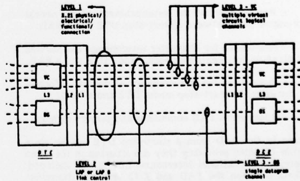
FIGURE 9 MODEL OF DTE/DCE INTERFACE SUPPORTING X.25 VIRTUAL CIRCUIT AND DATAGRAM OPERATION
