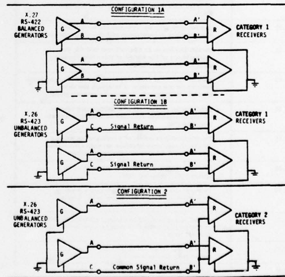
FIGURE 5 RECEIVER AND INTERCONNECTING CONFIGURATIONS
