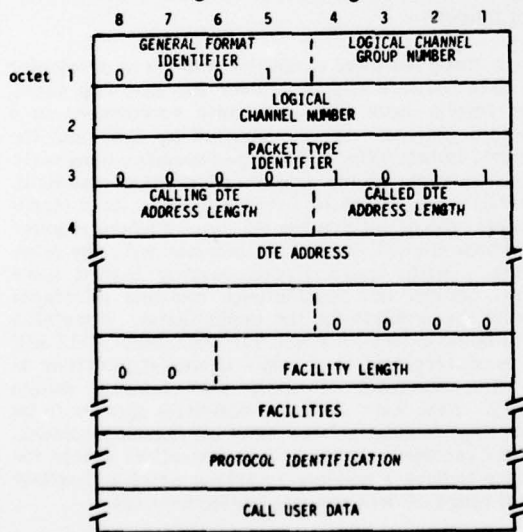
FIGURE 8 X.25 CALL REQUEST and INCOMING CALL Packet Format
