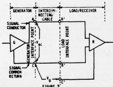
FIGURE 3 SYMBOLIC REPRESENTATION OF UNBALANCED CIRCUIT
