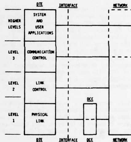
FIGURE 2 ARCHITECTURE OF INTERFACE LEVELS
