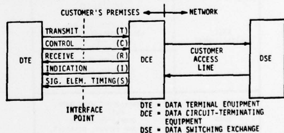
FIGURE 7 X.21 INTERFACE
