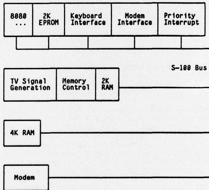
Figure 2.1. Block Diagram Of The Terminal.
