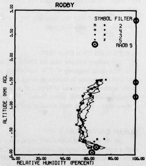
Fig. 6-3 (cont). Relative Humidity Versus Altitude for Twelve Project OPAQUE III Flights.
