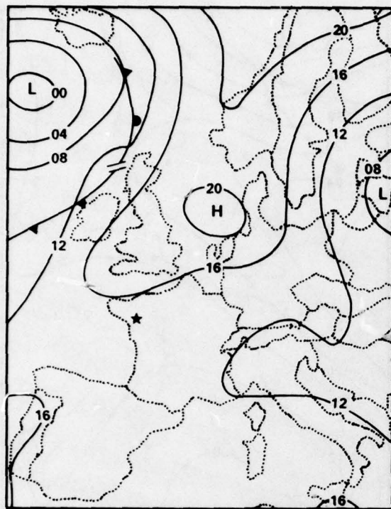
4 JULY 1977 0000 GMT
