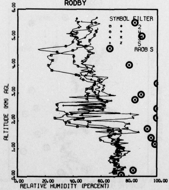
Fig. 6-3. Relative Humidity Versus Altitude for Twelve Project OPAQUE III Flights.
