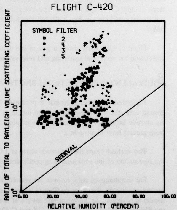
Fig. 8-11. Ratio of Total to Rayleigh Total Volume Scattering Coefficient as a Function of Relative Humidity for Flights C-411, C-412, C-415 and C-420.
