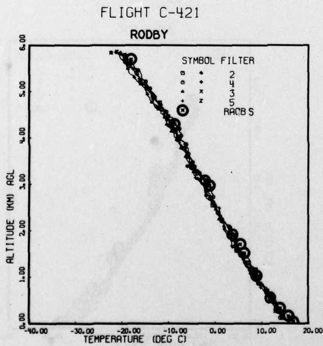
Fig. 6-2 (cont). Temperature Versus Altitude for Twelve Project OPAQUE III Flights.
