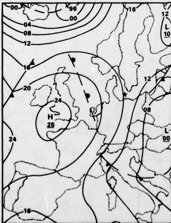
1 AUGUST 1977 1200 GMT
