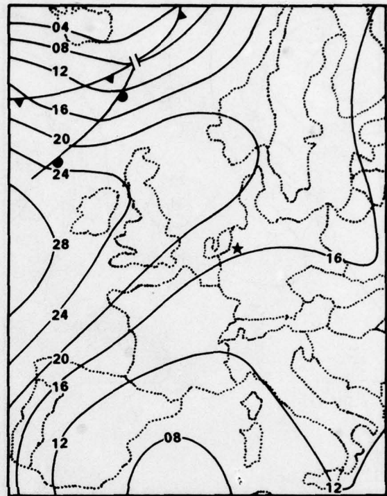
29 JULY 1977 1200 GMT
