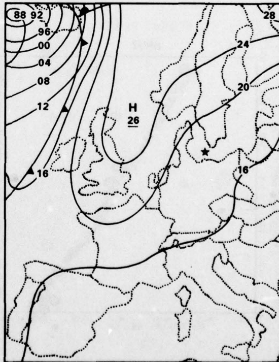
11 AUGUST 1977 1200 GMT
