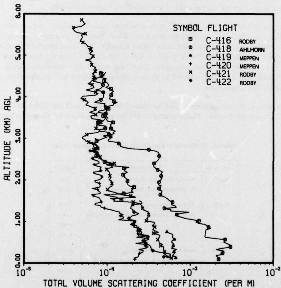
Fig. 8-6. Total Volume Scattering Coefficient for Filter 4 Pseudo-Photopic for six OPAQUE III Flights I through 11 August 1977.
