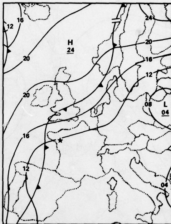
6 JULY 1977 1200 GMT
