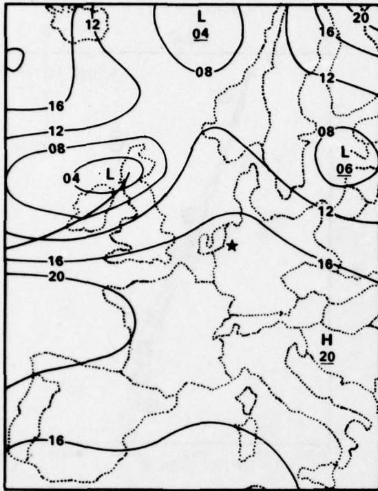
4 AUGUST 1977 1200 GMT
