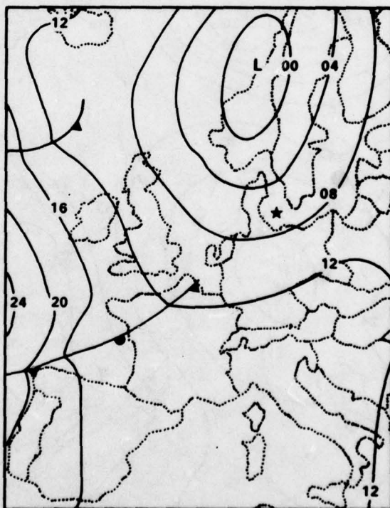
27 JULY 1977 1200 GMT
