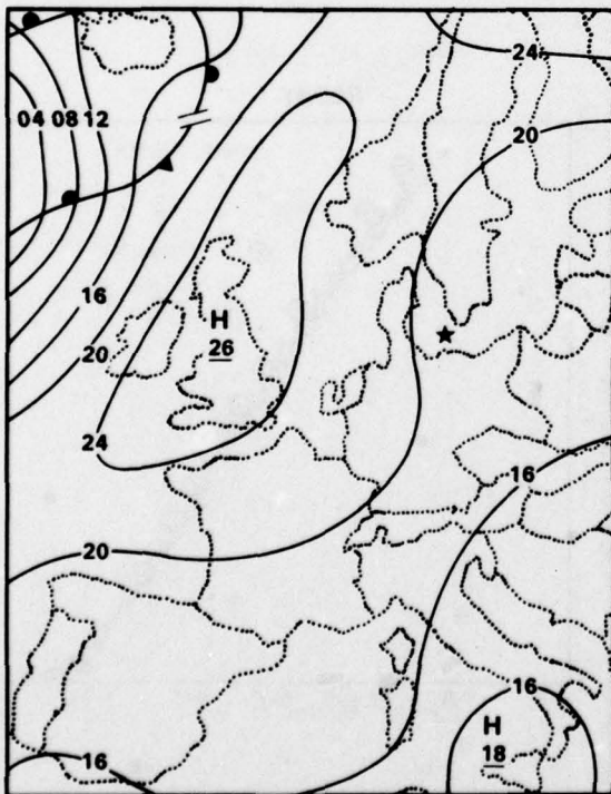
10 AUGUST 1977 1200 GMT
