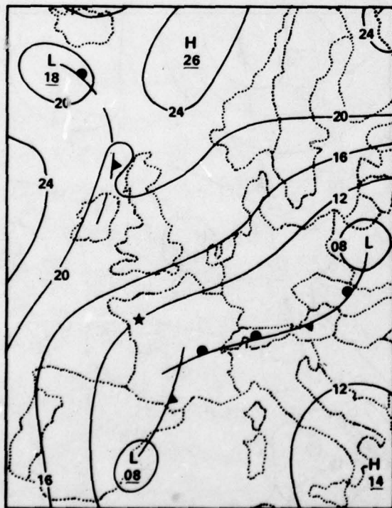
7 JULY 1977 1200 GMT
