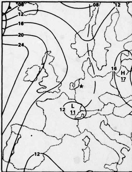
28 JULY 1977 1200 GMT
