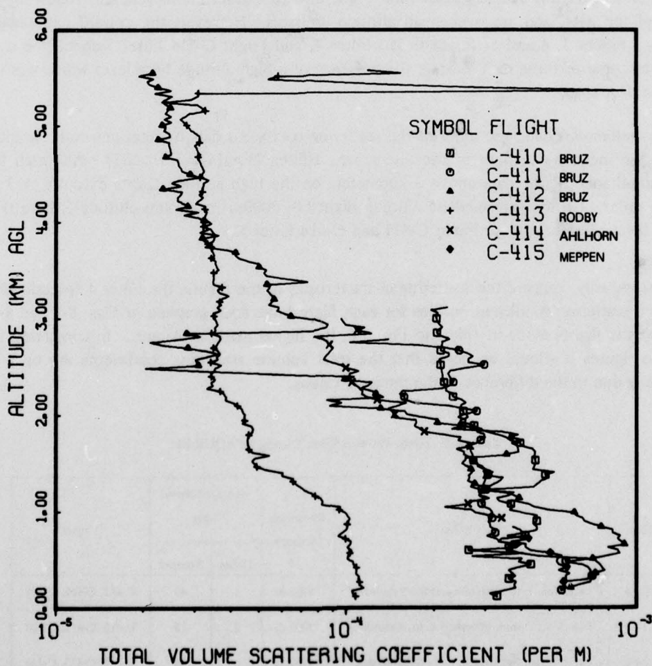
Fig. 8-5. Total Volume Scattering Coefficient for Filter 4 Pseudo-Photopic for six OPAQUE III Flights 4 through 29 July 1977.
