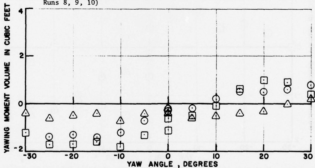
Figure 17. Variation of yawing moment volume with yaw angle for various angles of attack for the ACES II ejection seat with anthropometric dummy. (Configuration F, Runs 8, 9, 10)
