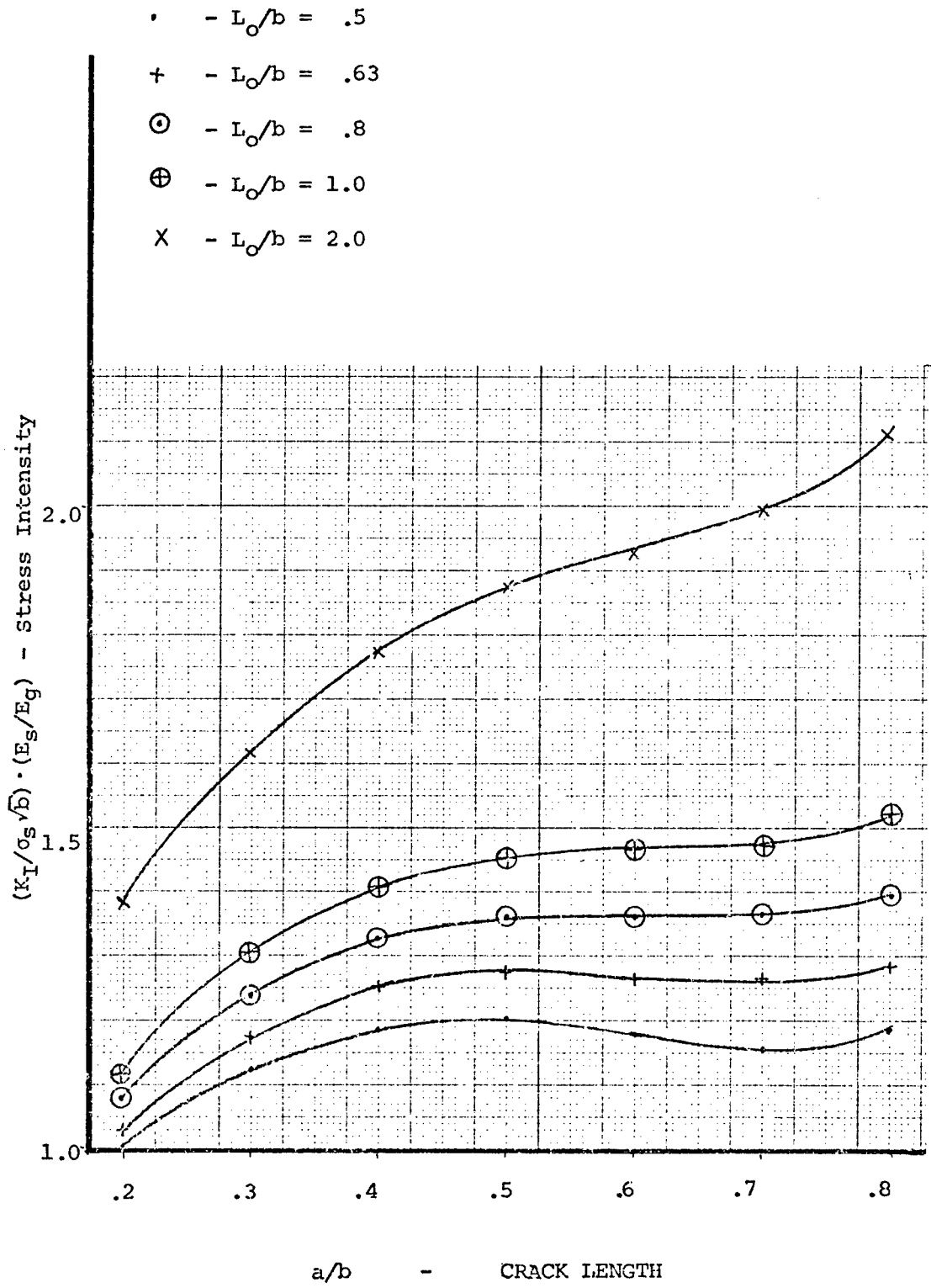
Figure 18. Stress Intensity Factor Results for Gages with t_c/t_o = .75 , L_c/b = .625
