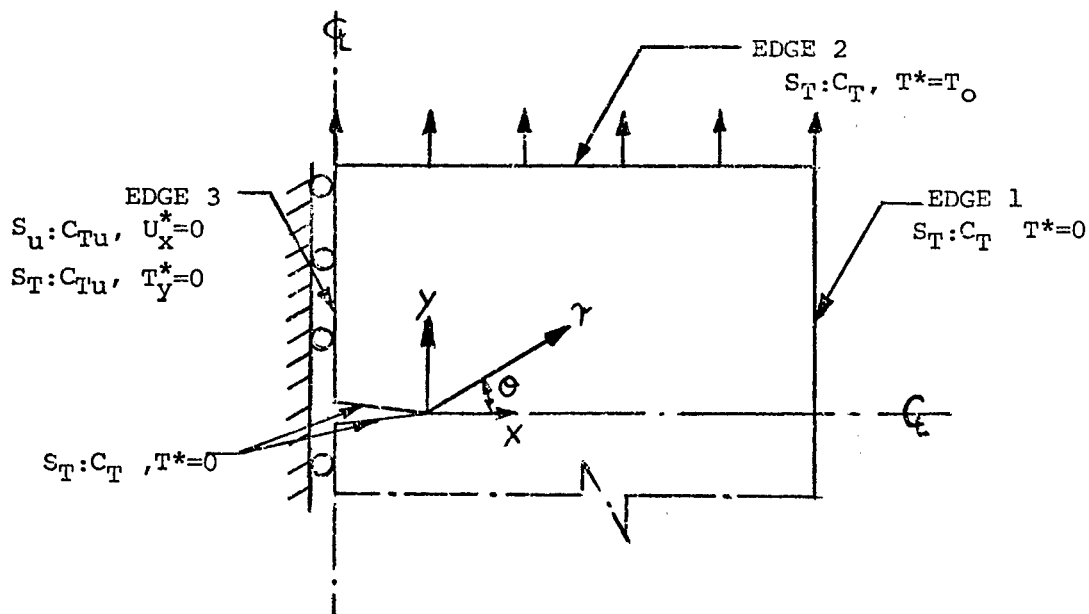
(b) Type 2, Mixed Boundary Conditions - Prescribed stresses and displacements on same region
