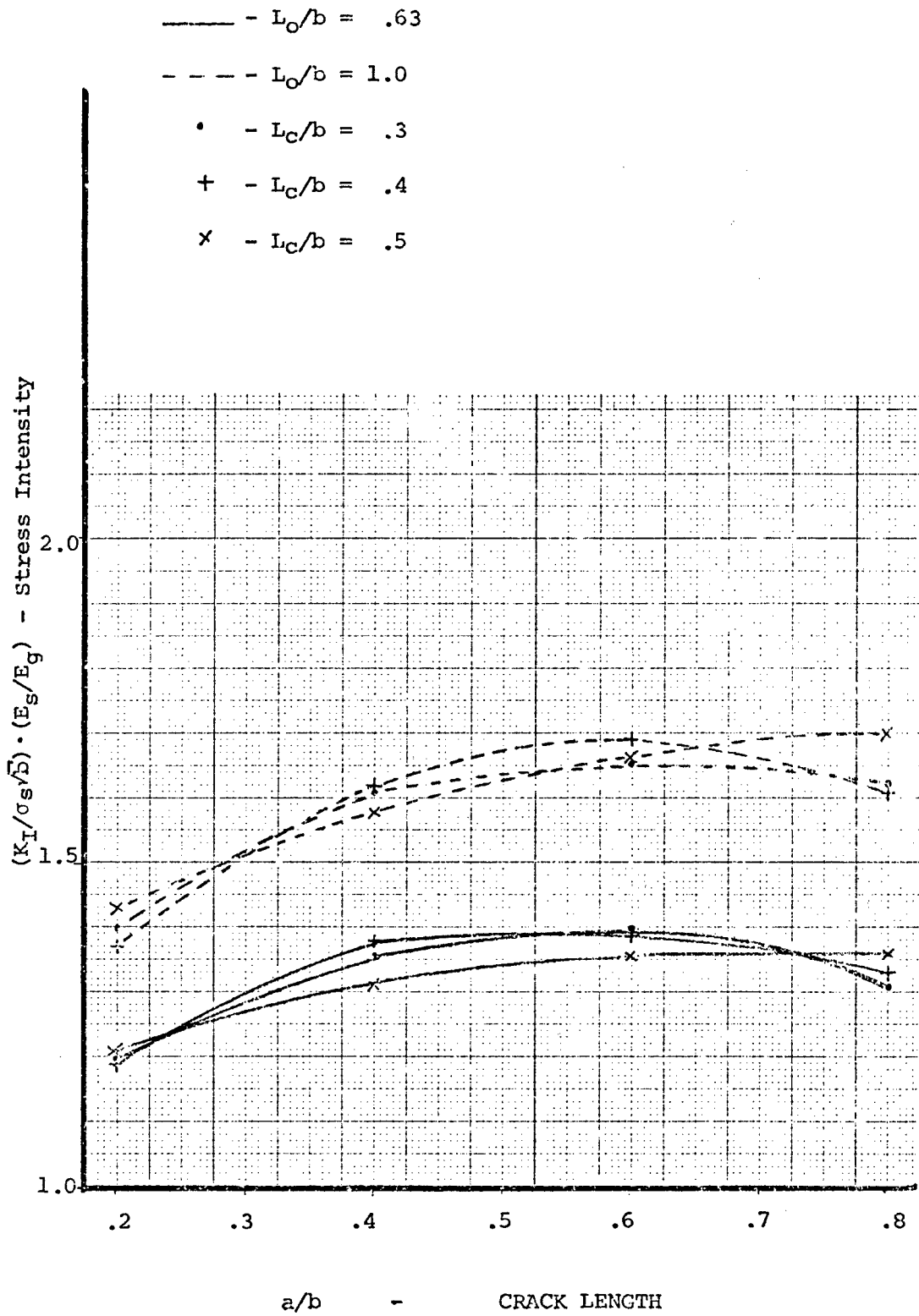
Figure 14. Stress Intensity Factor Results for Gages with t_c/t_0 = .5 , Various Length Ratio
