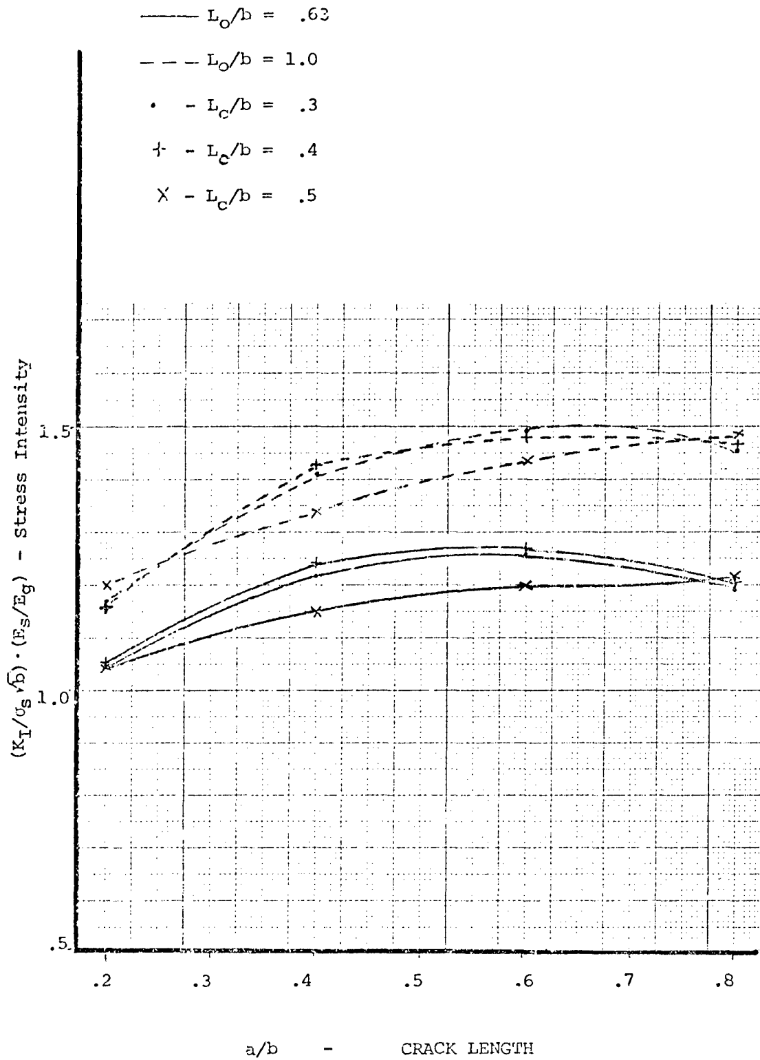
Figure 17. Stress Intensity Factor Results for Gages with t_c/t_0 = .75 , Various Length Ratios
