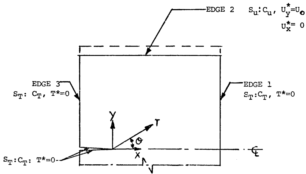
(a) Type 1, Mixed Boundary Conditions - No mix between prescribed traction and displacement on same region
