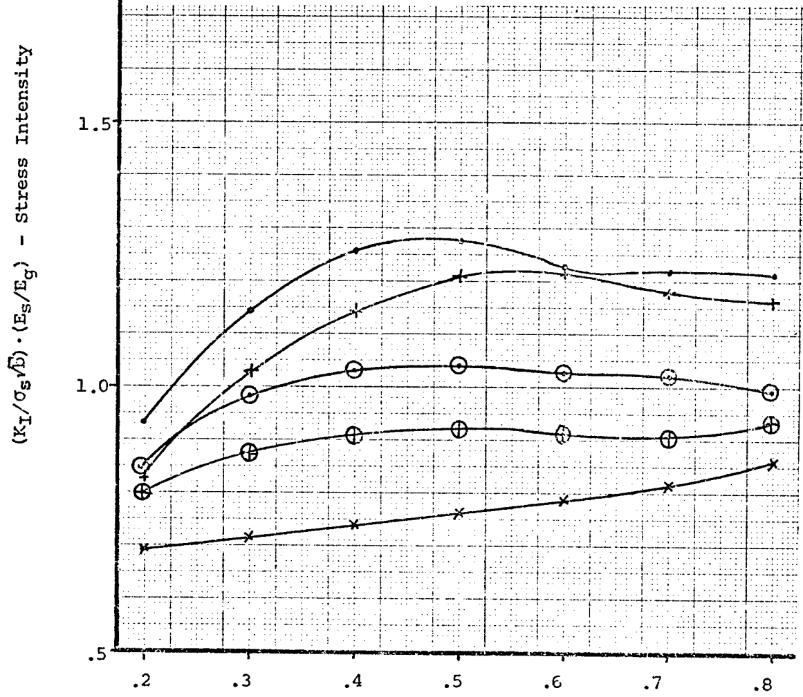
Figure 5. Stress Intensity Factor for Trapezoid Crack Gage H_a/b = 1 .
