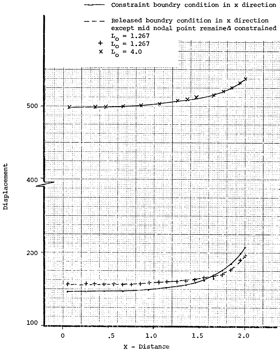
Figure 24. Displacements of Membrane Edge Due to Uniform Stress
