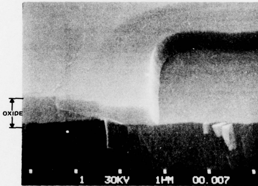
Figure 3. Cross Section of E-Beam Slice from Lot 110 at Emitter O.R. Oxide was not Stripped
