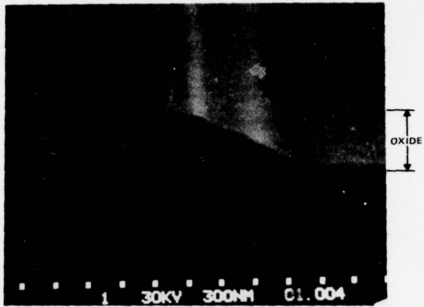
Figure 2. Cross Section of E-Beam Slice at Emitter O.R. with Oxide Stripped – Lot 107
