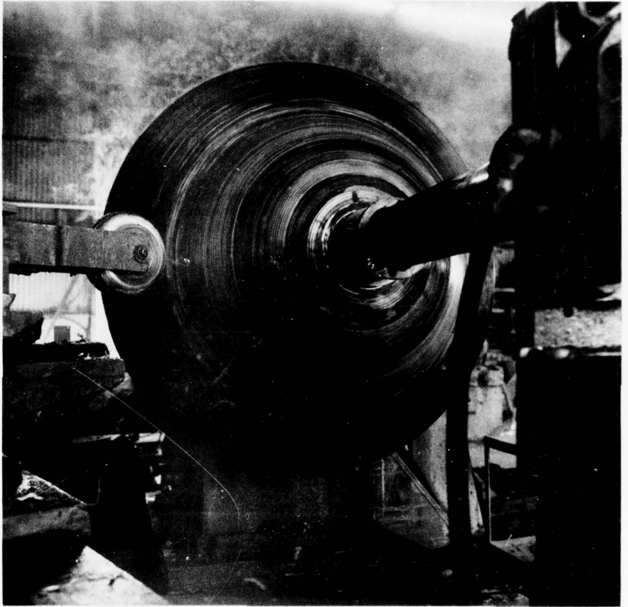
Figure 3-6. Spin Forming 60-Inch Diameter Plate
