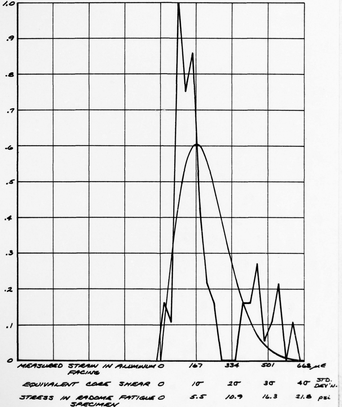
FIGURE 8 MEASURED STRAIN PEAK DISTRIBUTION HISTOGRAM, ALUMINUM SKIN FOAM CORE PANEL, SUBJECTED TO 30mm FIRING BLAST
