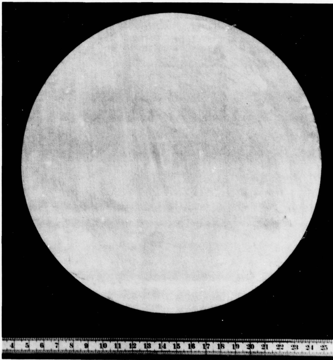
Figure 3-30. Template for Cutting Glass Cloth for Hemispherical Search Radome
