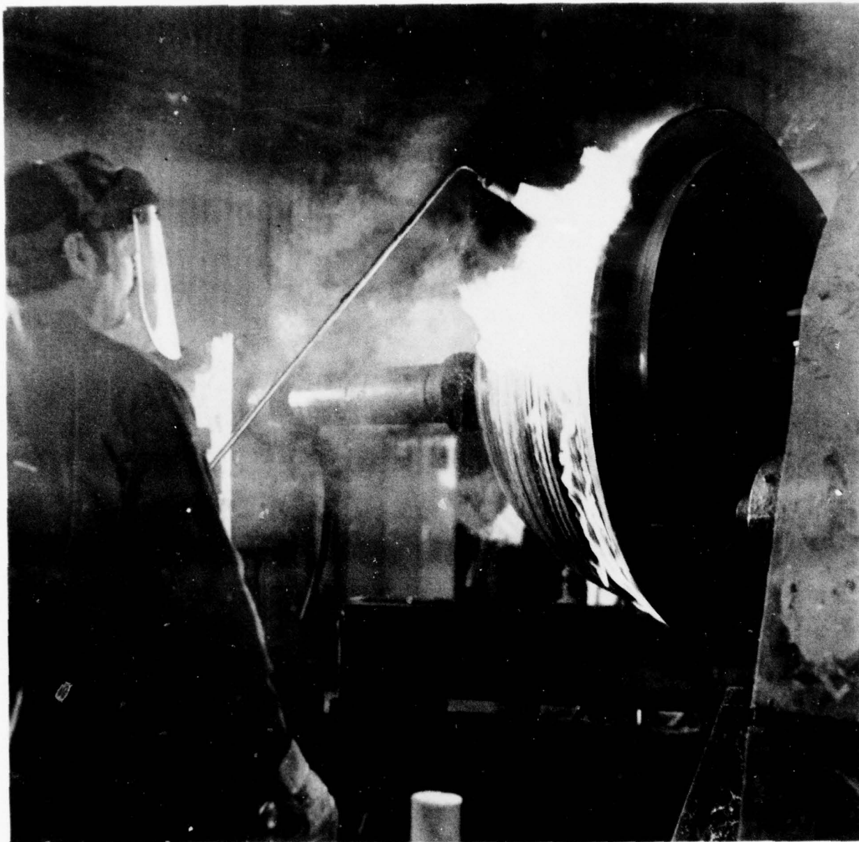
Figure 3-5. Spin Forming 60-Inch Diameter Aluminum Plate
