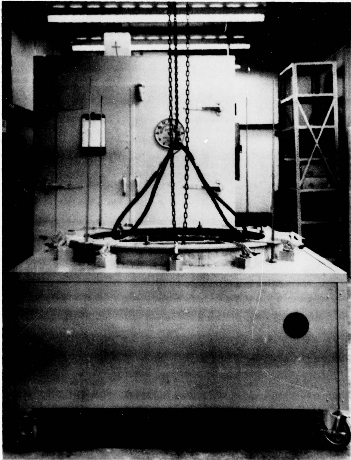
Figure 3-31. Naval Radome Mold Assembly After Oven Temperature Cure
