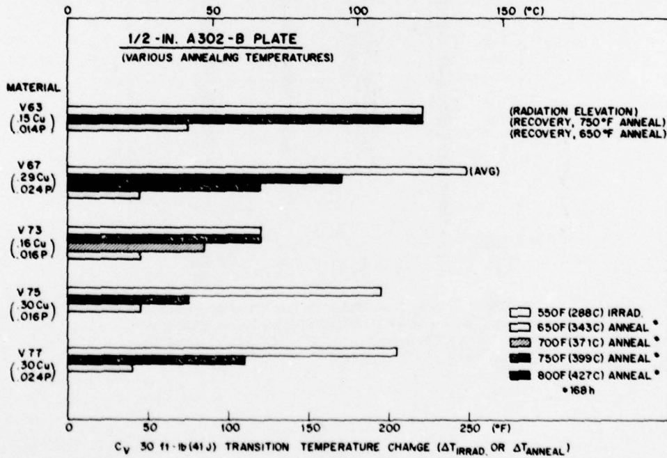
Fig. 12 — Comparison of Charpy-V transition-temperature recovery (41-J index) produced by various postirradiation heat-treatment temperatures. The initial radiation-induced elevations in transition temperature are also shown for reference.
