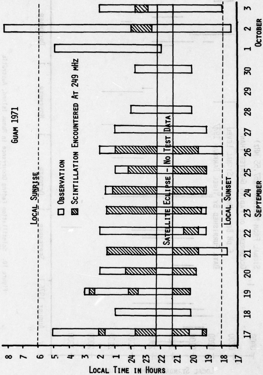
Figure 9. Duration of Scintillation Fading Occurrence in Guam (From Johnson Reference 12)
