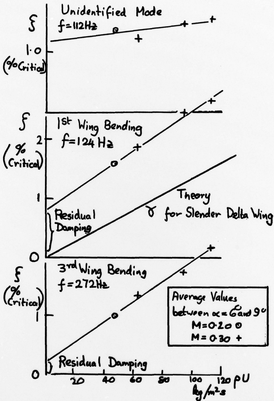
Fig 9 Variation of damping with (density \times velocity)
