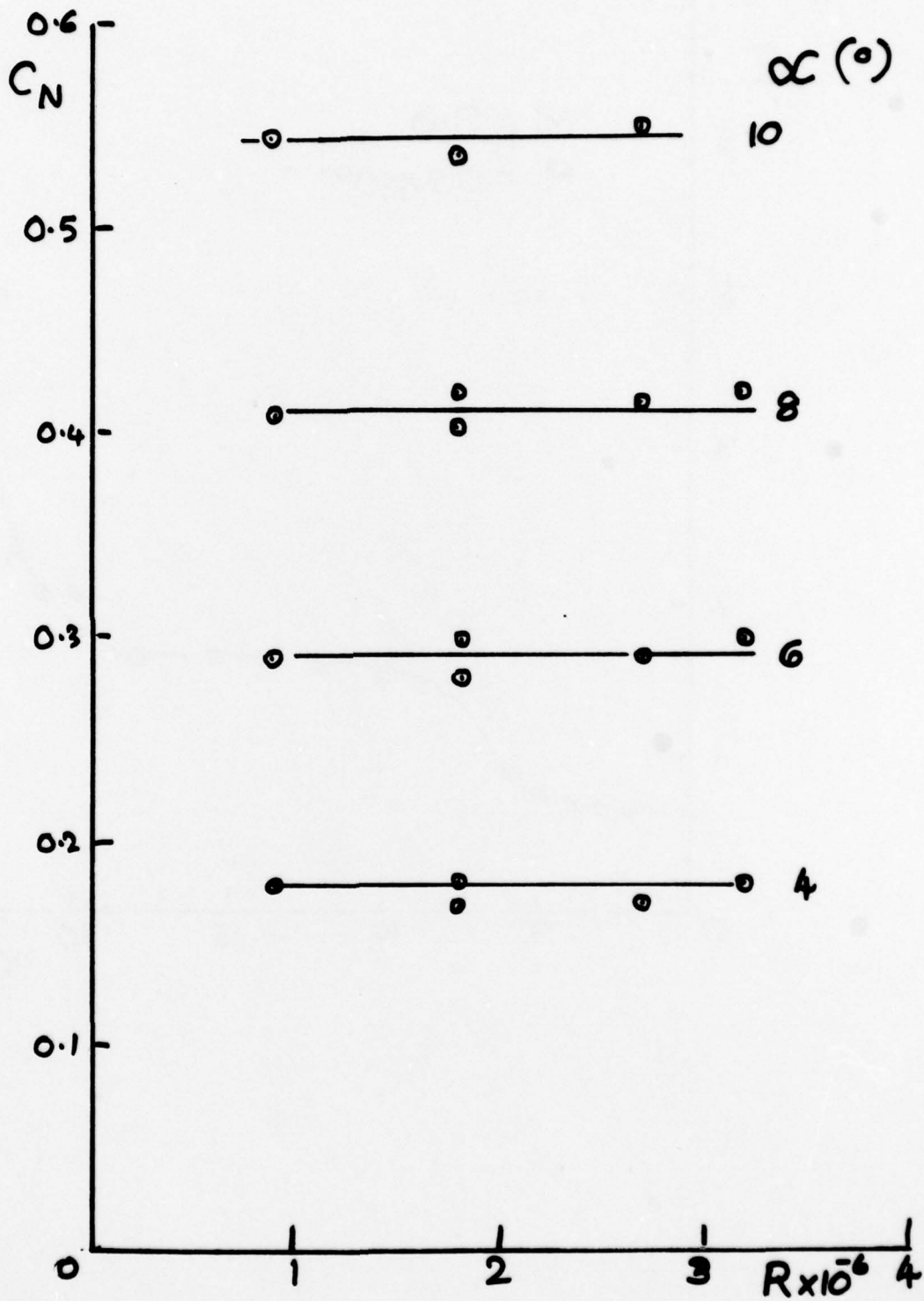
Fig 5 Variation of normal force coefficient with incidence and Reynolds number M = 0.30
