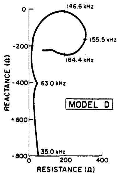
Fig. 6 - Typical Impedances
