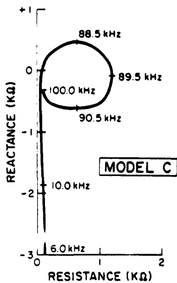
Fig. 6 - Typical Impedances
