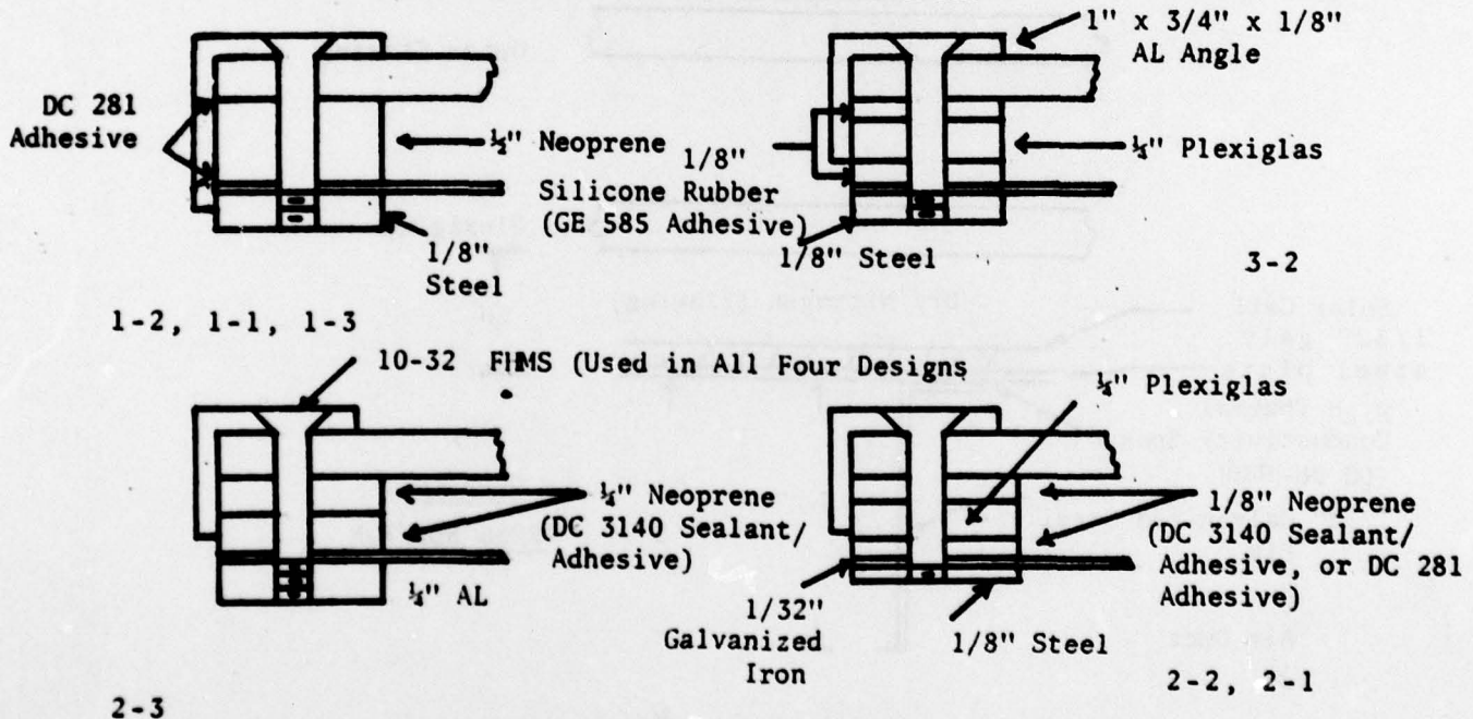
DETAIL OF CROSS SECTION A-A FOR VARIOUS SUBPANELS
