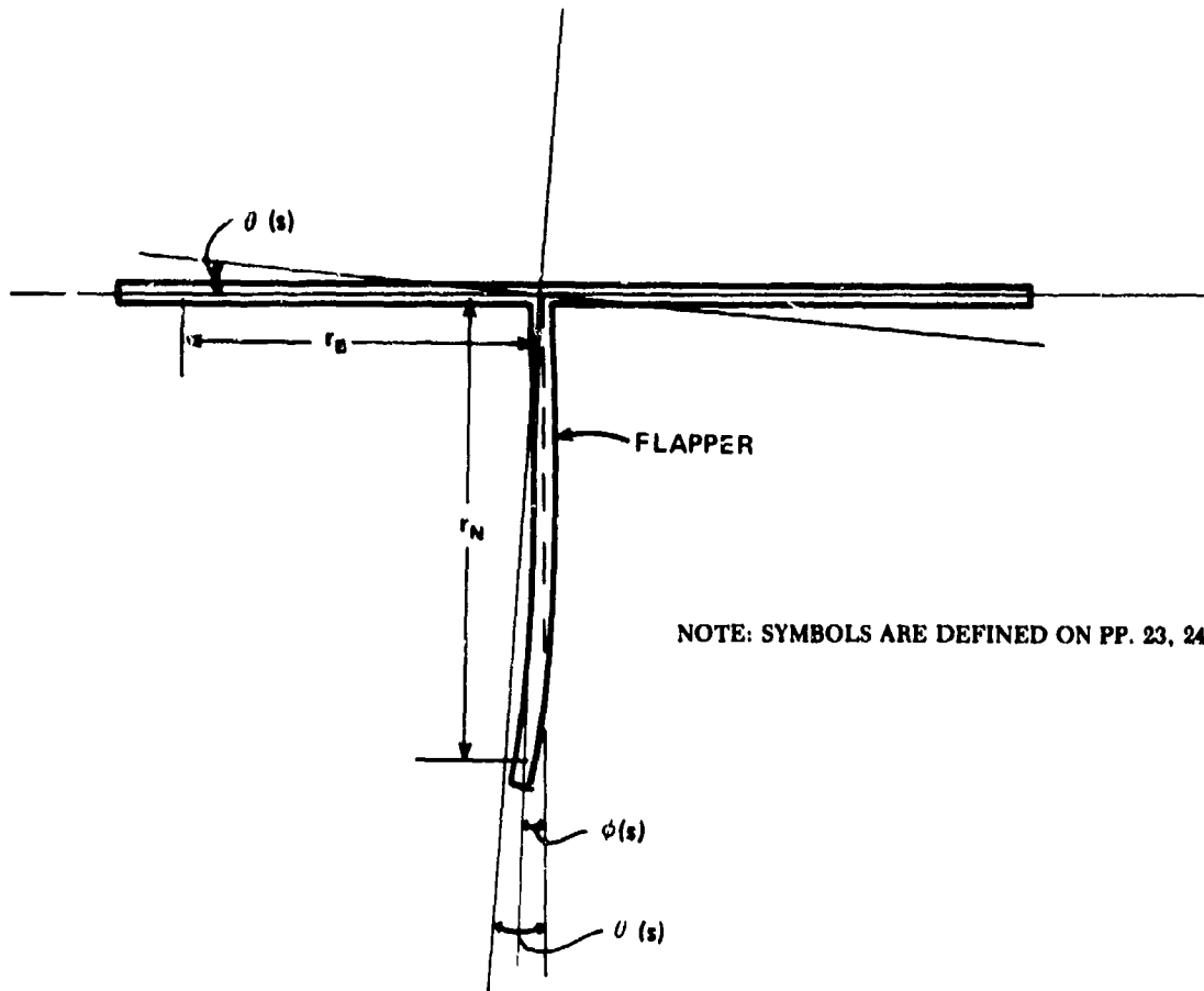
Figure 5. Flapper deflection and bending angle.
