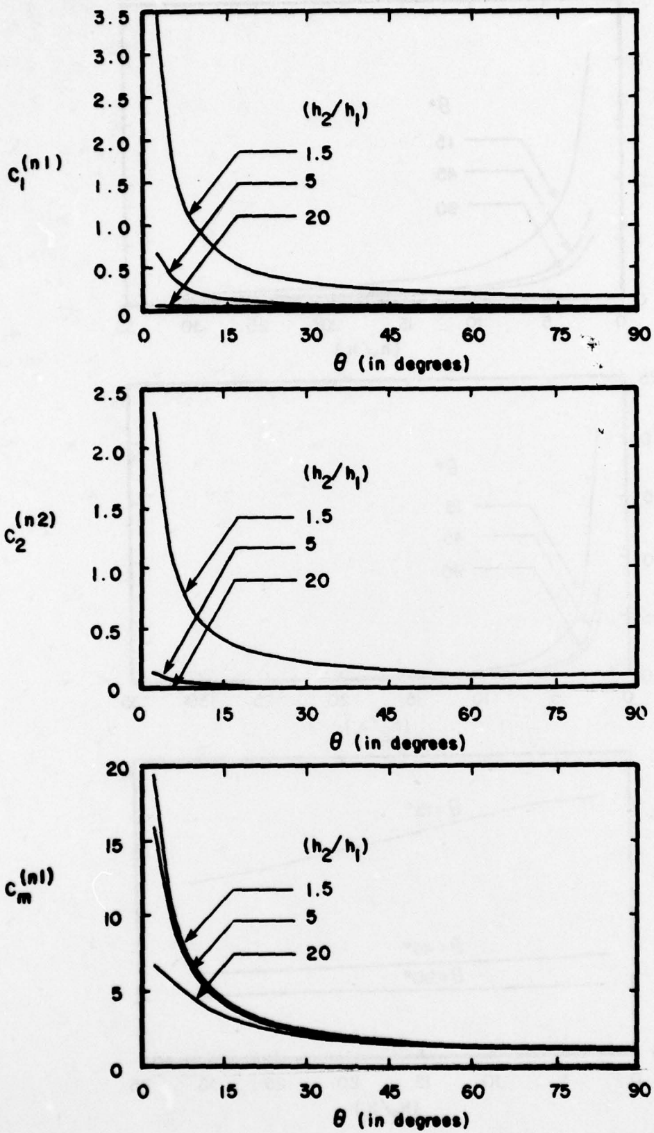
Figure 3.5. Normalized lumped capacitances as a function of skew angle
