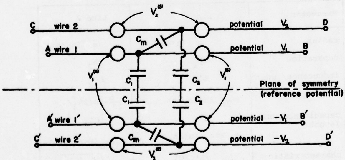
Figure 1.5b. Symmetrical form of the above circuit.
