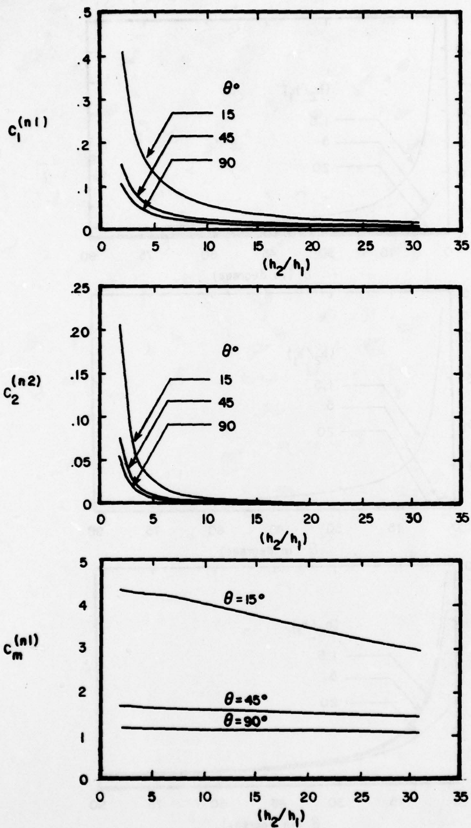
Figure 3.6. Normalized lumped capacitances as a function of relative height
