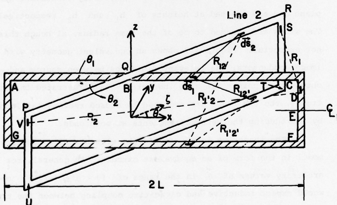
Figure 1.2. Equivalent pair of skewed two-wire transmission lines of length 2L .
