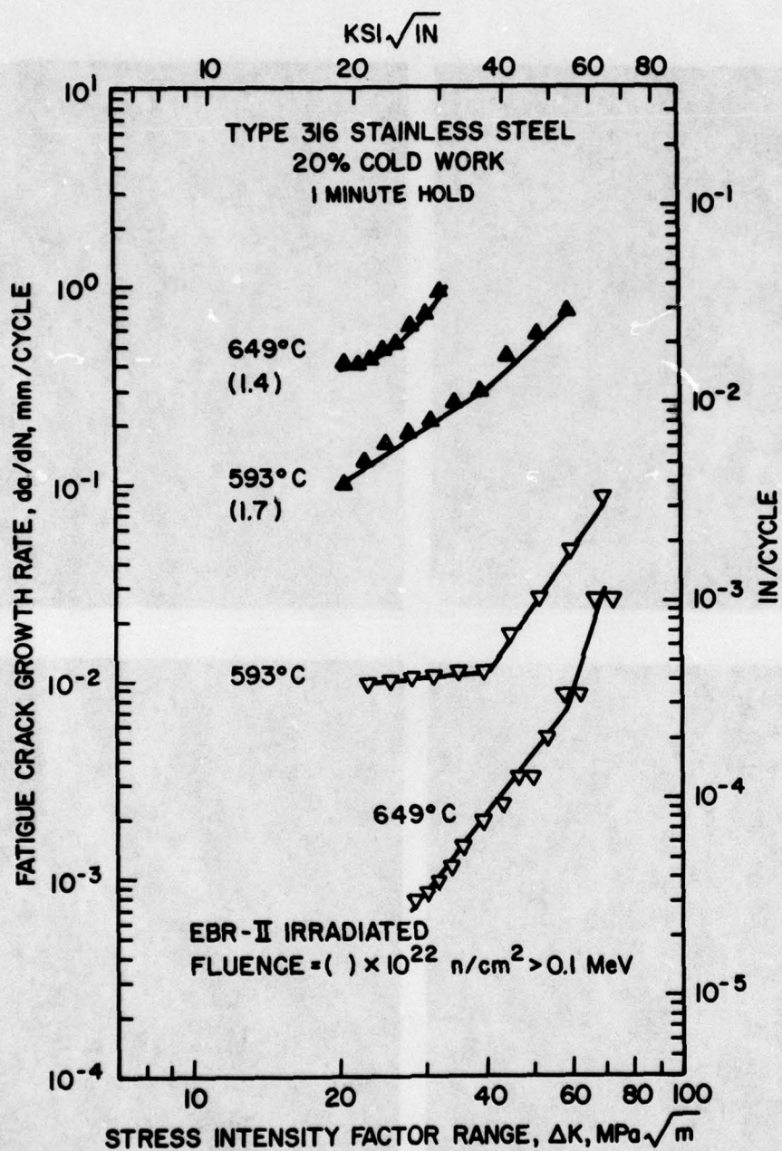
Fig. 4. Comparison of fatigue crack propagation rates, da/dN , in air at 593 and 649°C for 20 percent cold worked, EBR-II irradiated and unirradiated Type 316 stainless steel tested with one minute hold time.
