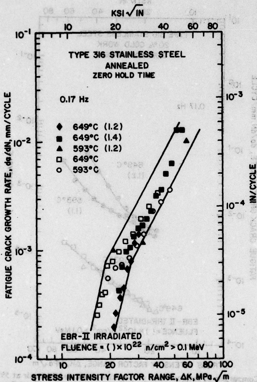
Fig. 1. Comparison of fatigue crack rates, da/dN , in air at 593 and 649°C for solution annealed, EBR-II irradiated and unirradiated Type 316 stainless steel tested for continuous cyclic loading at 0.17 Hz (10 cpm).
