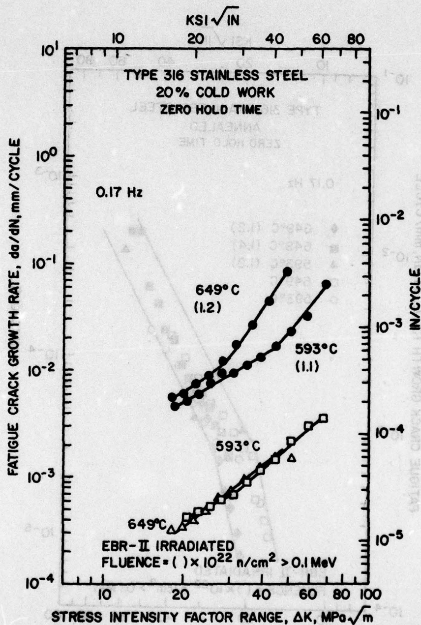
Fig. 2. Comparison of fatigue crack propagation rates, da/dN , in air at 593 and 649°C for 20 percent cold worked, EBR-II irradiated and unirradiated Type 316 stainless steel tested with continuous cyclic loading at 0.17 Hz (10 cpm).
