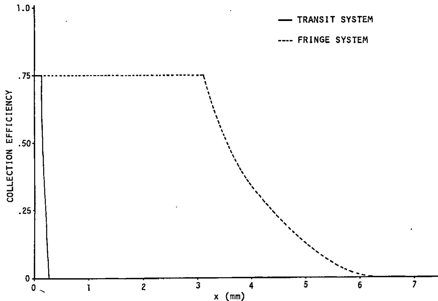
FIGURE 4. AXIAL COLLECTION EFFICIENCY OUTWARD FROM RECEIVER (FROM FIELD STOP IMAGE).
