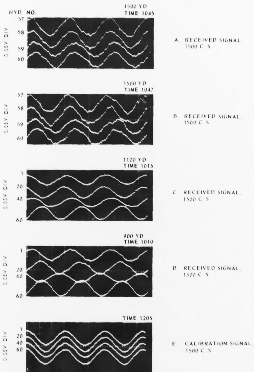
Figure 9. Simultaneous trace photographs comparing signal phases in four hydrophone channels at a time. No filters used. 200 \mu sec/div. Relative bearing 000 ^{\circ} except in 9D, 350.5 ^{\circ} .
