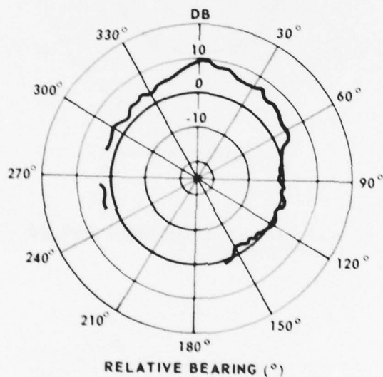
Figure 1. Relative responses of starboard bow and port bow reference hydrophones to noise pings from the REXBURG to the BAYA through 360° relative bearing. Transmitted noise bandwidth 100 c/s, centered at 1500 c/s. In each figure the constant radius circle represents zero response difference between the bow reference hydrophone and the array hydrophone. Curves outside the circle indicate that the bow hydrophone response is higher than that of the array hydrophone; those inside, that it is lower.
