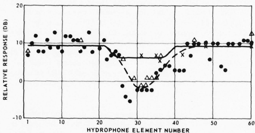
Figure 4. Responses of array elements and bow reference hydrophones to direct-path horizontal pings arriving from 000^{\circ} relative bearing, showing improvement with hydrophones mounted near Frame 3, 2 feet above deck.
