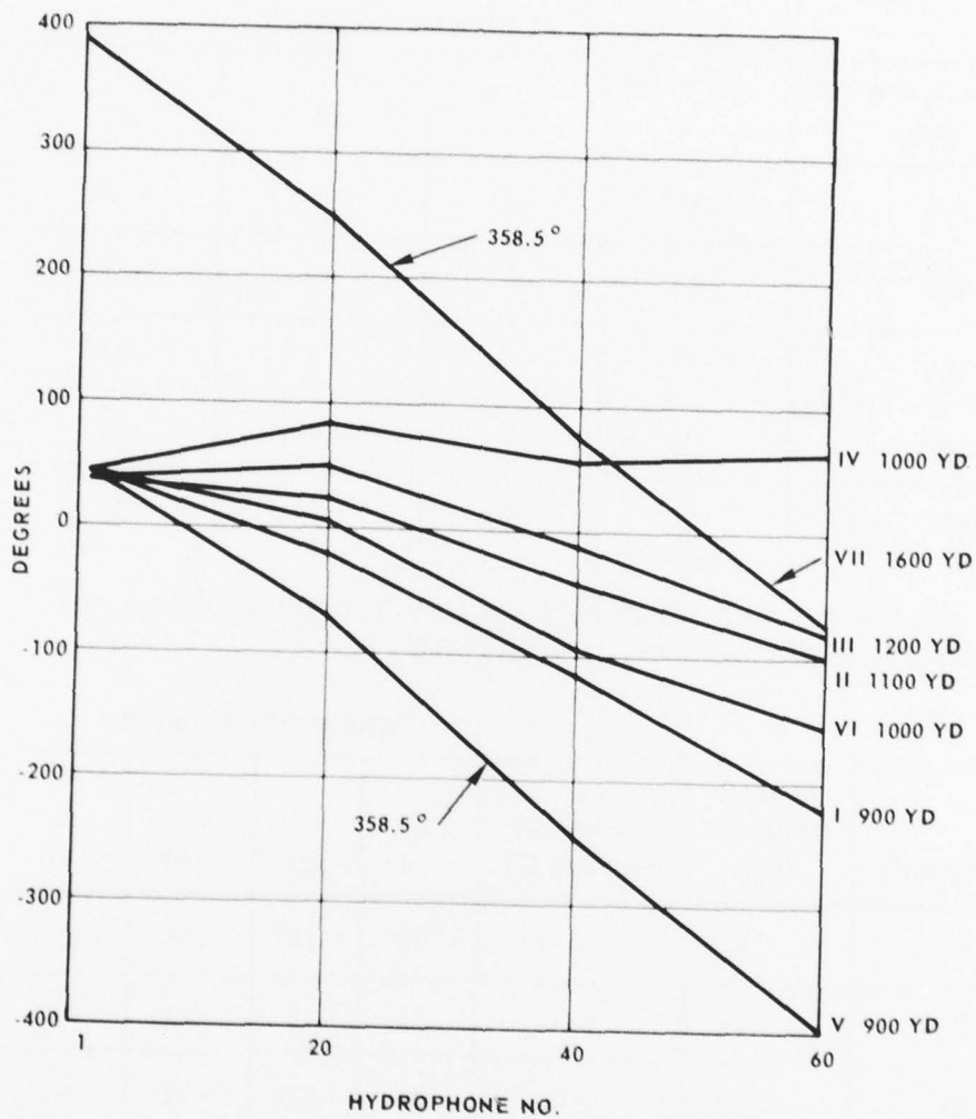
Figure 11. Measured hydrophone phase differences corrected for curved wavefront. Periscope bearing of source assumed to be 000^{\circ} except where indicated to be 358.5^{\circ}
