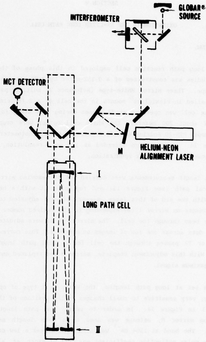
Figure 14. Optical Path Used in Conjunction with the Long Path Cell
