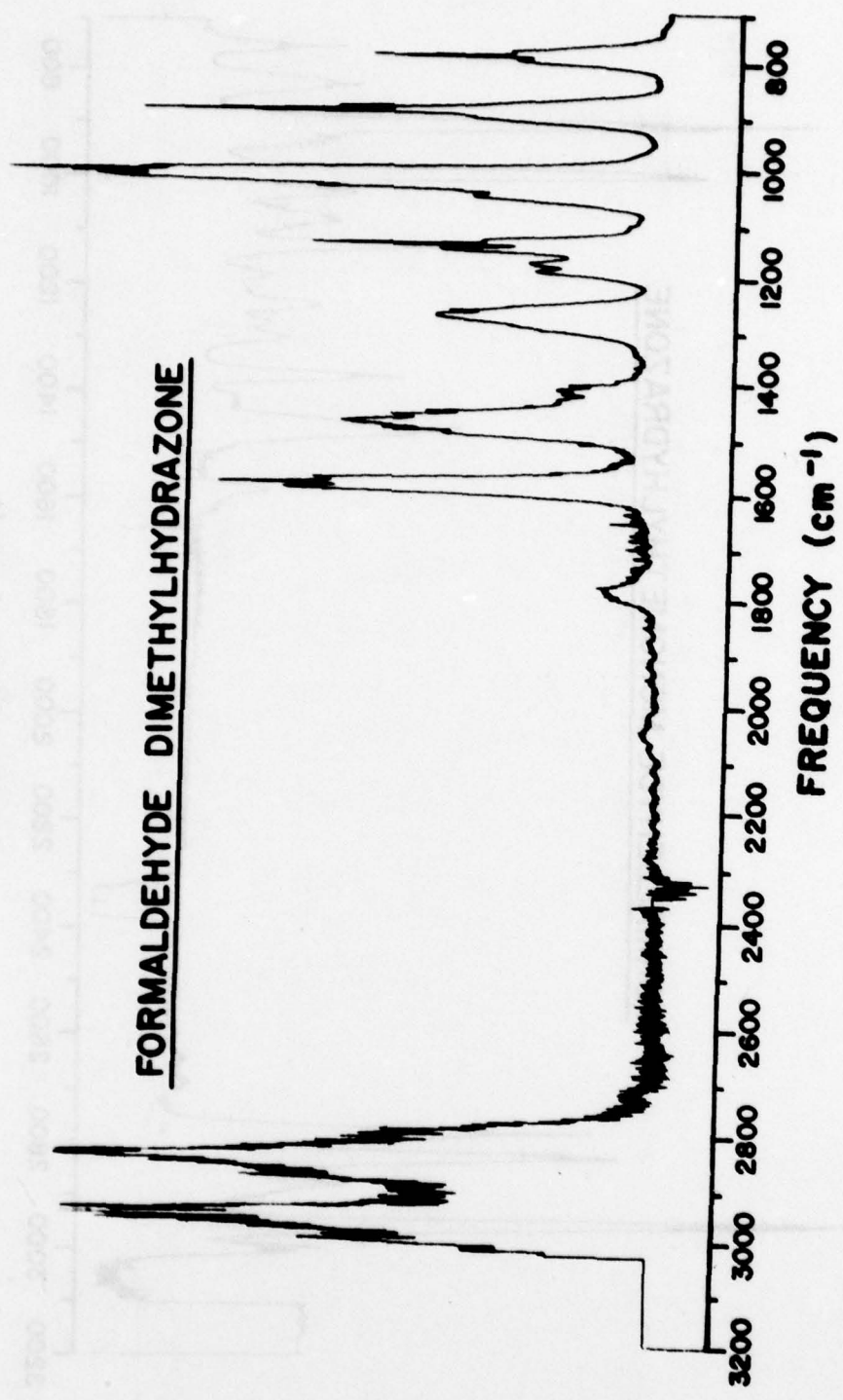
Figure 18. Infrared Spectrum (1.0-cm -1 Resolution) of Formaldehyde Dimethylhydrazone
