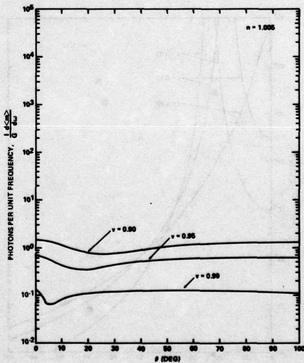
Figure 15. Mean number of photons per unit frequency versus \theta .
