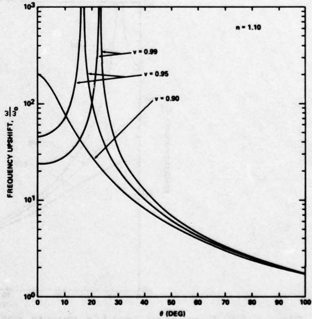
Figure 7. Frequency upshift versus \cos \theta ; two Cerenkov branches appear at v = 0.95 and 0.99 .
