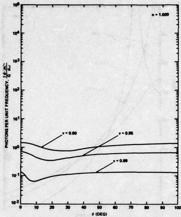
Figure 14. Mean number of photons per unit frequency versus \theta ; curves are smooth for all \theta .
