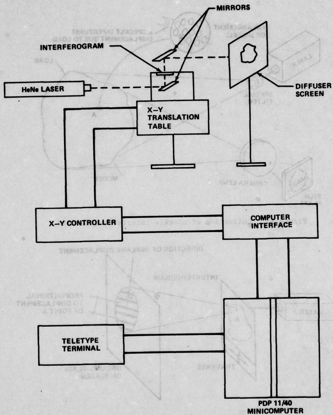
Figure 13. Electromechanical single-beam speckle interferometric analyzer system.
