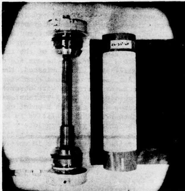
Figure 10. Loading fixture.
