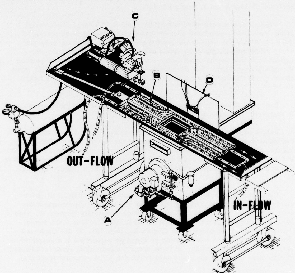
FIGURE 1. USAARL T-1 Furnace (A) and Pneumatically Operated Water-Cooled Shutter System (B).
