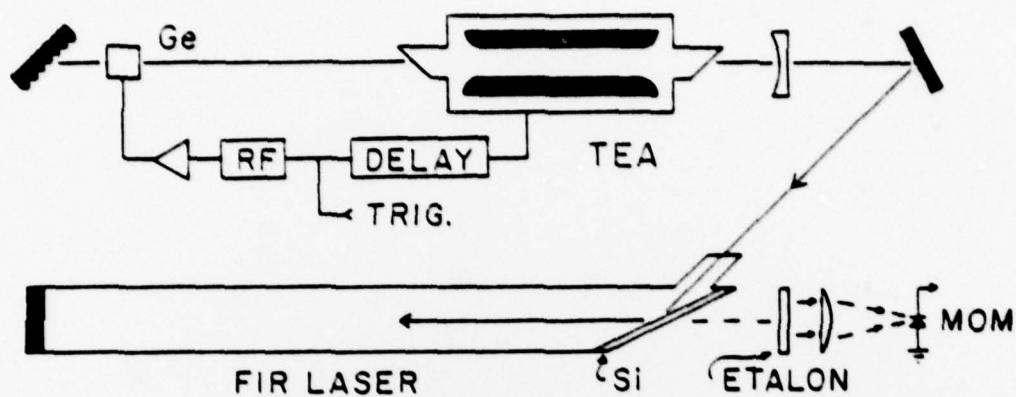
Fig. 1. Synchronously pumped FIR laser experiment.
