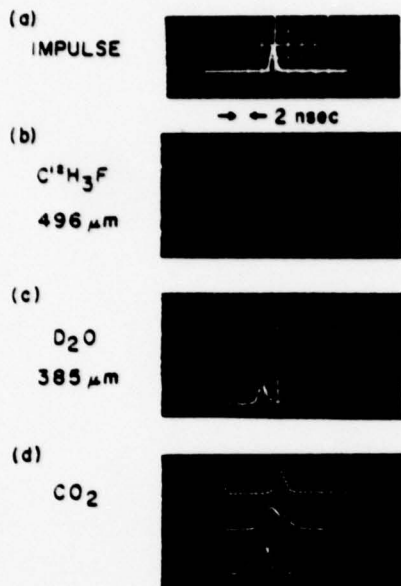
Fig. 2. Single pulses from the trains in Fig. 1 showing irregularities due to incomplete mode locking and normal locking. The impulse for (a) was a 400-psec triangular pulse.
