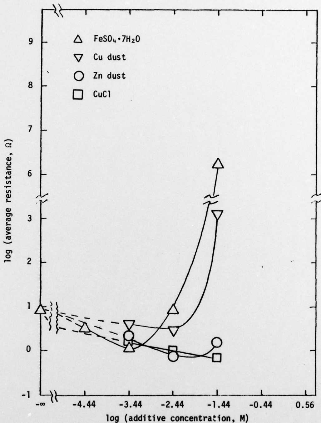
Figure 8. Average resistance of the silver deposit on ivory as a function of the additives (to AgNO 3 ) and their concentration. [Plating sequence: 42.5% H 3 PO 4 etch, WB, 100 g/l AgNO 3 + additive (pH~6) - 400 g/l FeSO 4 (pH~6), 10X.]
