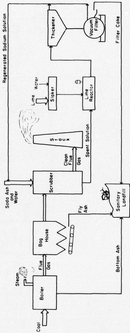
Figure 4. Double alkali scrubbing system.
