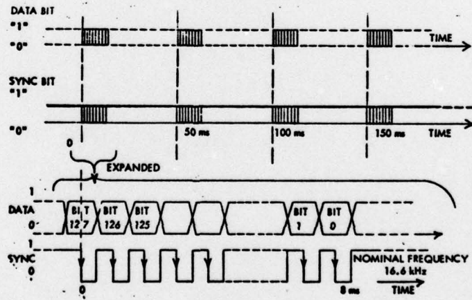
FIGURE 5. DATA BURST TIMING
