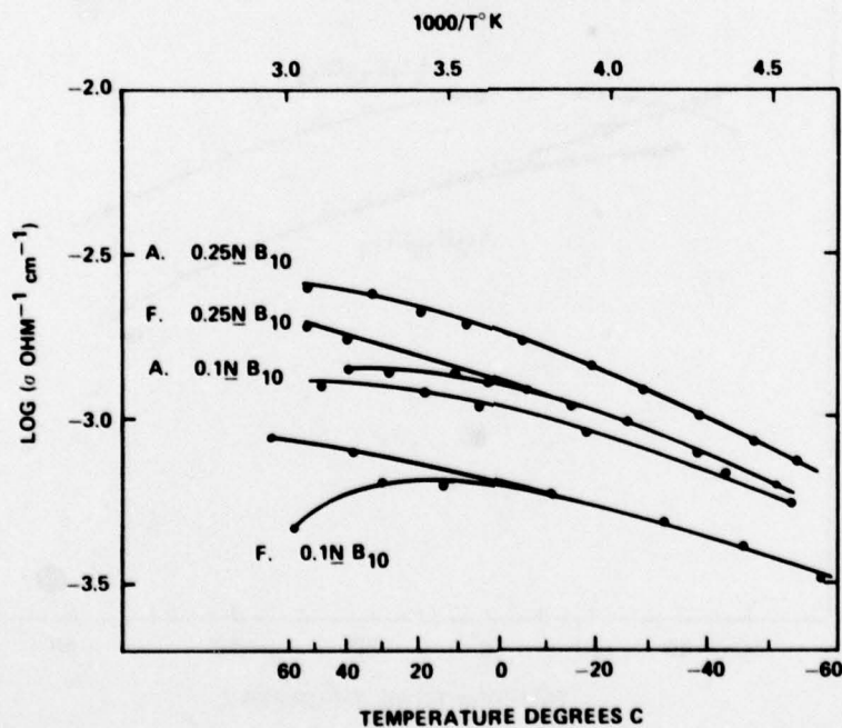
Figure 11. Log \sigma vs. 1000/T for 0.1N and 0.25N Li 2 B 10 Cl 10 in SOCl 2 Before (Fresh) and After (Aged) Storage at Room Temperature
