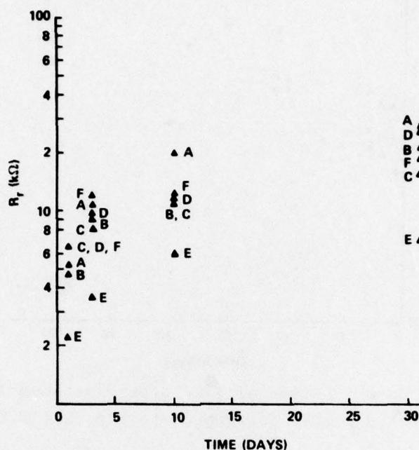
Figure 6. R_r as a Function of Time and Storage Temperature. For temperatures see Figure 5.
