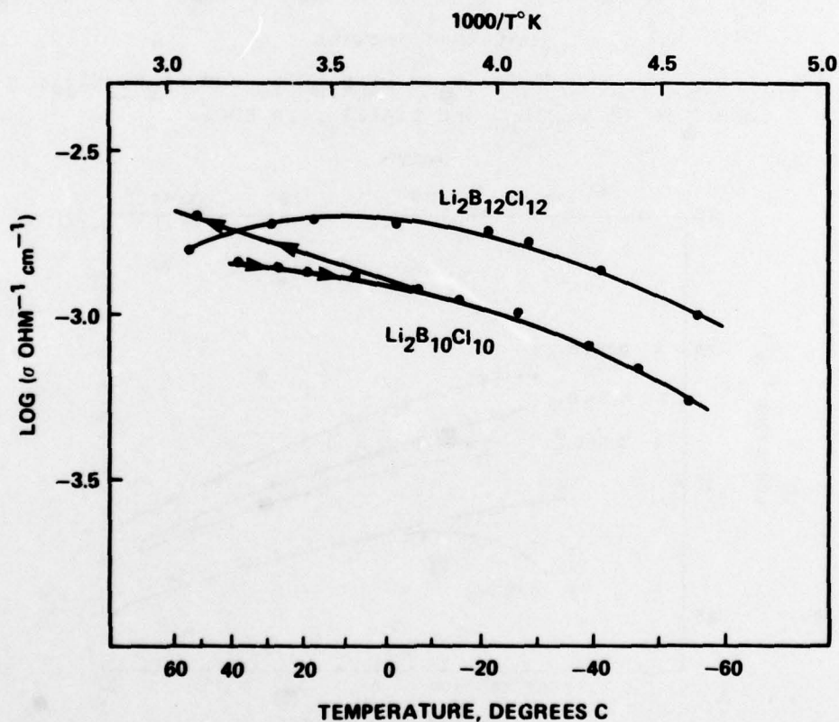
Figure 9. Log \sigma vs. 1000/T for 0.25N Li_2B_{10}Cl_{10} and Li_2B_{12}Cl_{12} in SOCl_2
