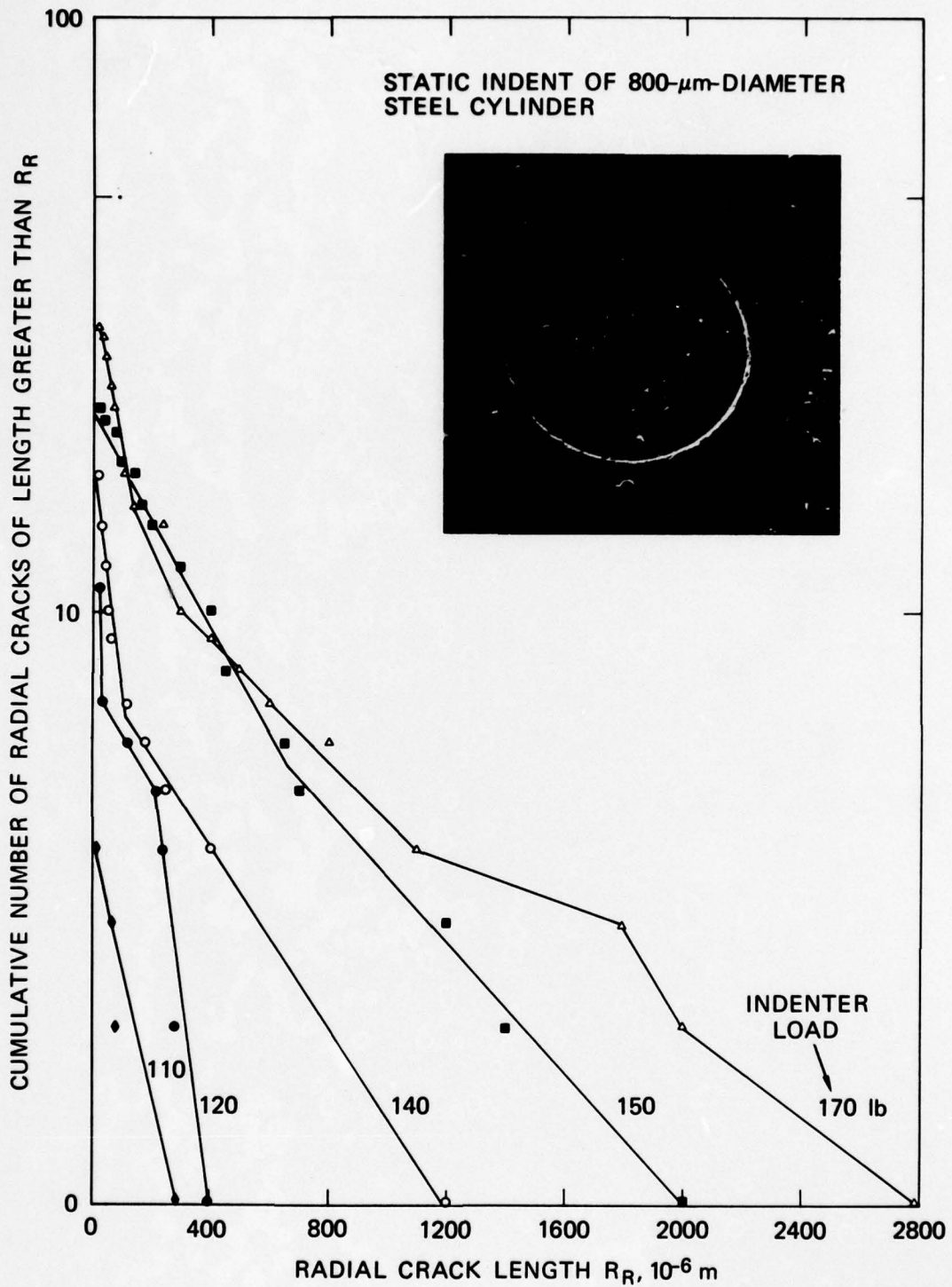
FIGURE 19 MEASURED SIZE DISTRIBUTIONS OF RADIAL CRACKS PRODUCED BY 800- \mu\text{m} -DIAMETER RIGHT CIRCULAR CYLINDERS UNDER VARIOUS INDENTATION LOADS
