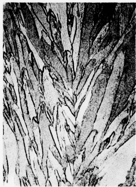
(c) GRAIN STRUCTURE NORMAL TO DEPOSITION DIRECTION
