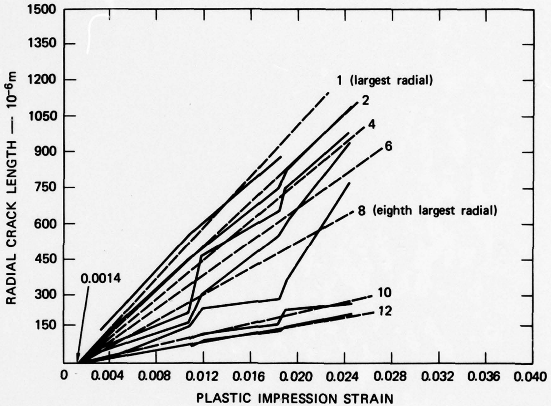
FIGURE 10 VARIATION OF RADIAL CRACK SIZE WITH PLASTIC IMPRESSION STRAIN FOR SEVERAL OF THE DOMINANT RADIALS PRODUCED BY IMPACT OF 800- \mu m DIAMETER SPHERES
