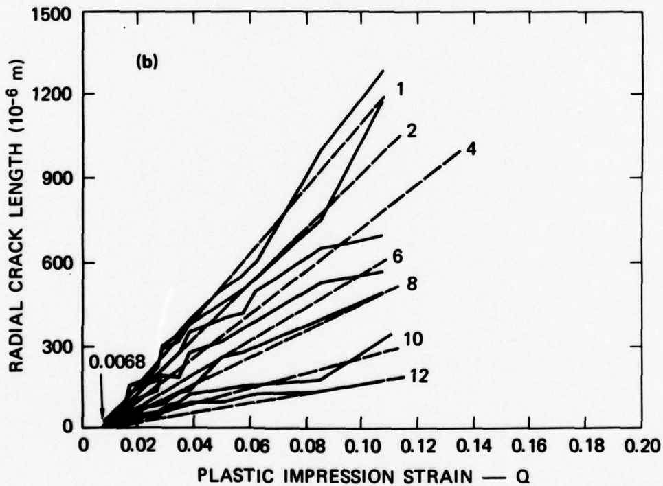
FIGURE 17 VARIATION OF NUMBER (a) AND SIZE (b) OF RADIAL CRACKS WITH PLASTIC IMPRESSION STRAIN FOR DOMINANT RADIALS PRODUCED BY QUASI-STATIC INDENTATION OF 400- \mu m-DIAMETER SPHERES
