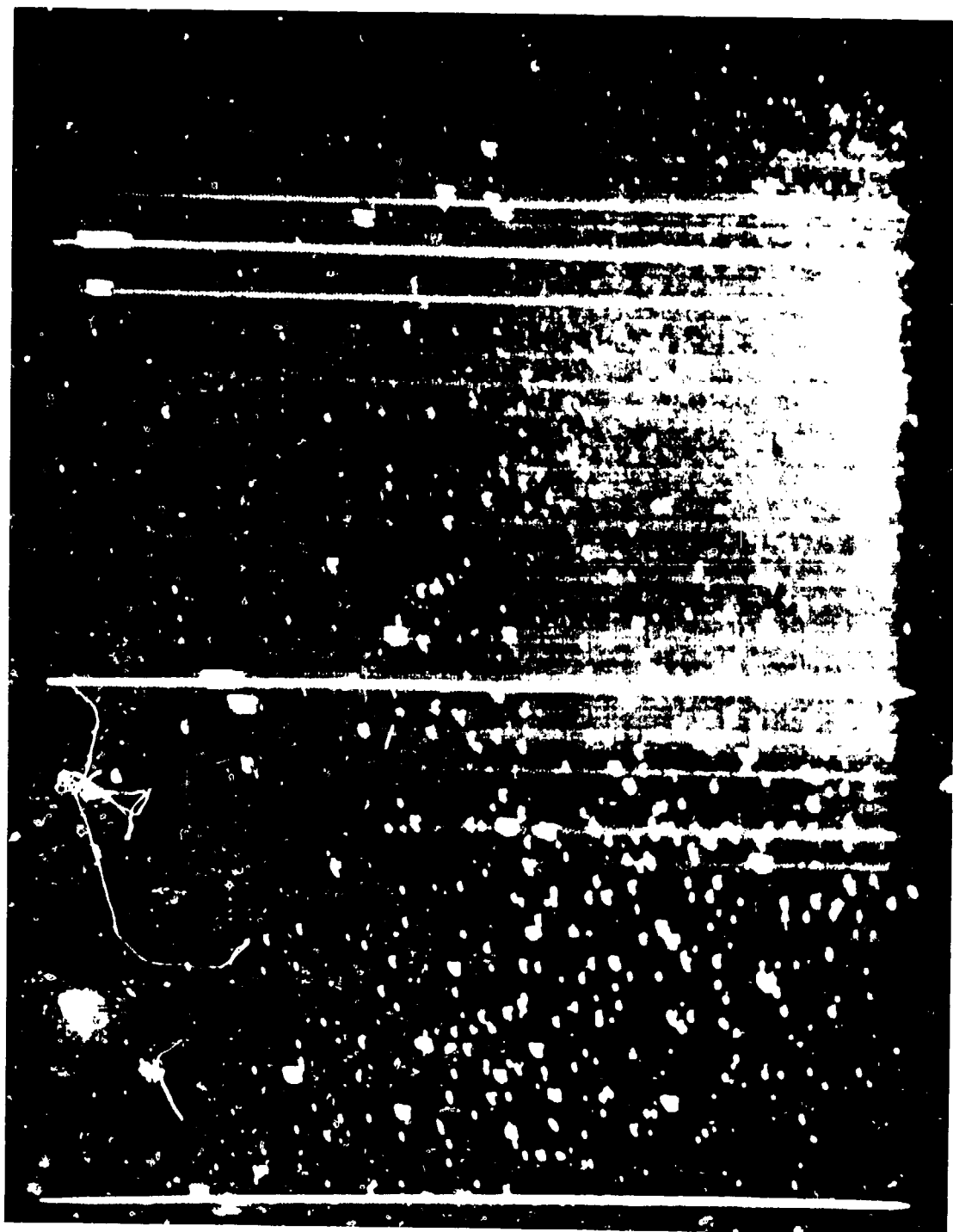
Figure 40 Dark Current Display of a CCD imager with 32 ms Integration Time. Backsid sandblast damage is on the upper third of the device.
