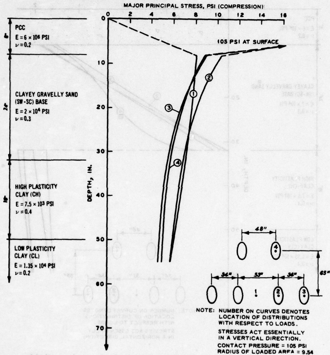
Figure A28. Distribution of major principal stress in a rigid pavement with a granular base loaded with a C-5A gear
