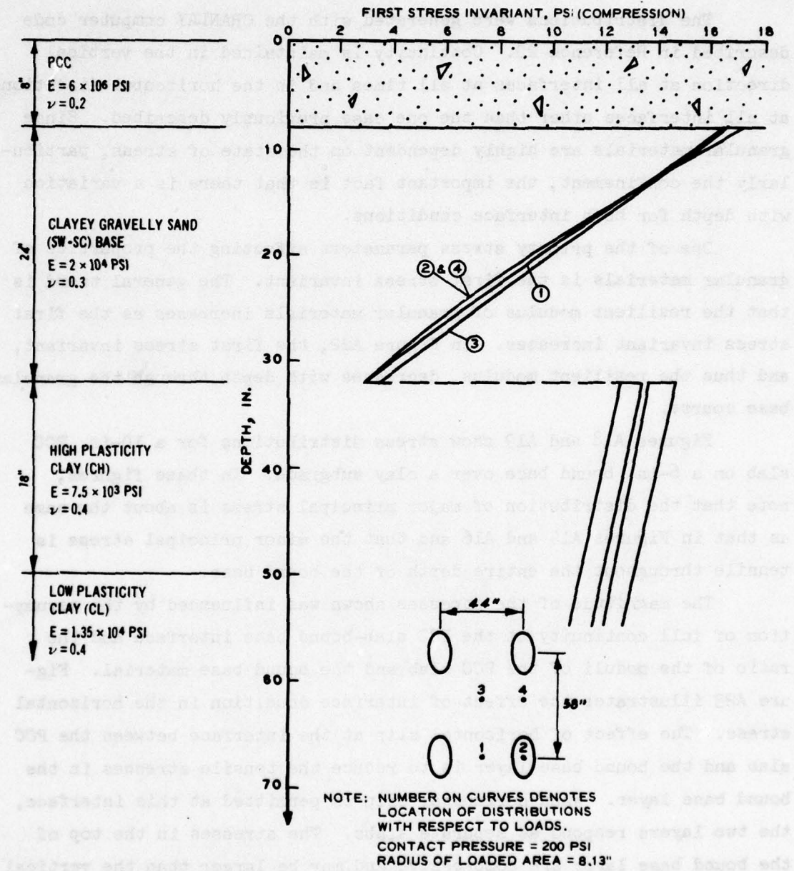
Figure A22. Distribution of the first stress invariant in a rigid pavement with a granular base loaded with a dual-tandem gear
