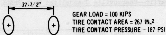
Figure B8. Schematic representation of loads used in Sharonville Channelized Traffic Test Track
