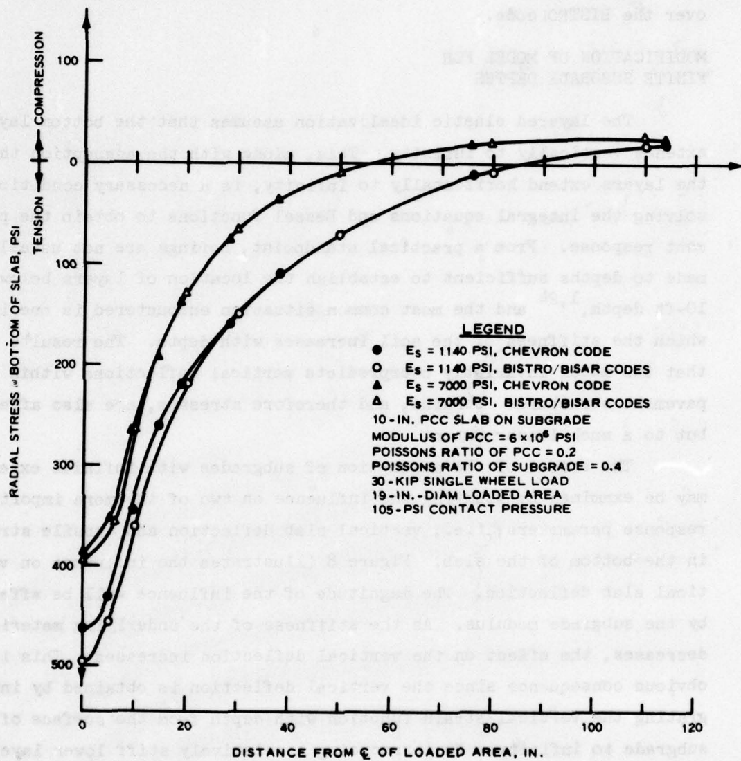
Figure 7. Comparison of tensile stress in bottom of PCC slab computed with CHEVRON and BISTRO/BISAR codes
