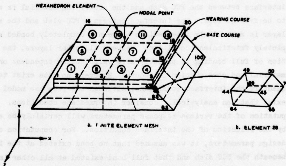
Figure 3. Pavement idealization using the finite element program (from Crawford and Katona 12 )
