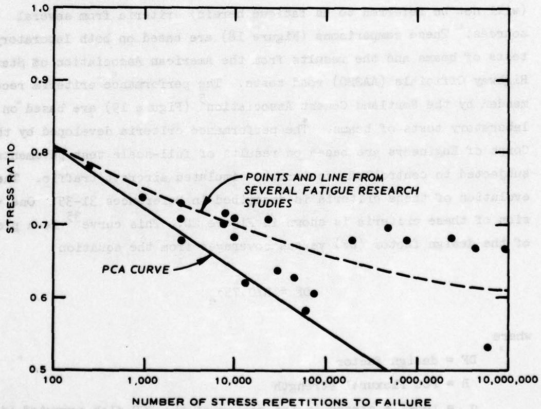
Figure 19. Fatigue curve for concrete subjected to flexural stresses 5
