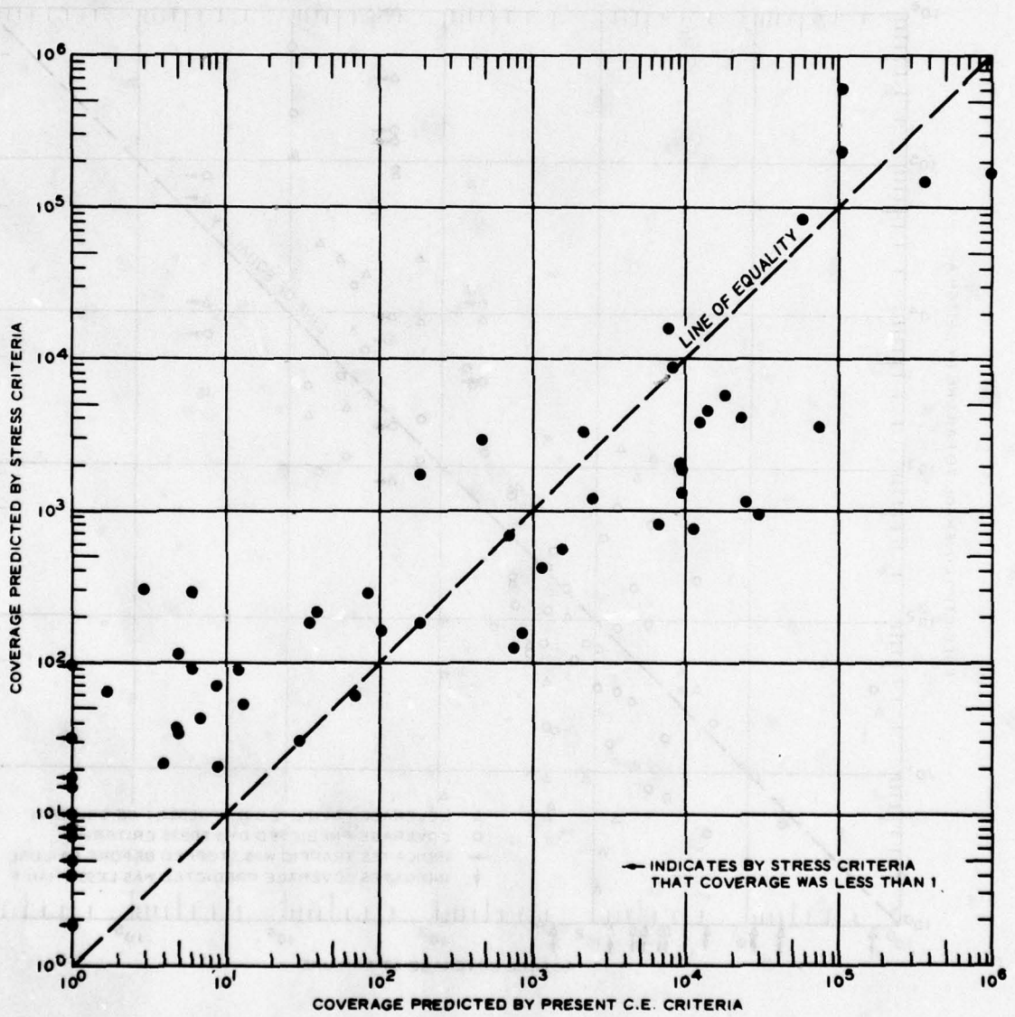
Figure 37. Comparison of coverage predicted by present design criteria with coverage predicted by stress criteria
