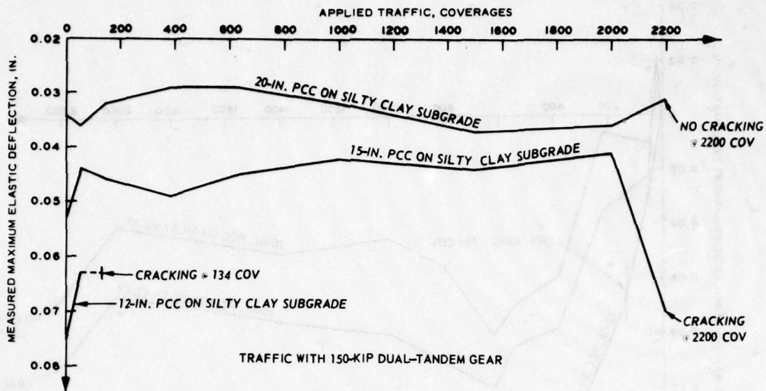
Figure 16. Elastic slab deflection versus traffic
