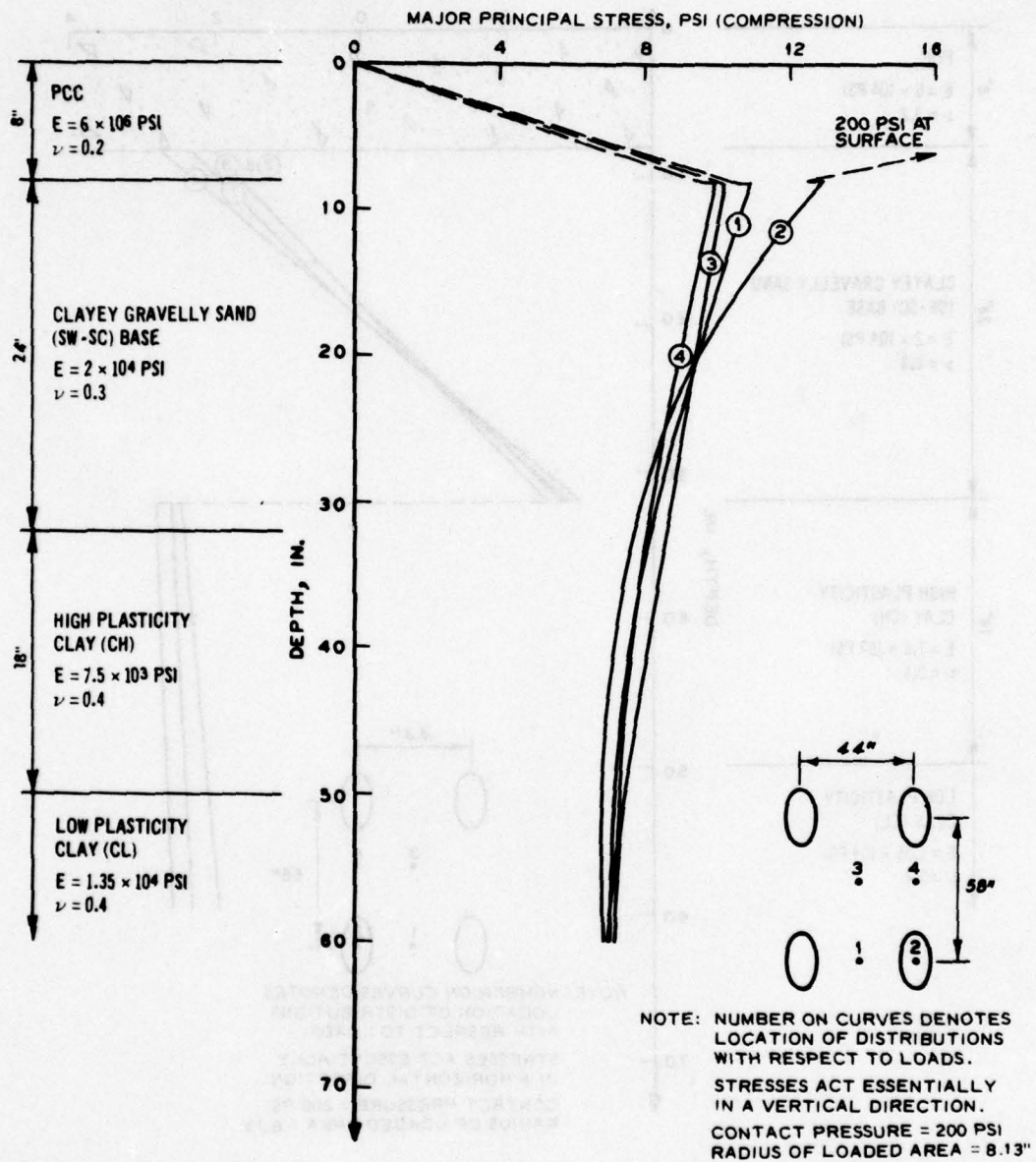
Figure A16. Distribution of major principal stress in a rigid pavement with a granular base loaded with a dual-tandem gear
