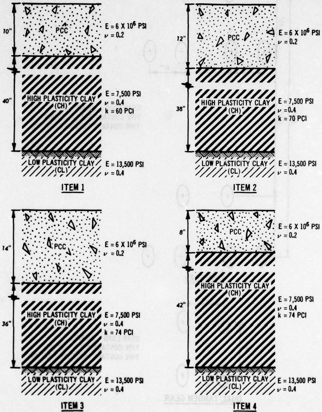
Figure B11. Description of test pavements in Multiple-Wheel Heavy Gear Load Test Track
