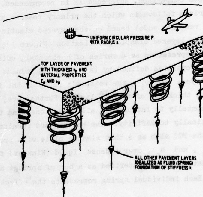
Figure 2. Westergaard pavement idealization (from Crawford and Katona 12 )
