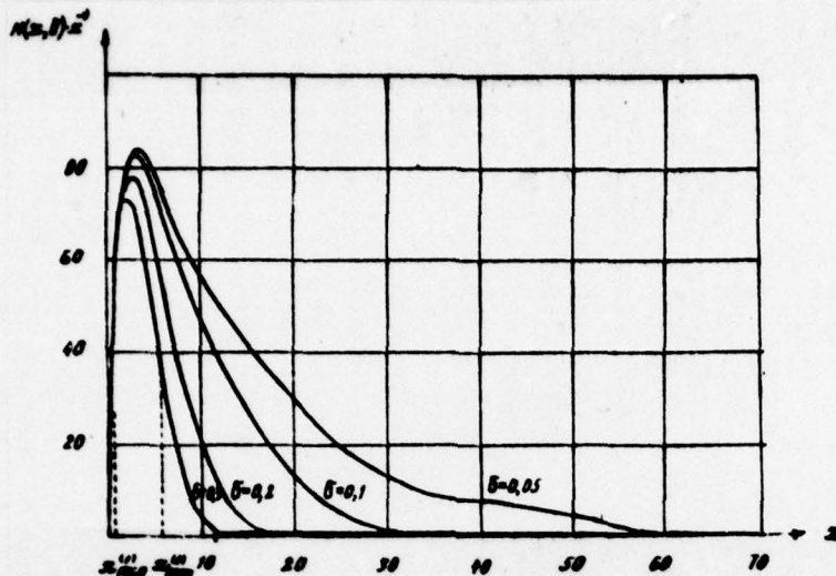
Fig. 6. Dependences M(x, \beta) \cdot x^{-v}
