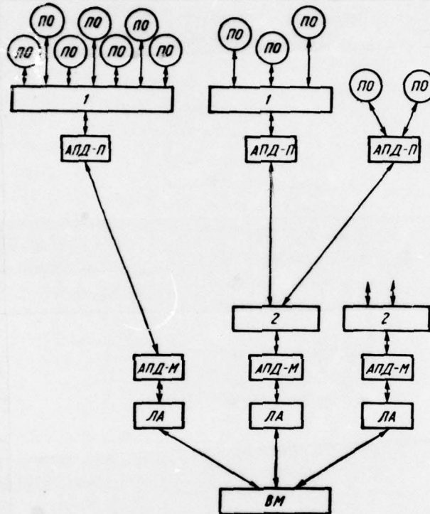
Fig. 2. Structural diagram of ASMO: 1 - commutator; 2 - concentrator.
