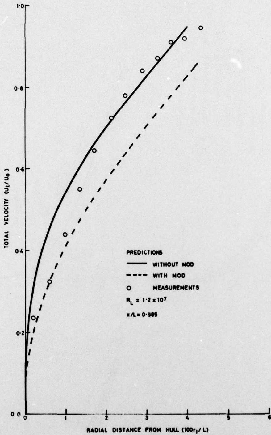
FIG. 15 VELOCITY PREDICTIONS AND MEASUREMENTS ON A BODY OF REVOLUTION WITH FULL AFTER-END
