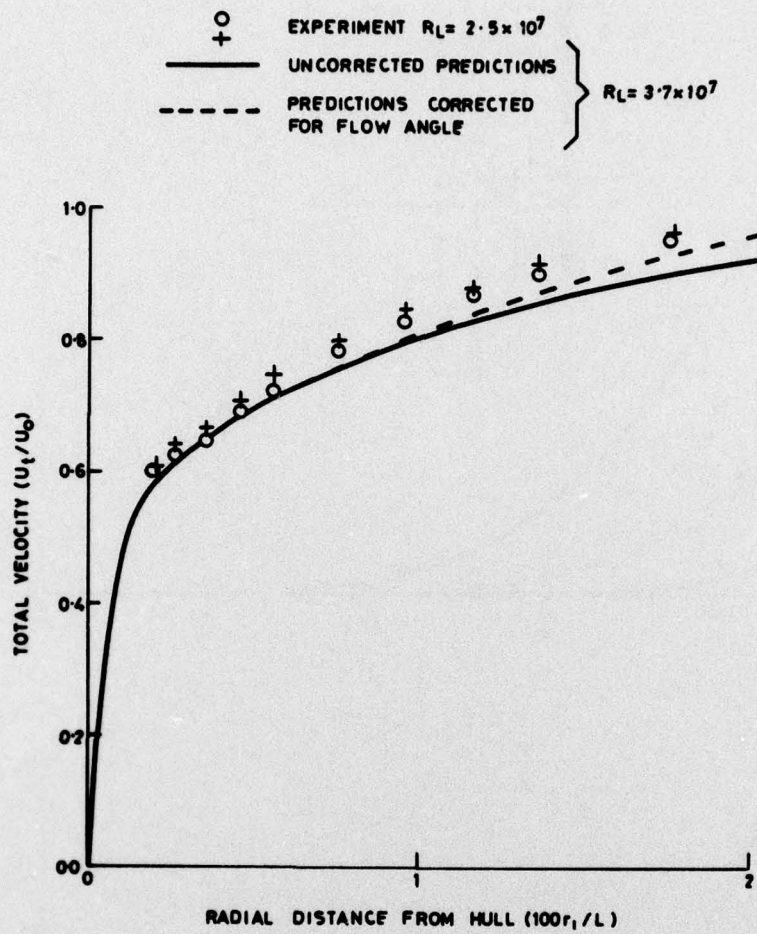
FIG.11 VELOCITY PREDICTIONS AND MEASUREMENTS ON BODY WITH FIN-DUCT
