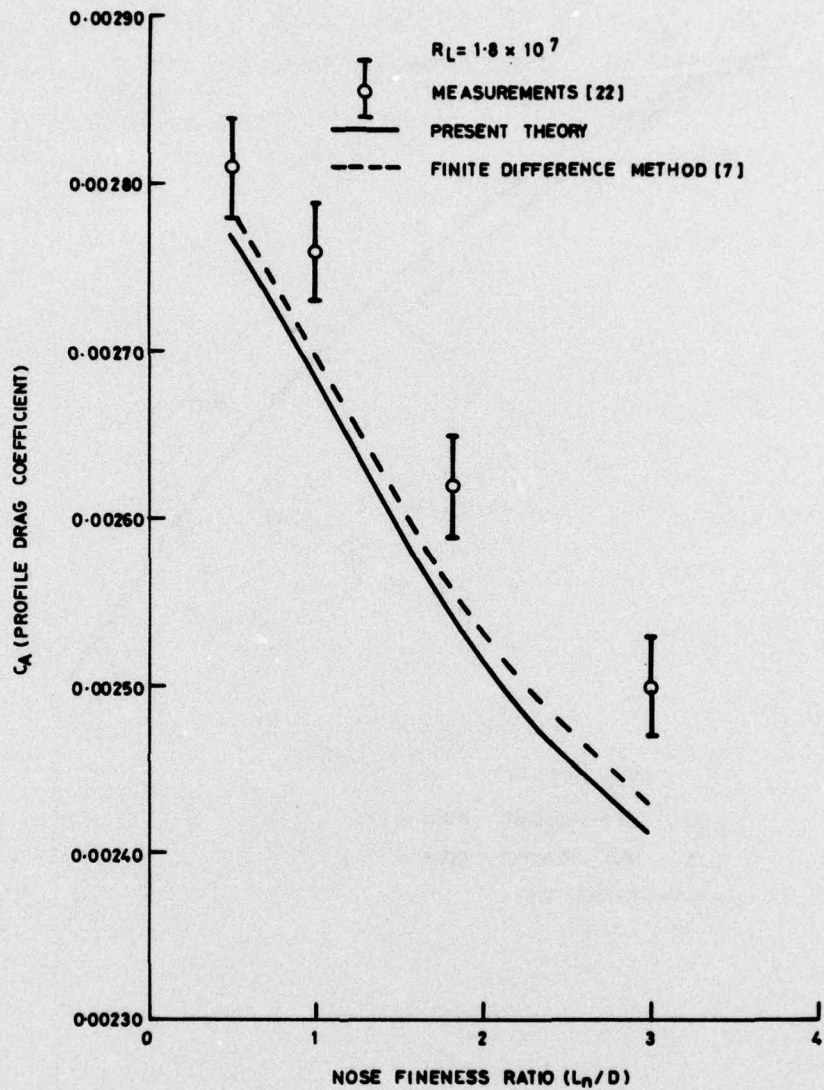
FIG. 2 THE EFFECT OF NOSE FINENESS RATIO ON DRAG
