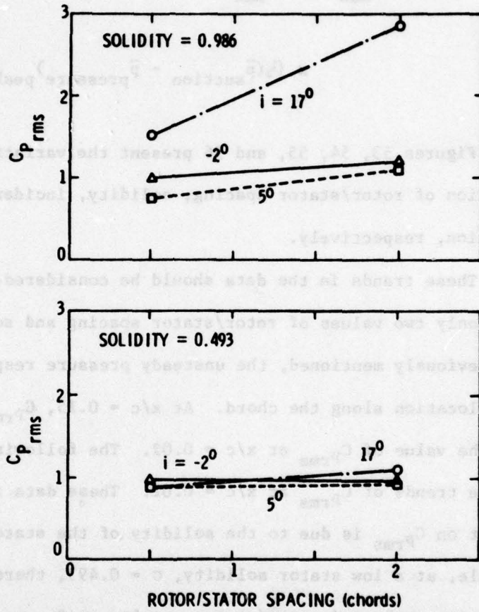
Figure 53. Variation of C_{p\ rms} with Rotor/Stator Spacing at x/c = 0.02
