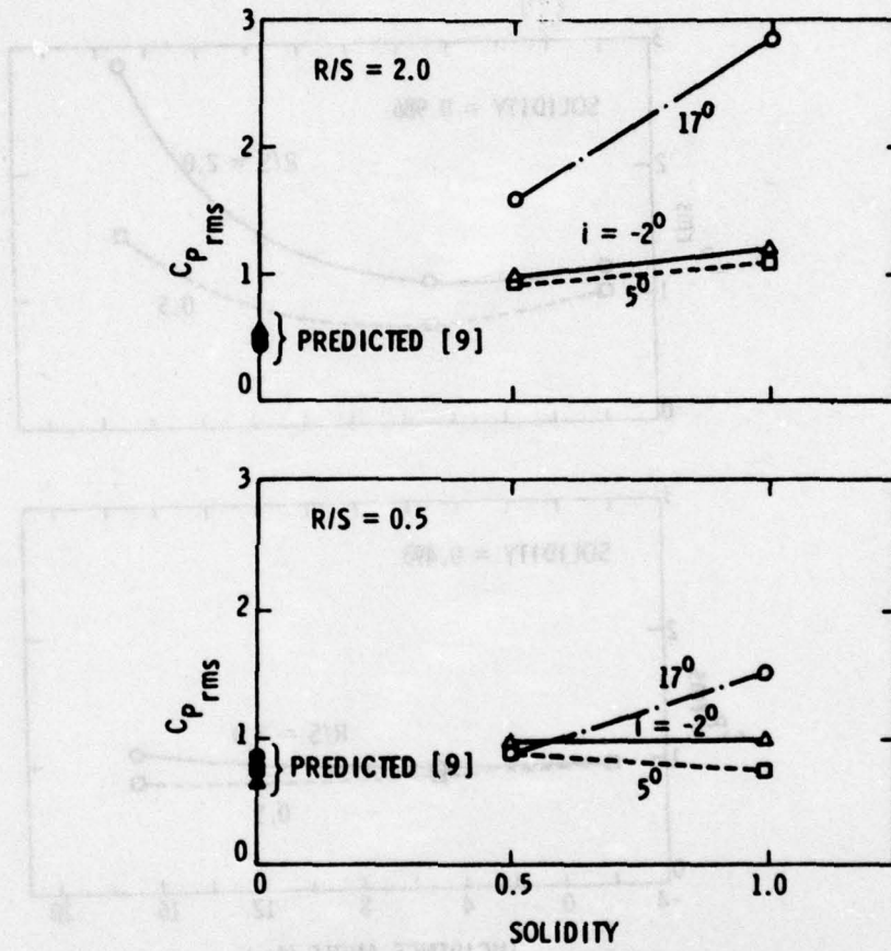
Figure 54. Variation of C_{p\text{ rms}} with Solidity at x/c = 0.02
