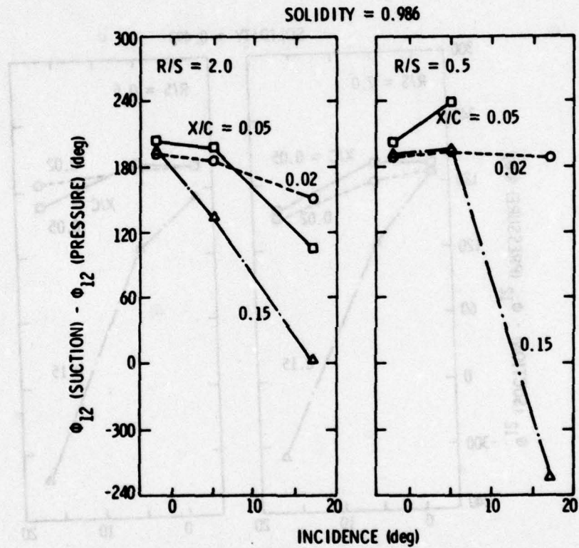
Figure 50. Suction and Pressure Surface Phase Angle Difference versus Incidence Angle--Blade Passing Harmonic (Continued)
