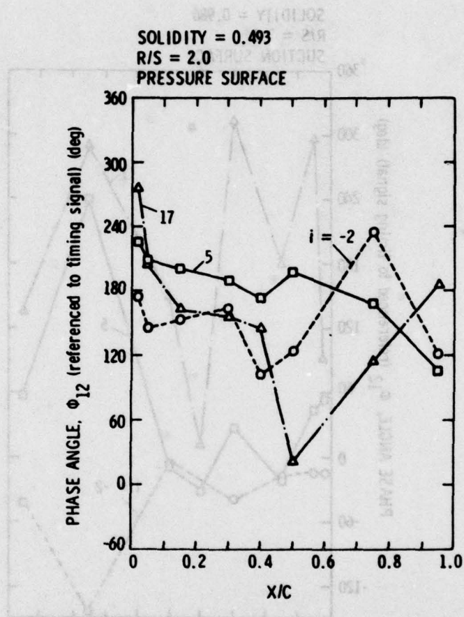
Figure 48. Unsteady Pressure Phase Angle versus x/c - R/S = 2.0 , \sigma = 0.493 (Continued)
