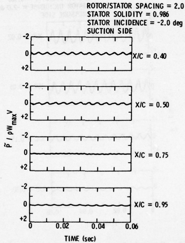
Figure 40. Unsteady Pressure Coefficient versus Real Time-Suction Surface, i = -2 deg (Continued)
