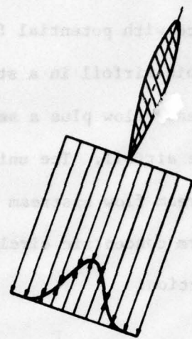
Figure 5. Rotor Wake Flow Relative to Rotor Blade
