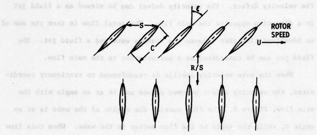
Figure 3. Geometry of Axial Flow Stage
