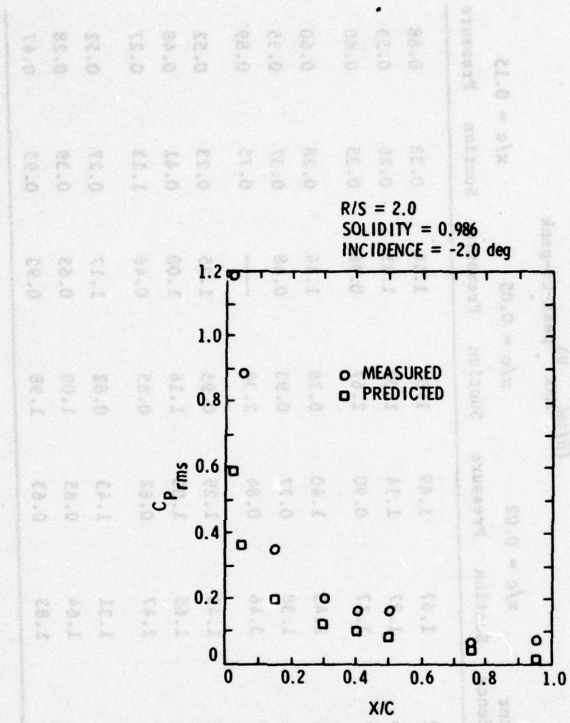
Figure 59. Comparison of Measured and Predicted C_{p,rms}
