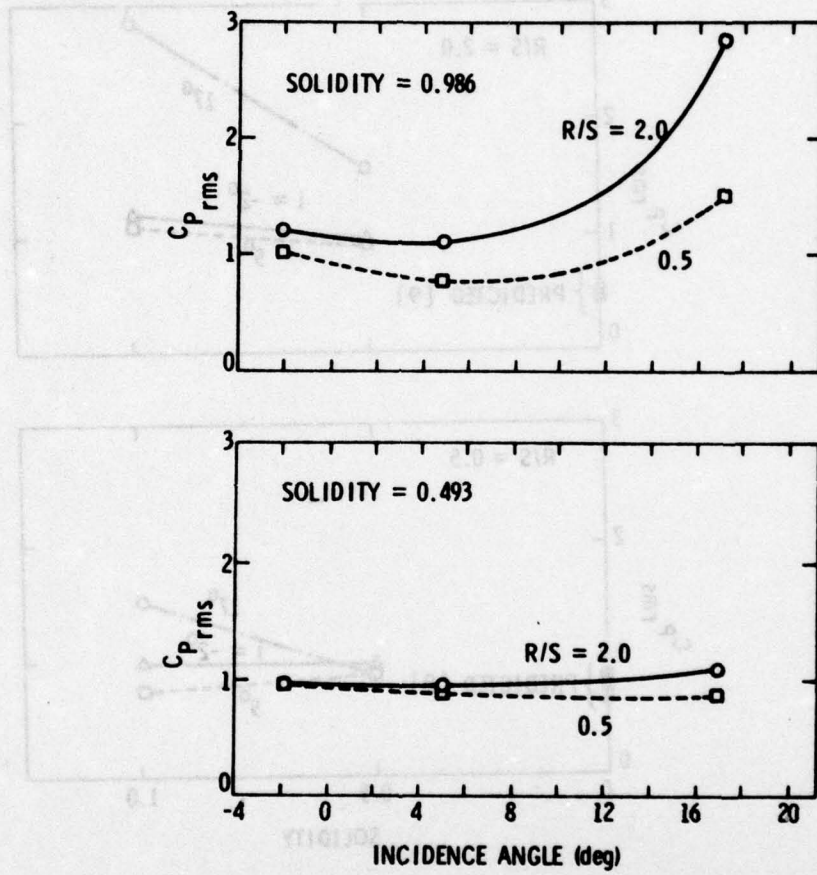
Figure 55. Variation of C_{p\text{rms}} with Incidence Angle at x/c = 0.02
