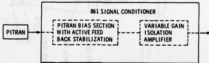
Figure 16. Pitran Signal Conditioner
