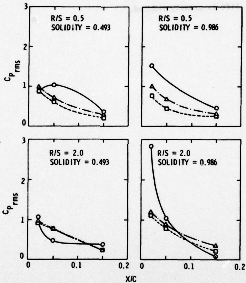
Figure 56. Variation of C_{p,rms} with Chordwise Position
