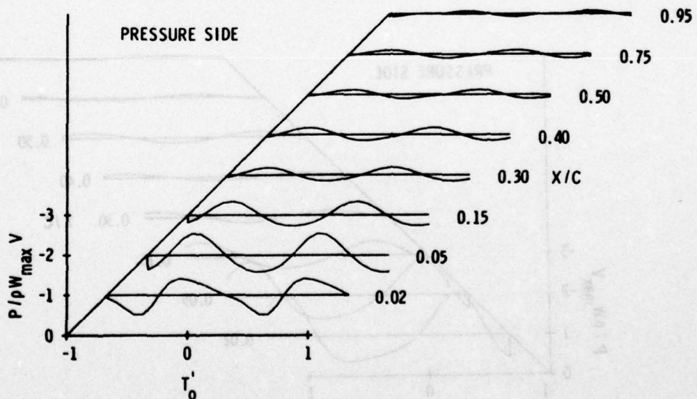
Figure 45. Unsteady Pressure Coefficient Variation During the Passage of a Single Rotor Wake, i = 17 deg
