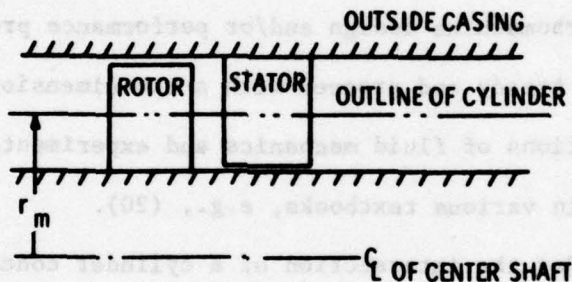
Figure 2. Schematic of Axial Flow Stage
