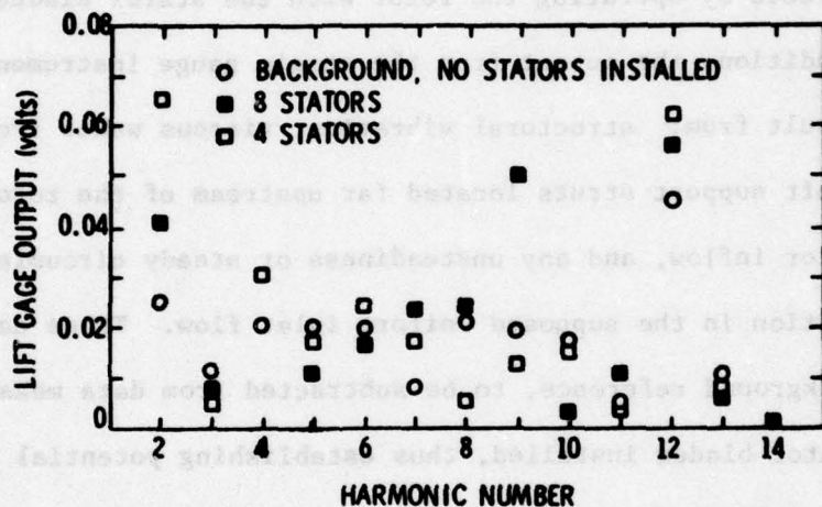
Figure 61. Magnitude of Unsteady Lift Gauge Output versus Harmonic Number, R/S = 0.5 and i = 17 deg
