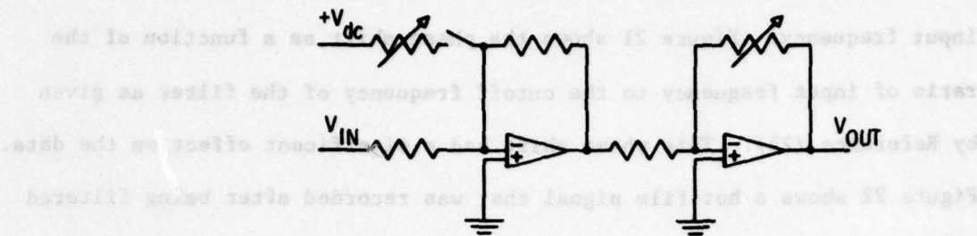
Figure 20. Schematic of Hot-Film Anemometer Signal Conditioner
