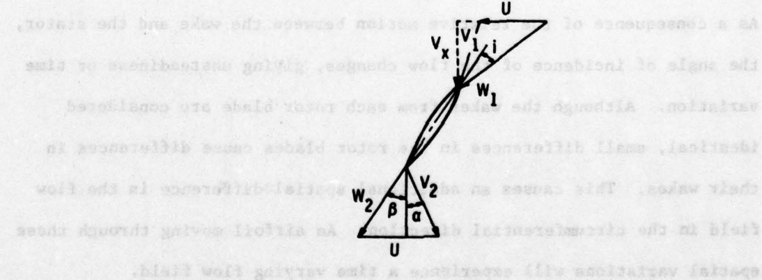
Figure 4. Rotor Velocity Diagram at Inlet and Exit
