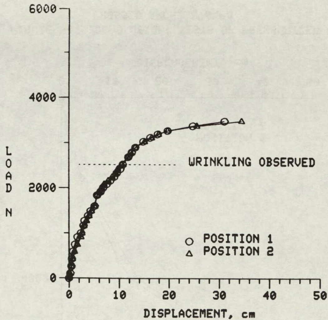
FIGURE 33. DEAD WEIGHT TESTS OF PRESSURIZED RIB TENTS CROSSED ARCH, 207KPA
