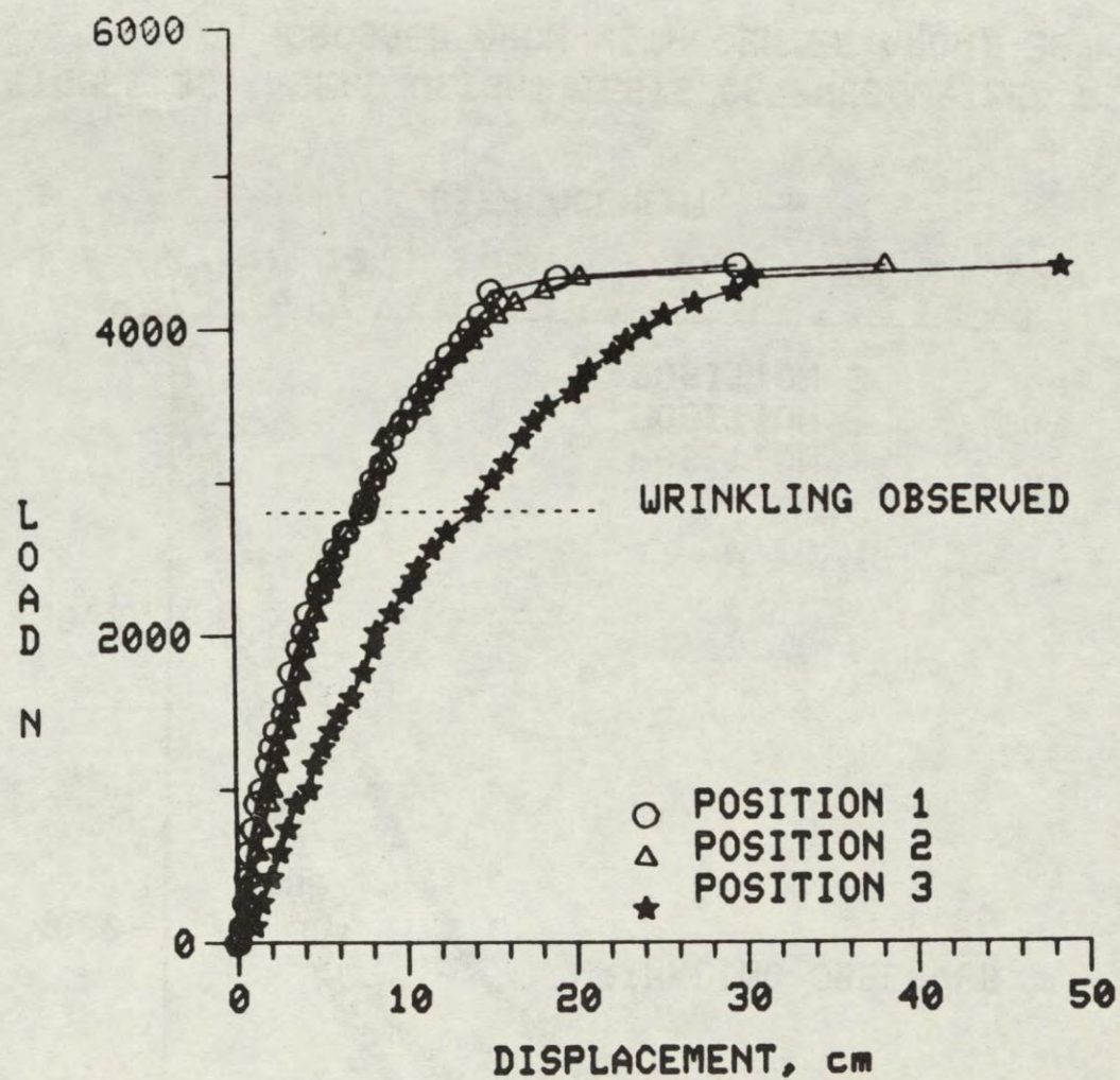
FIGURE 37. DEAD WEIGHT TESTS OF PRESSURIZED RIB TENTS CROSSED ARCH WITH CENTER ARCH, 138KPA
