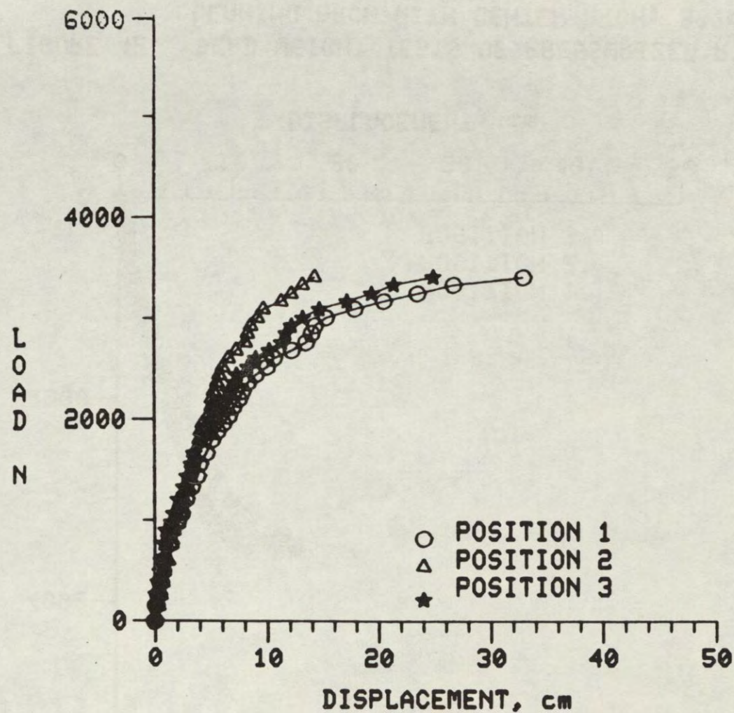
FIGURE 41. DEAD WEIGHT TESTS OF PRESSURIZED RIB TENTS LEANING ARCH WITH CENTERARCH, 138KPA
