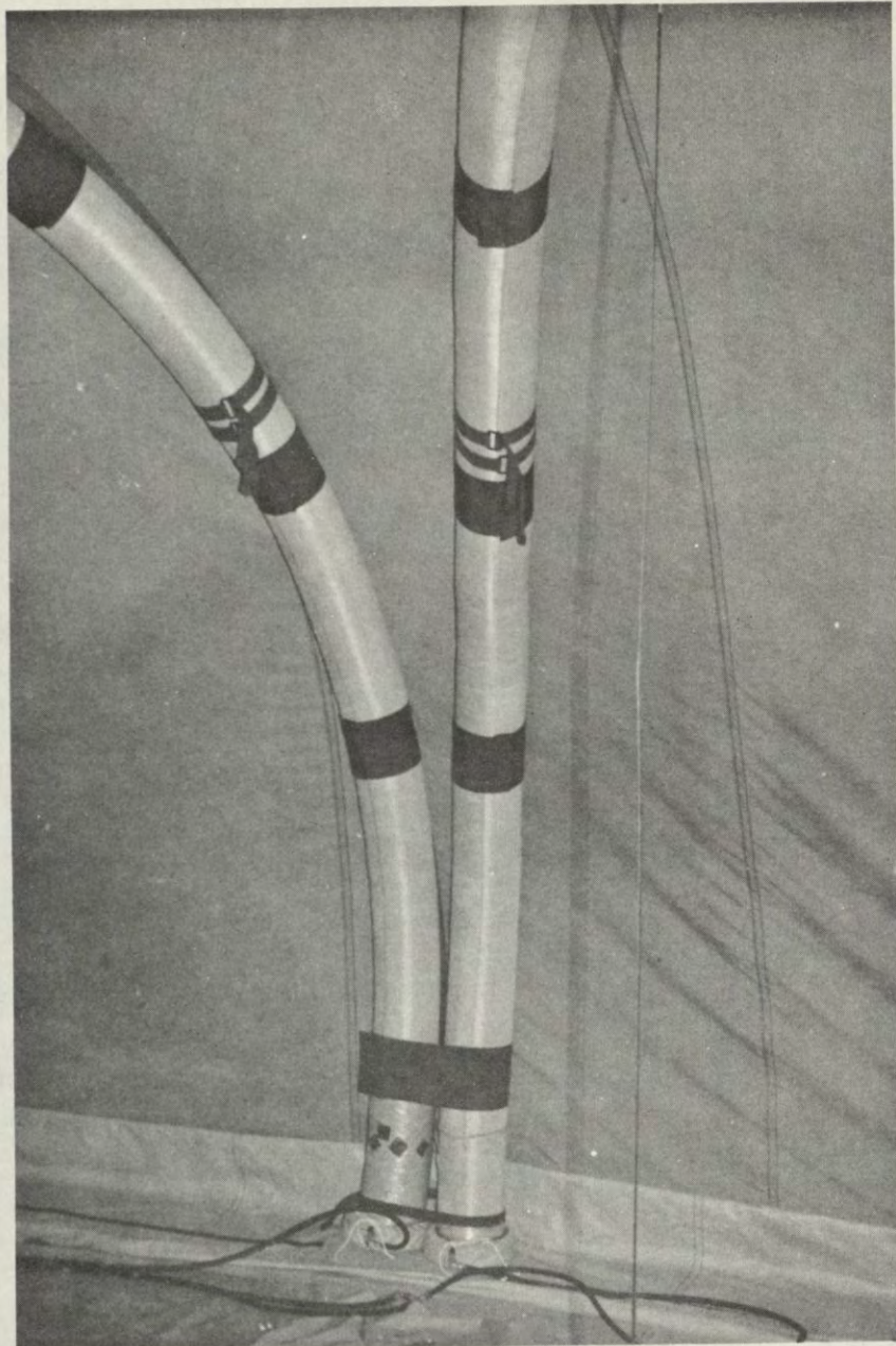
FIGURE 25. ATTACHMENT OF ENVIRONMENTAL BARRIER TO TENT FRAME.
