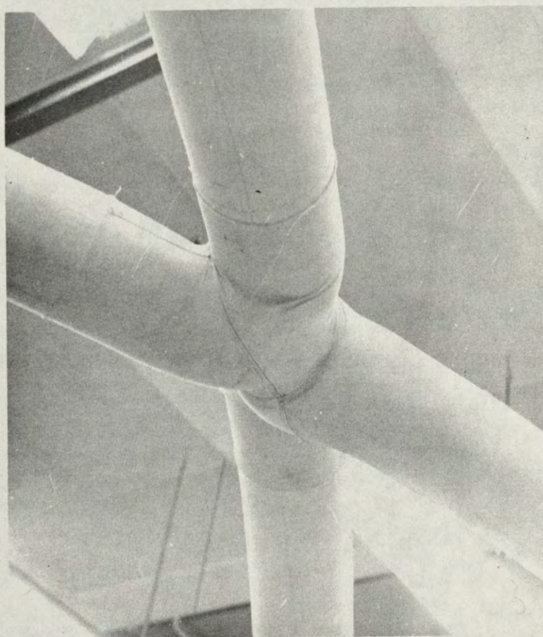
FIGURE 16. CONNECTION OF THE ARCHES IN THE CROSSED ARCH CONCEPT.
