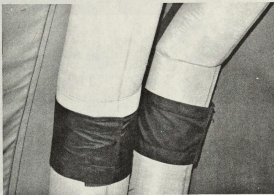
FIGURE 44. WRINKLING OF PRESSURE STABILIZED ARCHES UNDER LOAD.
