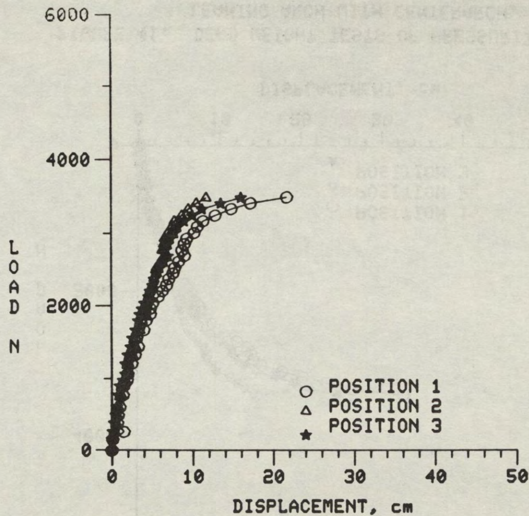
FIGURE 42. DEAD WEIGHT TESTS OF PRESSURIZED RIB TENTS LEANING ARCH WITH CENTER ARCH, 207KPA
