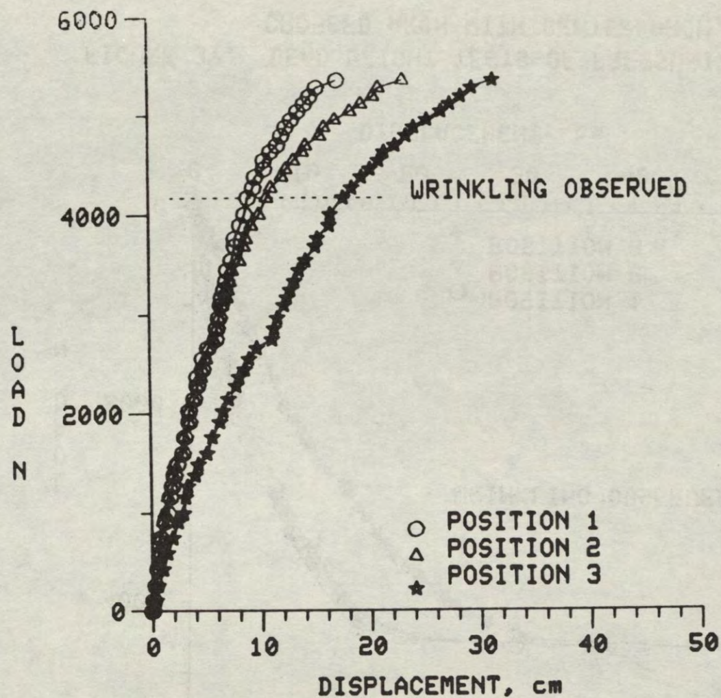
FIGURE 38. DEAD WEIGHT TESTS OF PRESSURIZED RIB TENTS CROSSED ARCH WITH CENTER ARCH, 207KPA
