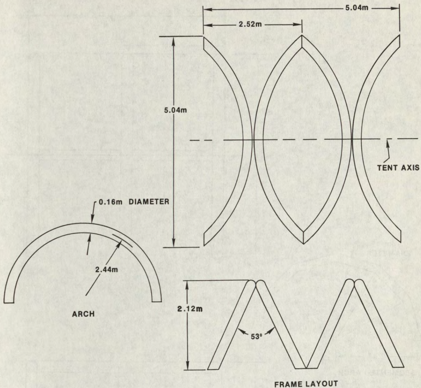
FIGURE 5. SKETCH OF ARCH AND FRAME LAYOUT FOR LEANING ARCH CONCEPT.
