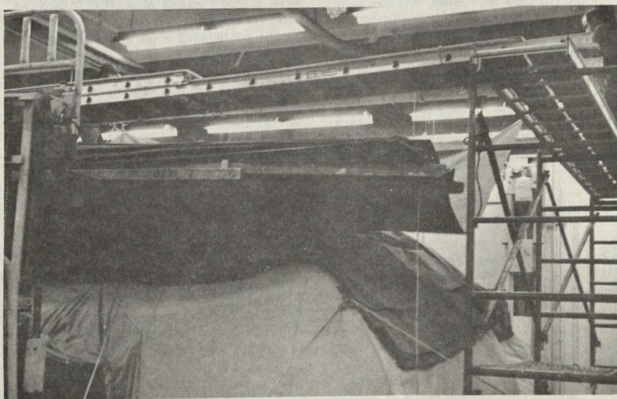
FIGURE 30. ILLUSTRATION OF THE SIMULATED SNOW LOAD TESTING TECHNIQUE.
