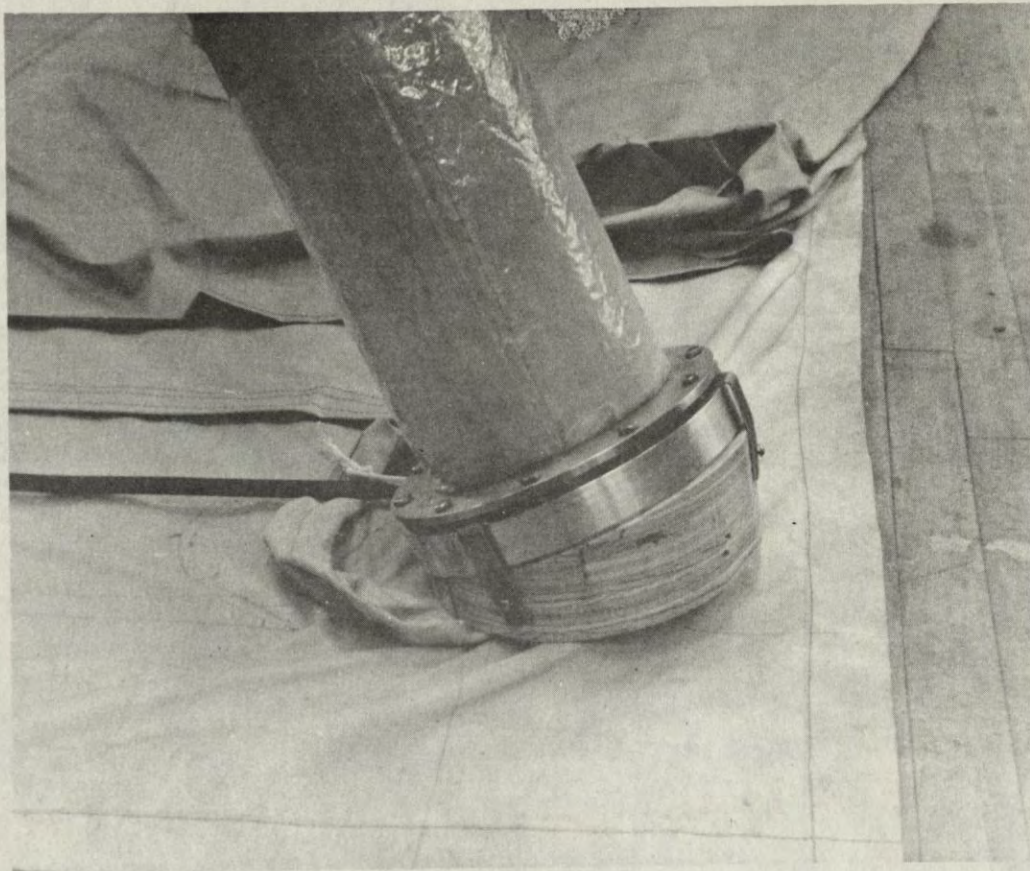
FIGURE 19. END CAP ADAPTER BLOCK USED WITH LEANING ARCH CONCEPT.
