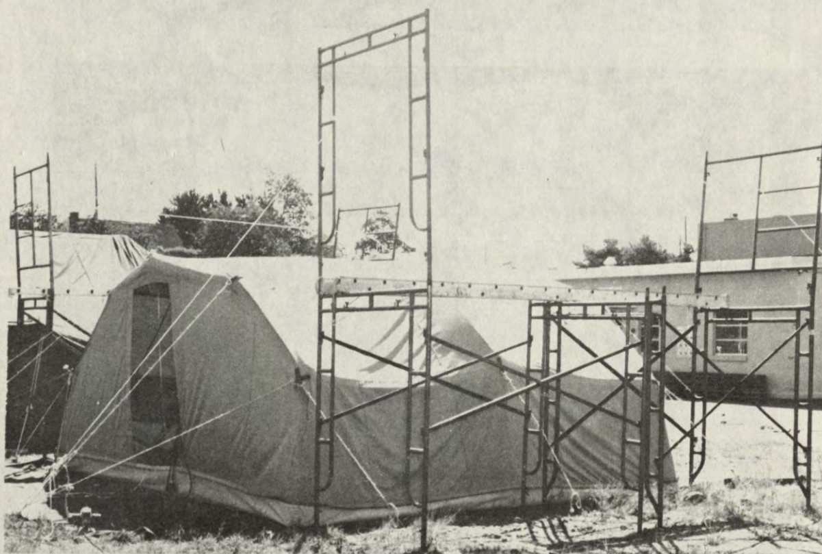
FIGURE 29. PROTOTYPE ARCH AND PURLIN TENT.
