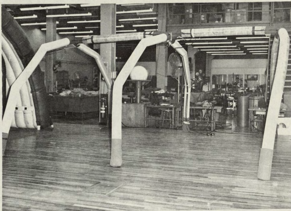
FIGURE 31. DOUBLE MODULE ARCH AND PURLIN FRAME ASSEMBLY WITH SEGMENTED ARCHES.
