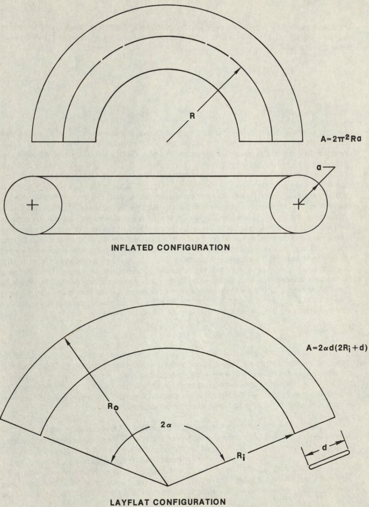
FIGURE 9. LAYFLAT AND INFLATED TUBE CONFIGURATIONS.
