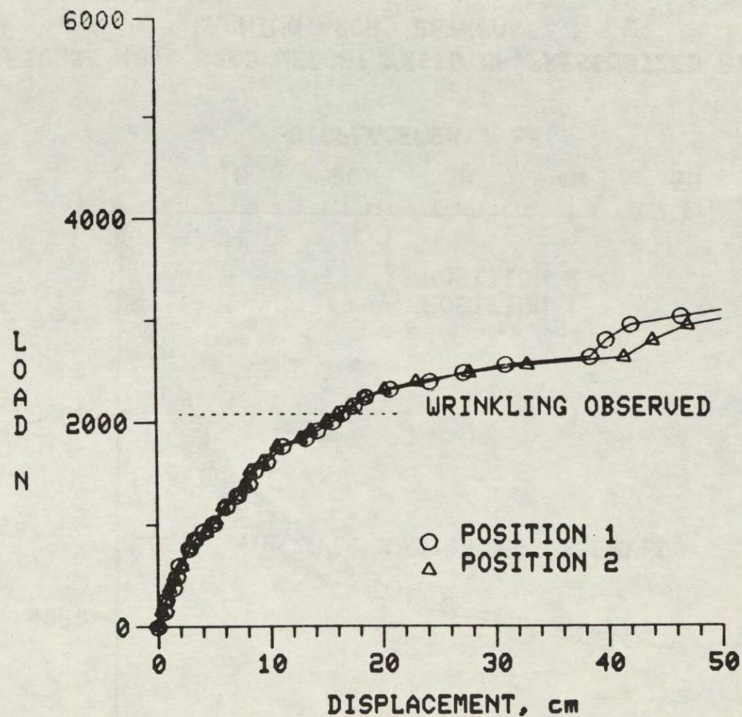
FIGURE 39. DEAD WEIGHT TESTS OF PRESSURIZED RIB TENTS LEANING ARCH, 138KPA
