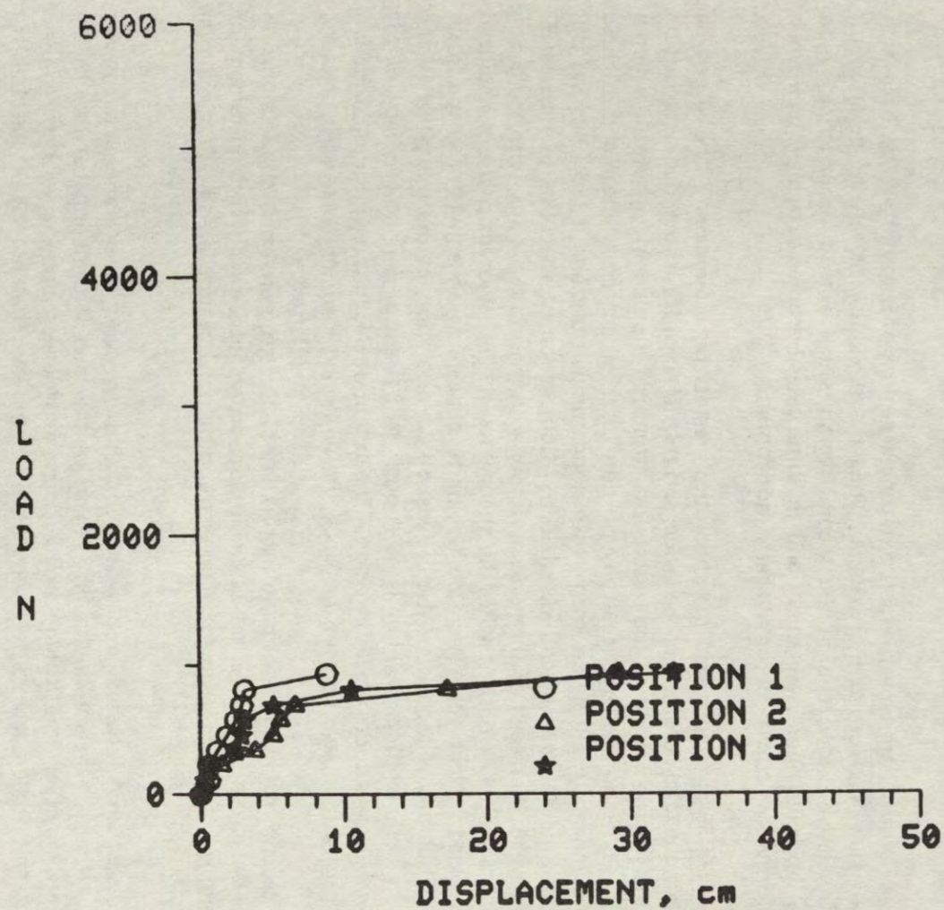
FIGURE 43. DEAD WEIGHT TESTS OF PRESSURIZED RIB TENTS ARCH AND PURLIN, 69KPA
