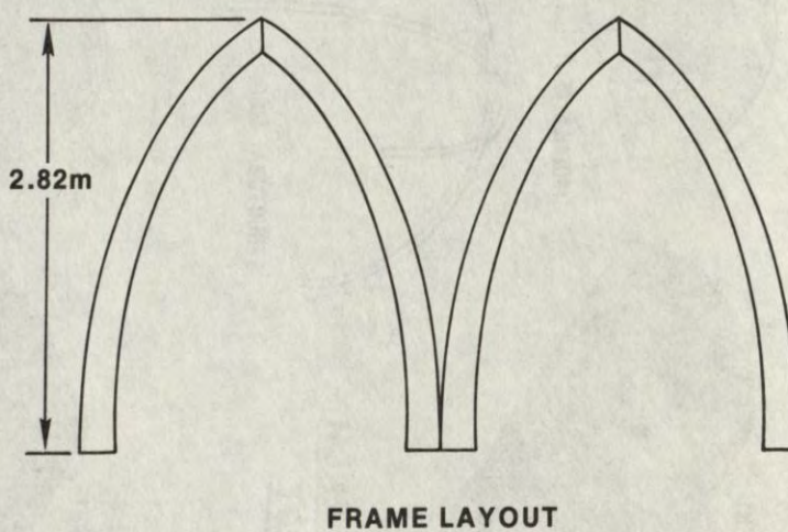
FIGURE 3. SKETCH OF ARCH AND FRAME LAYOUT FOR THE CROSSED ARCH CONCEPT.
