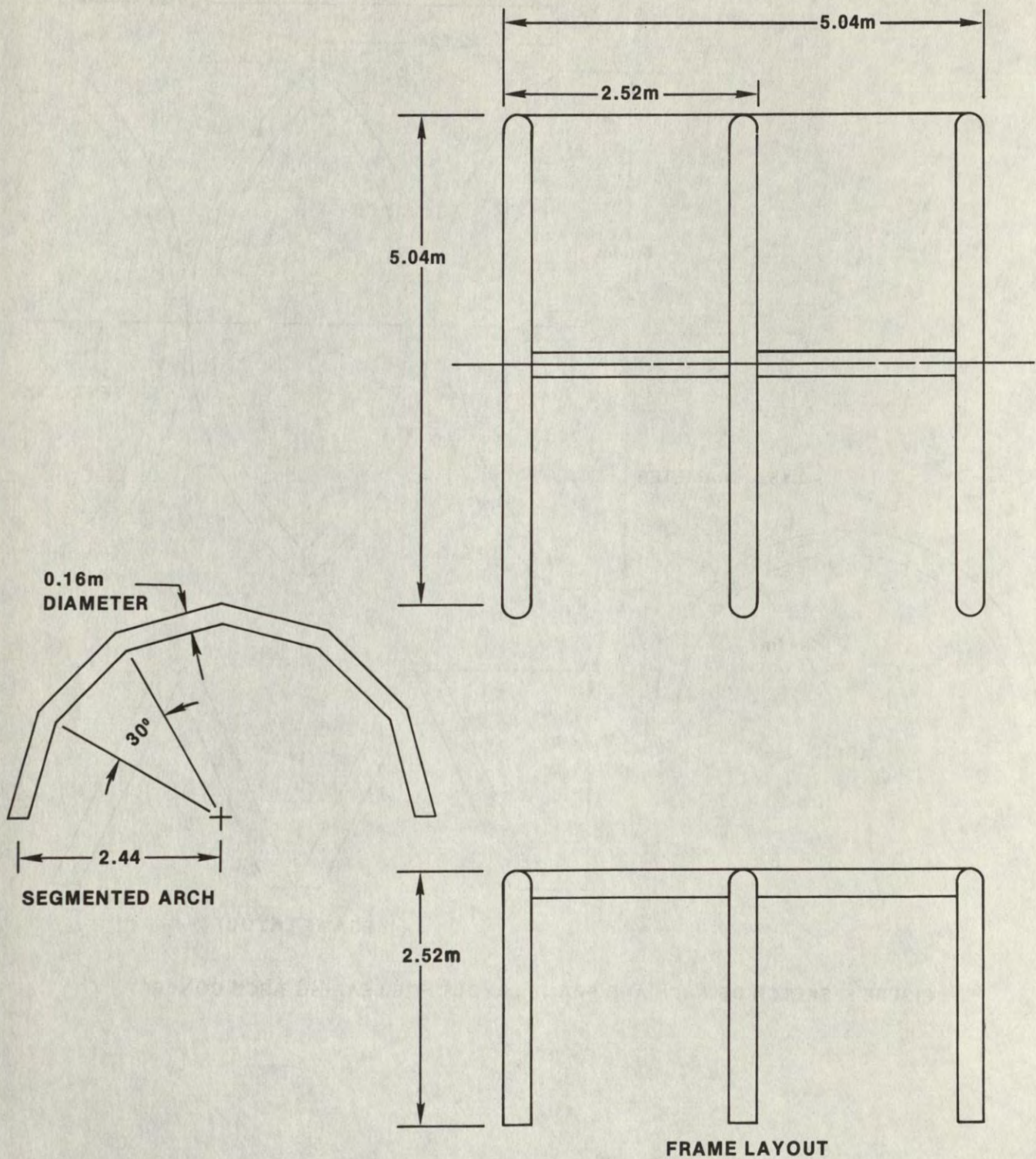
FIGURE 6. SKETCH OF ARCH AND FRAME LAYOUT FOR ARCH AND PURLIN CONCEPT.
