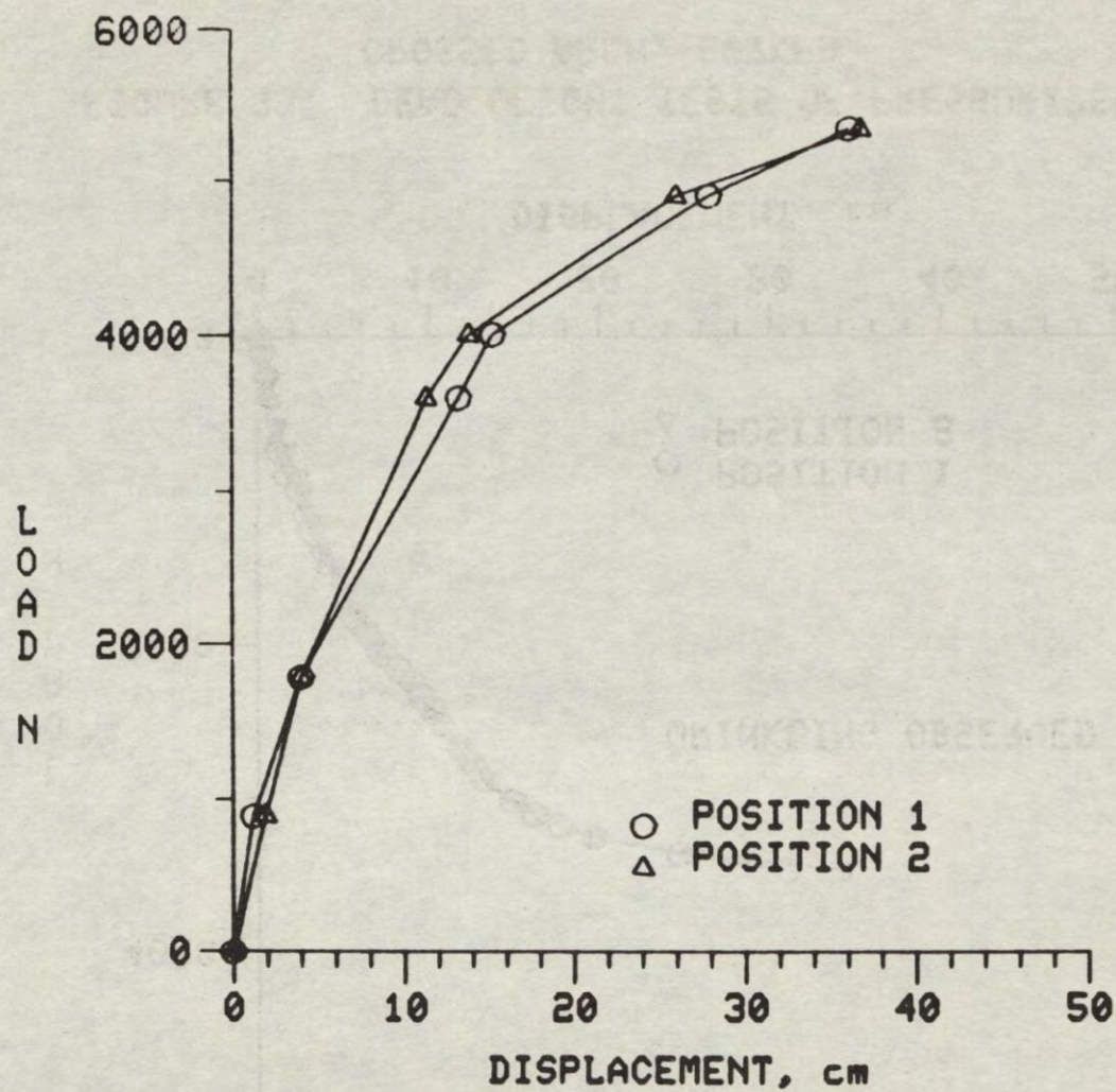
FIGURE 34. DEAD WEIGHT TESTS OF PRESSURIZED RIB TENTS CROSSED ARCH, 276KPA
