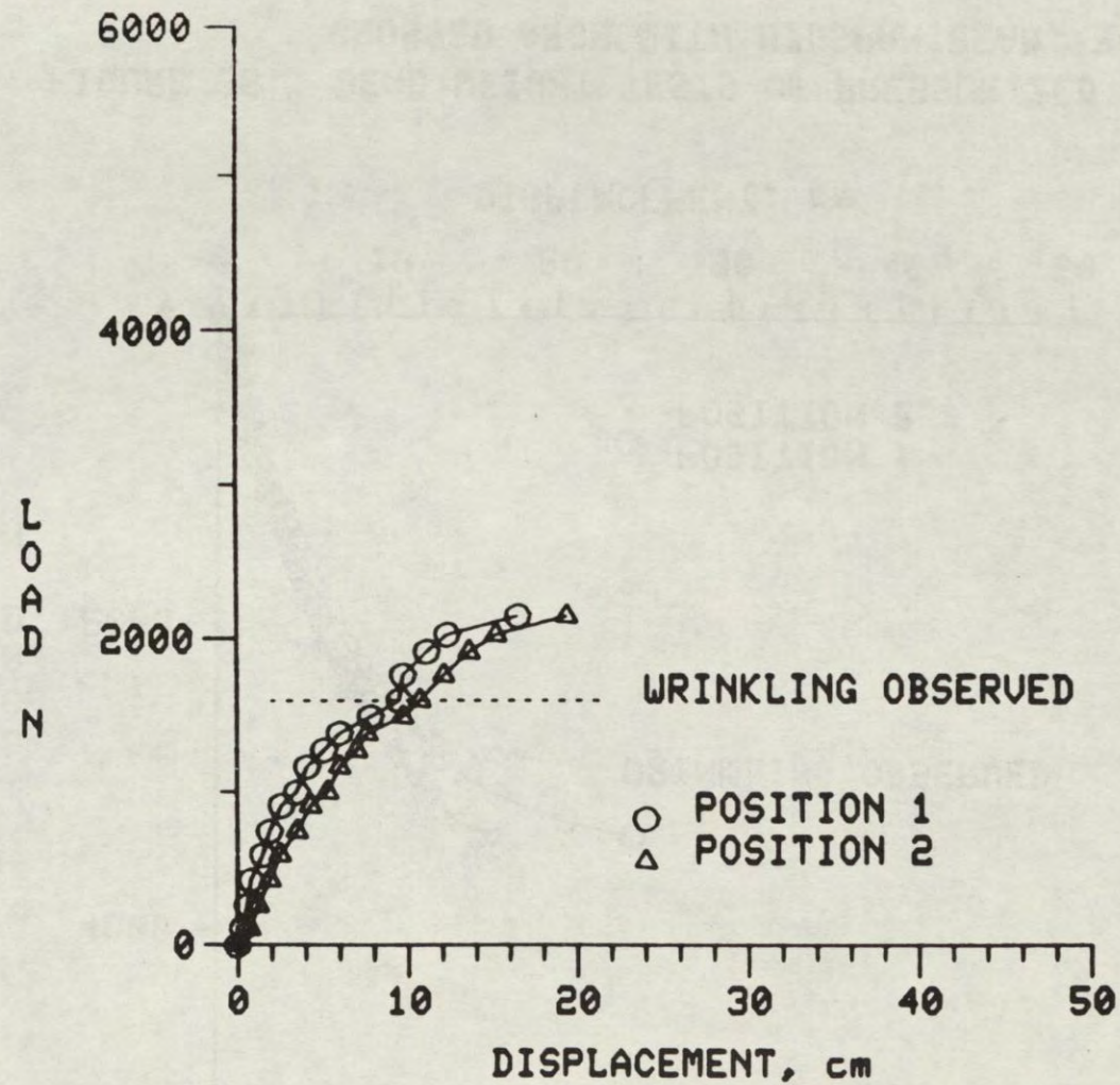
FIGURE 35. DEAD WEIGHT TESTS OF PRESSURIZED RIB TENTS CROSSED ARCH WITH MIDSPAN BEAM, 138KPA
