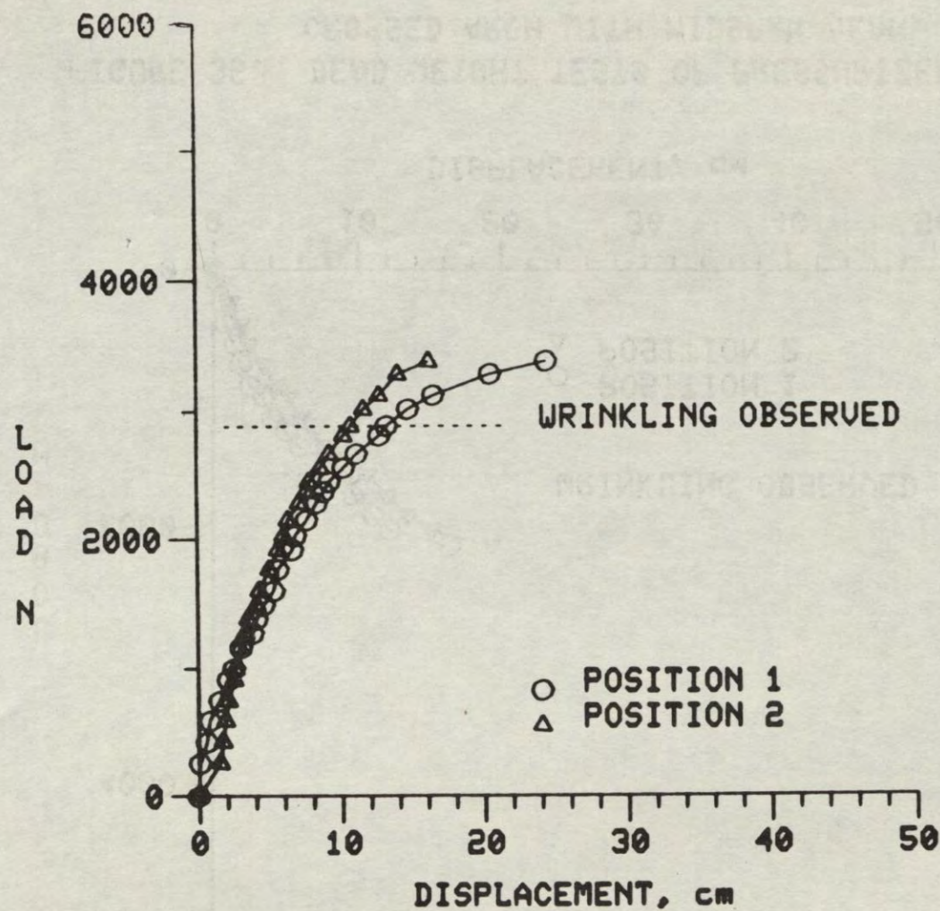
FIGURE 36. DEAD WEIGHT TESTS OF PRESSURIZED RIB TENTS CROSSED ARCH WITH MIDSPAN BEAM, 207KPA
