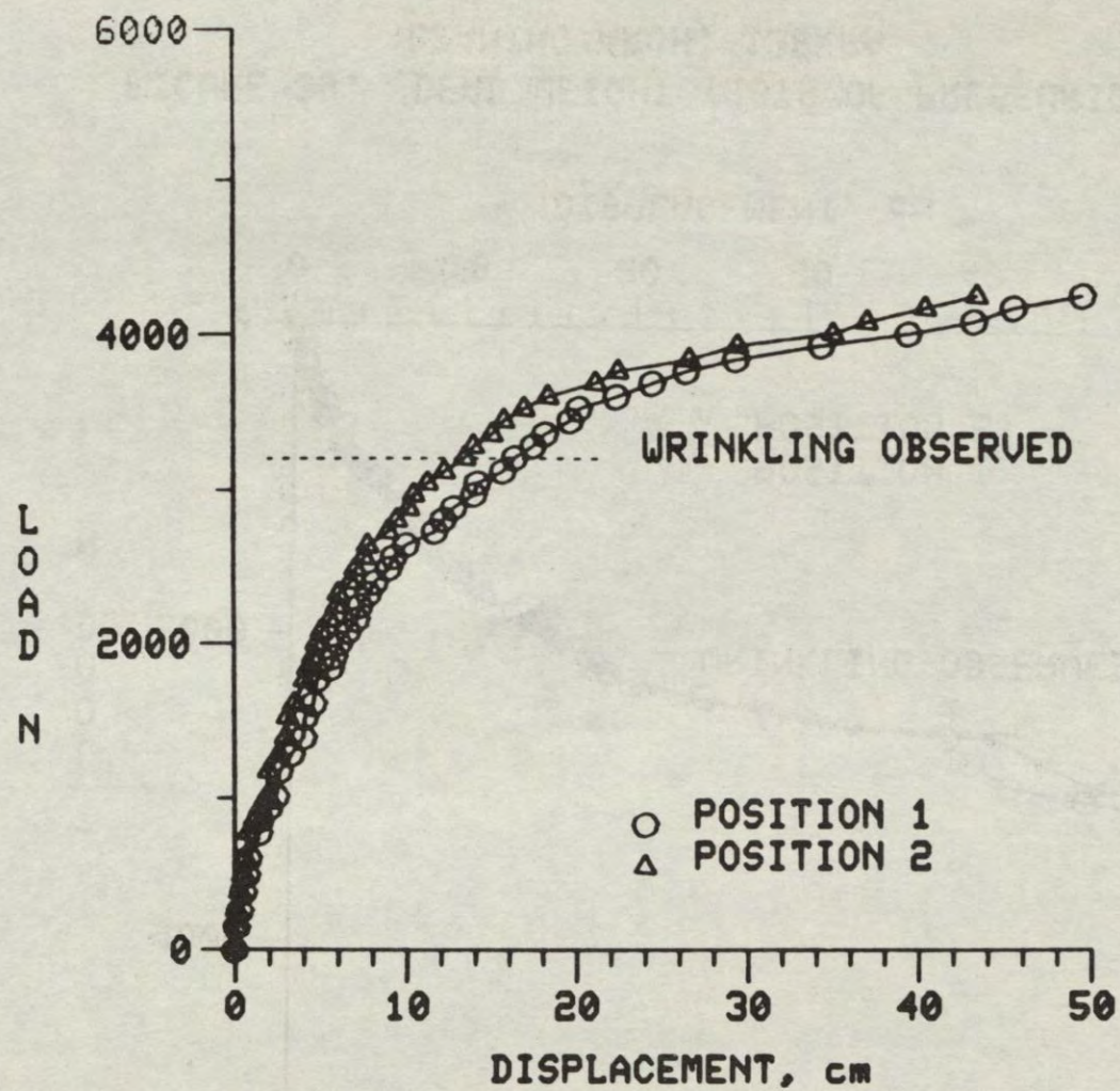
FIGURE 40. DEAD WEIGHT TESTS OF PRESSURIZED RIB TENTS LEANING ARCH, 207KPA
