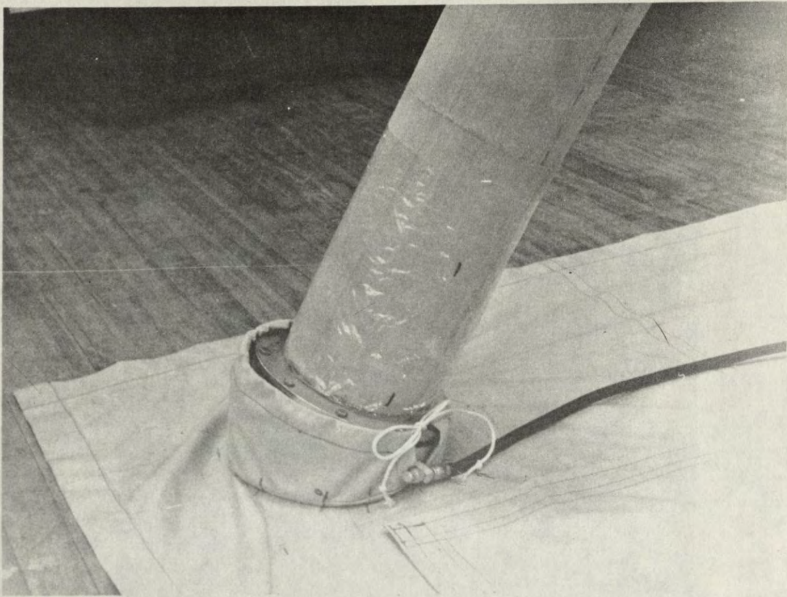
FIGURE 26. ATTACHMENT OF ARCH END CAP TO TENT FLOOR.
