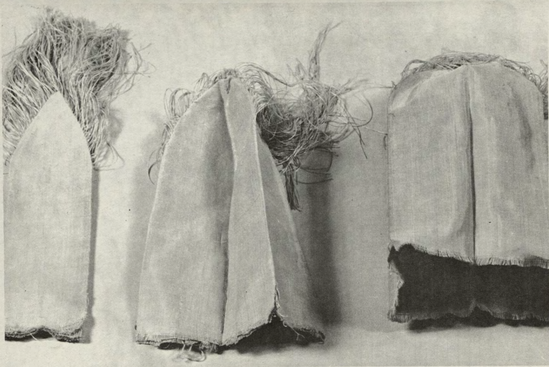
FIGURE 11. WOVEN HEMISPHERICAL END CAP IN VARIOUS STAGES OF UNFOLDING FROM WEAVING TO END USE CONFIGURATION.
