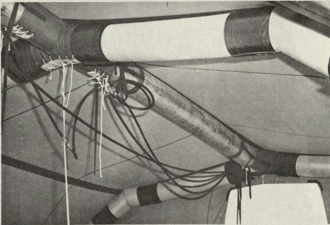
FIGURE 24. PHOTOGRAPH OF ARCH AND PURLIN CONNECTION.
