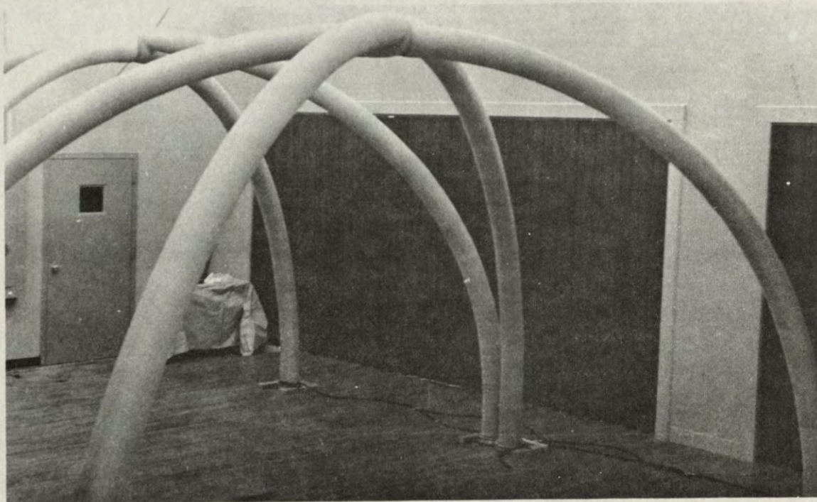
FIGURE 17. DOUBLE MODULE CROSSED ARCH FRAME ASSEMBLY.
