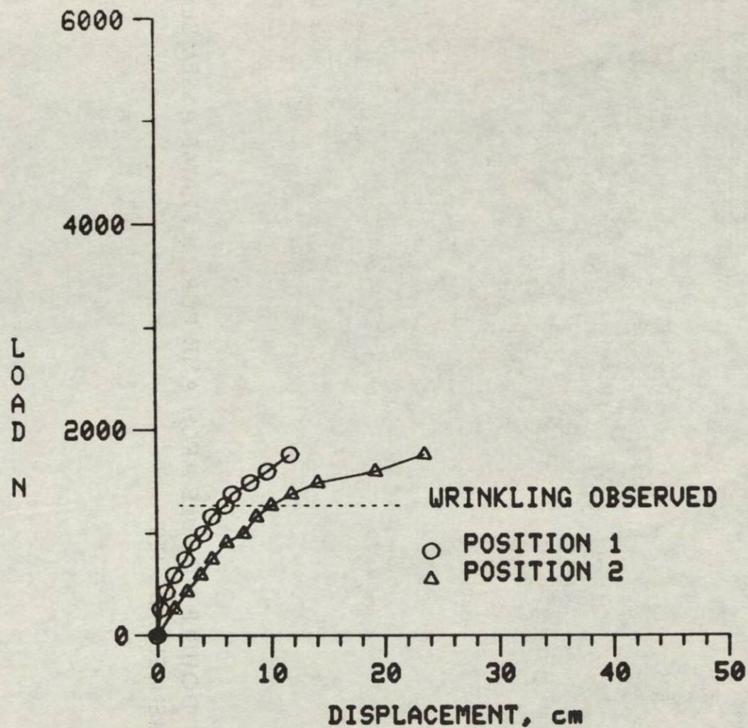
FIGURE 32. DEAD WEIGHT TESTS OF PRESSURIZED RIB TENTS CROSSED ARCH, 138KPA
