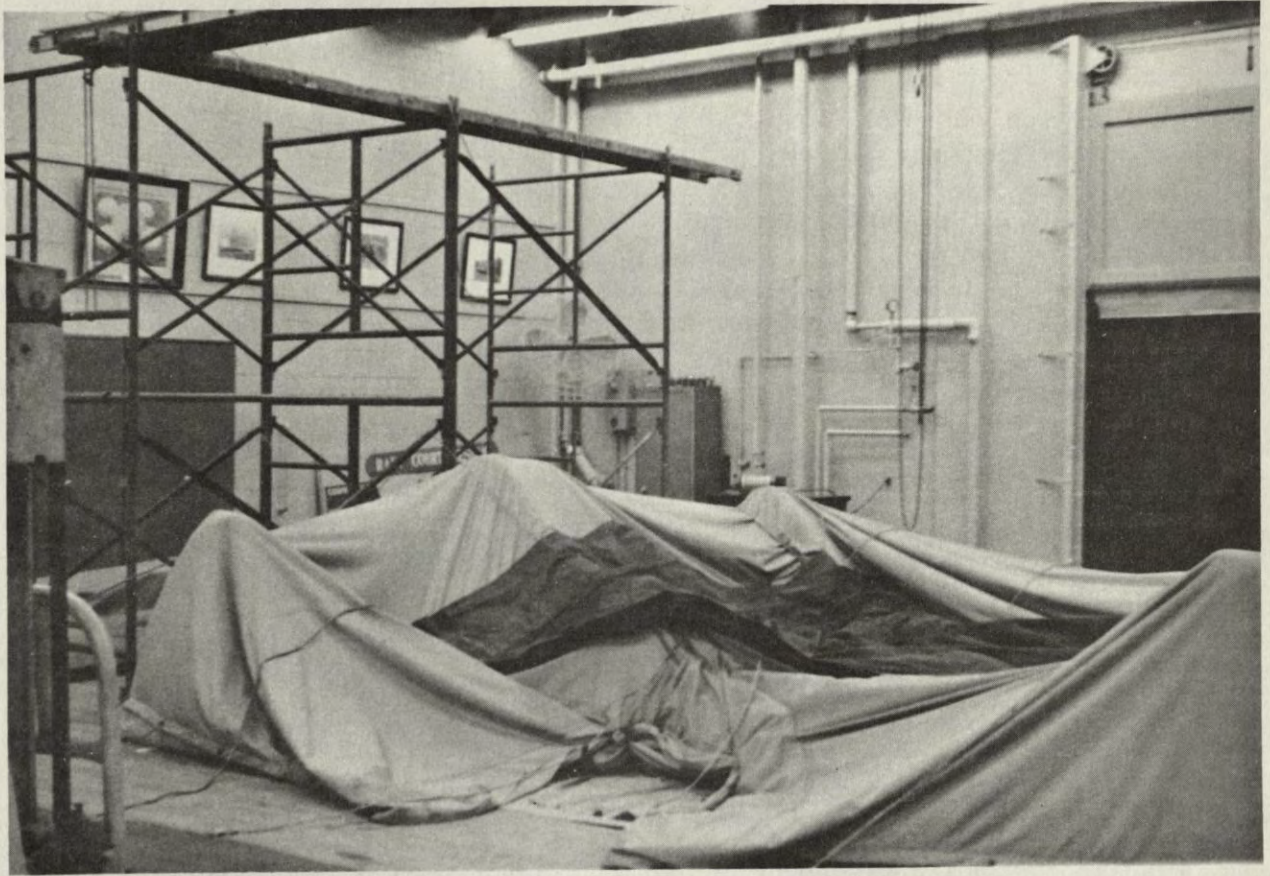
FIGURE 45. CROSSED ARCH PROTOTYPE TENT IN THE COLLAPSED STATE.
