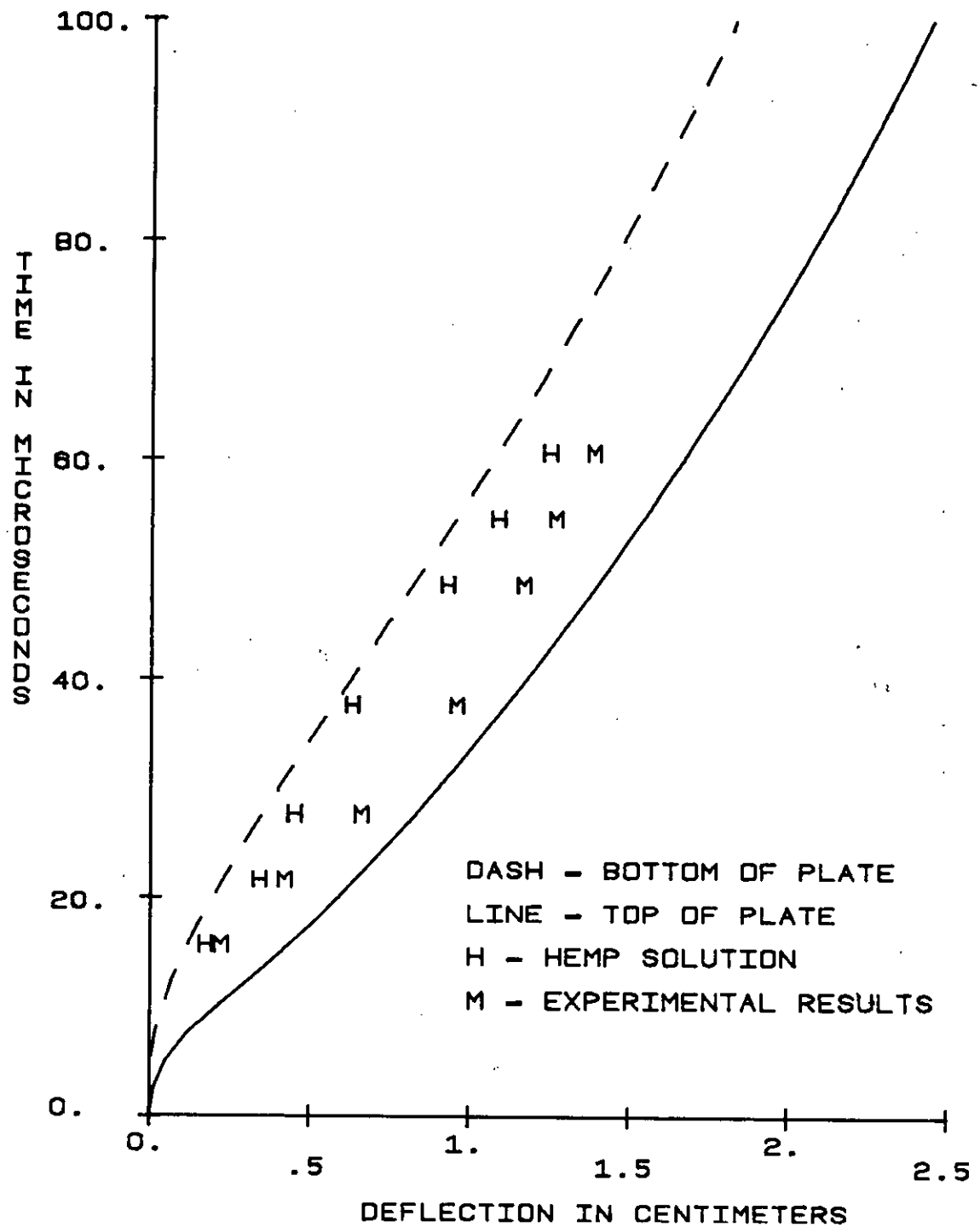
Figure 2. Numerical results for time increment of 2.5 \mu s
