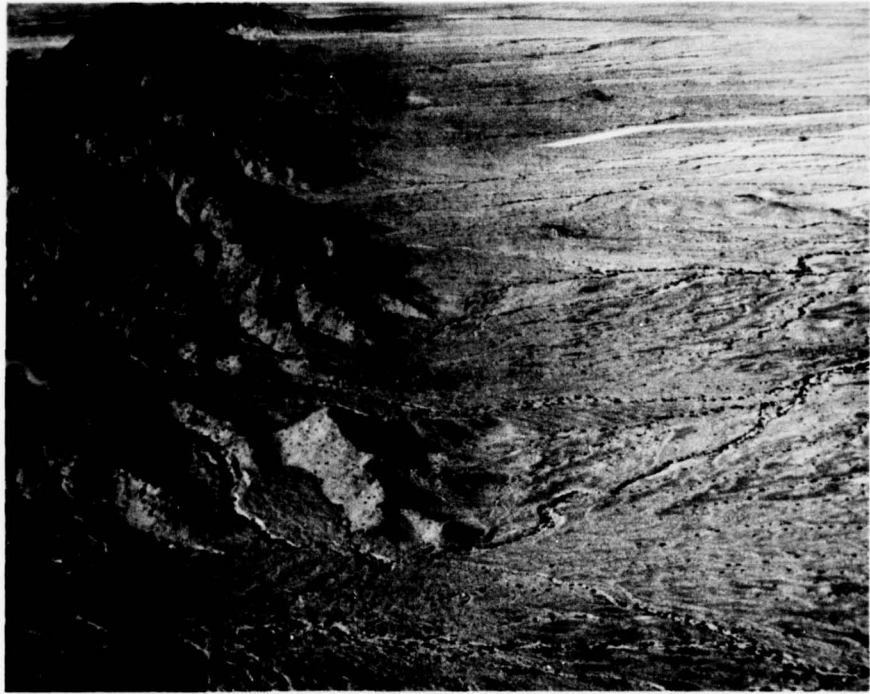
Figure 2:21 Mohawk Mountains front El. An erosional fault scarp running at a slight angle to the front can be seen in the mountains.
