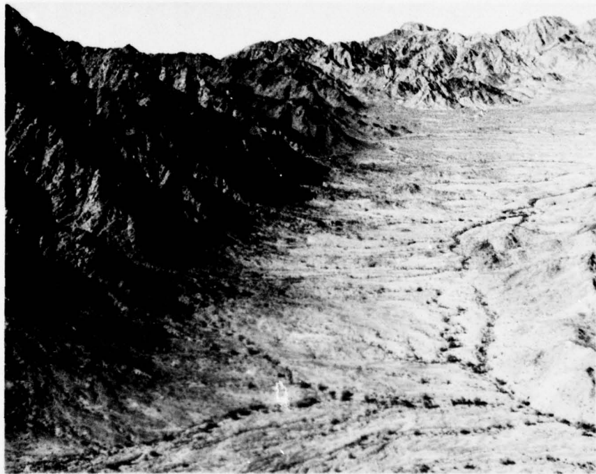
Figure 2:8 Gila Mountains front W2. View parallel to front.
