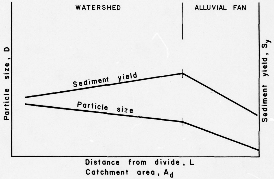
Figure 4:15 Changes in gravel particle size and sediment yield with distance from divide.
