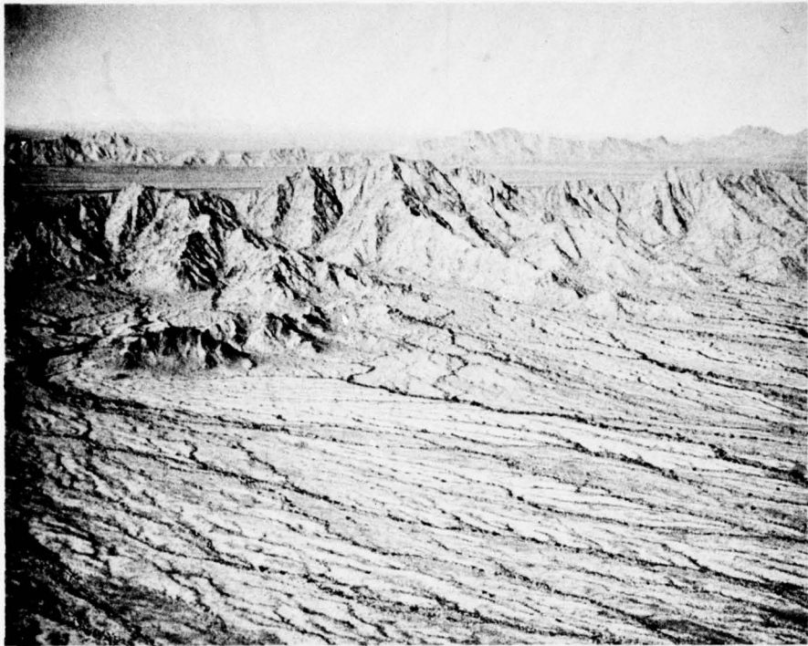
Figure 2:23 Granite Mountains front E. Class 3B.
