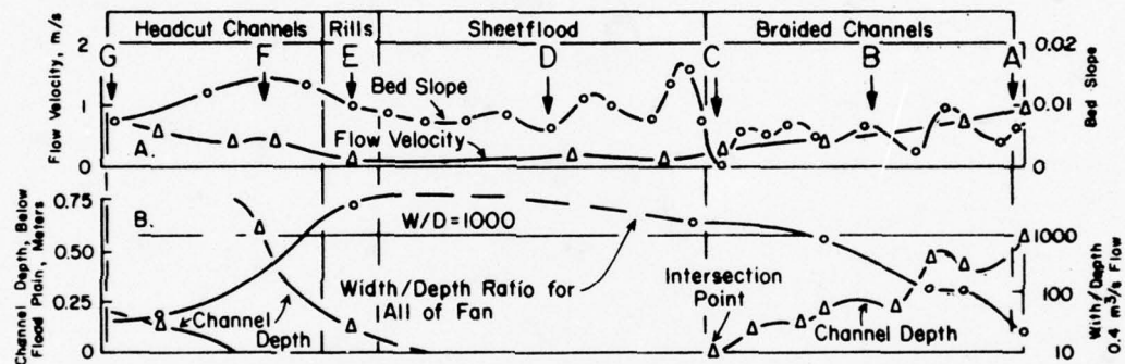
Figure 5 Summary of hydraulic data for the Dead Mesquite fan. After Packard, 1974, Figure 26
