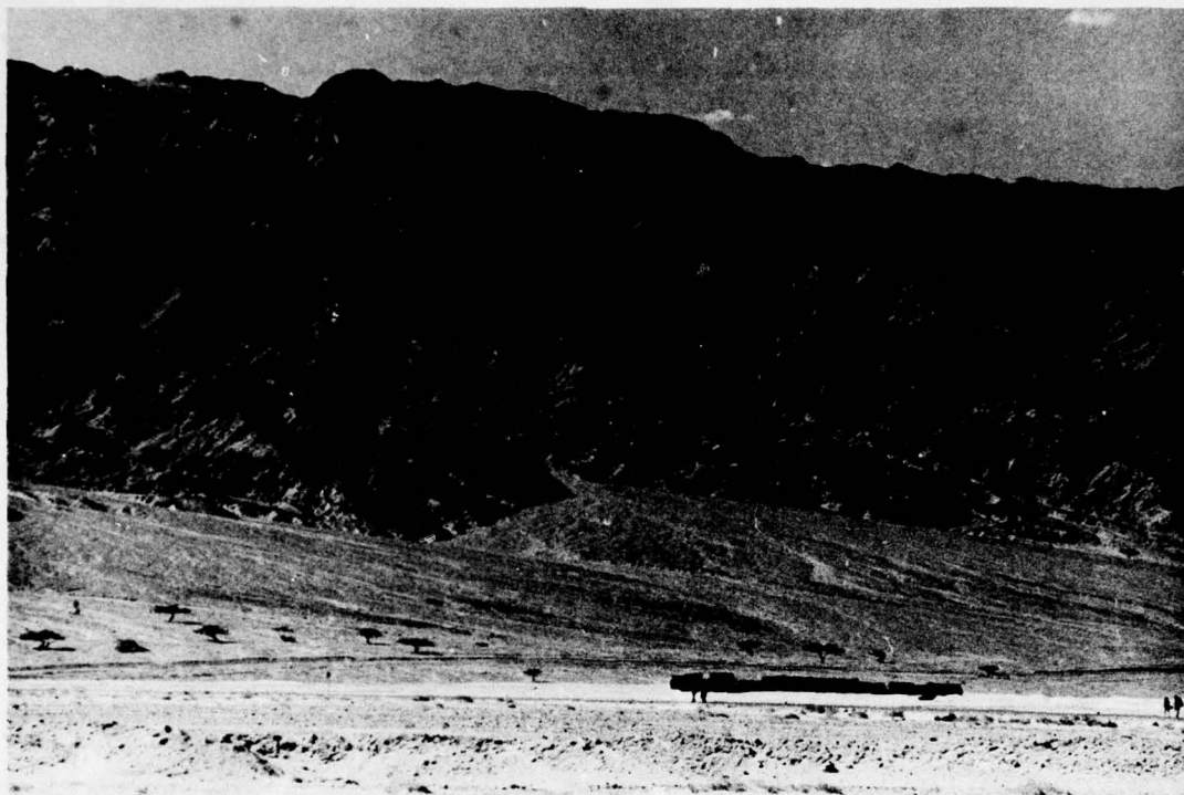
Figure 16 Unentrenched alluvial fans along the east side of the Sinai Peninsula west of the Neviot. The rapid rate of accumulation of these fans can be described by Equation 5 of the text.
