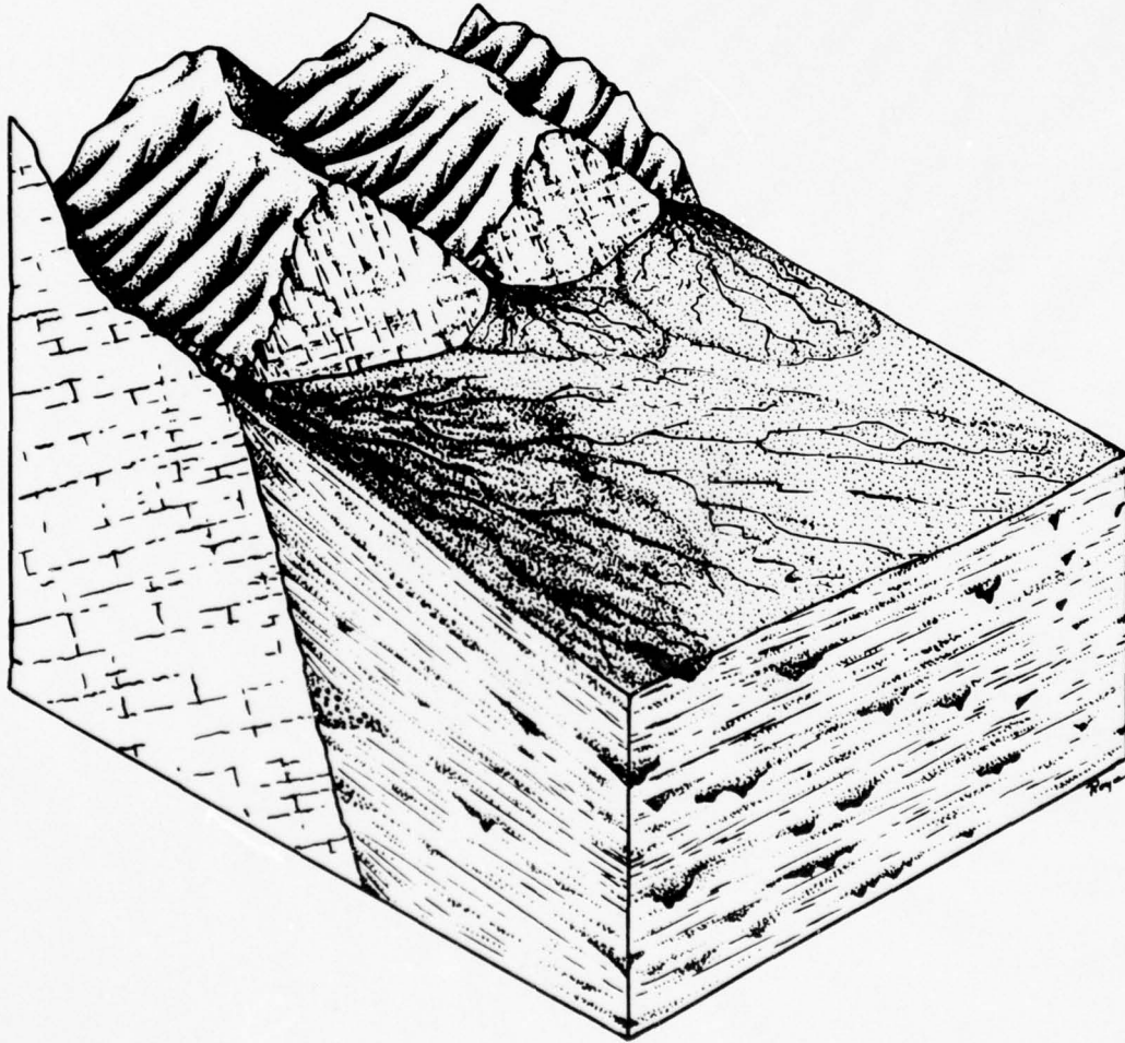
Figure 10 A diagrammatic sketch showing the internal structure of a typical alluvial fan.
