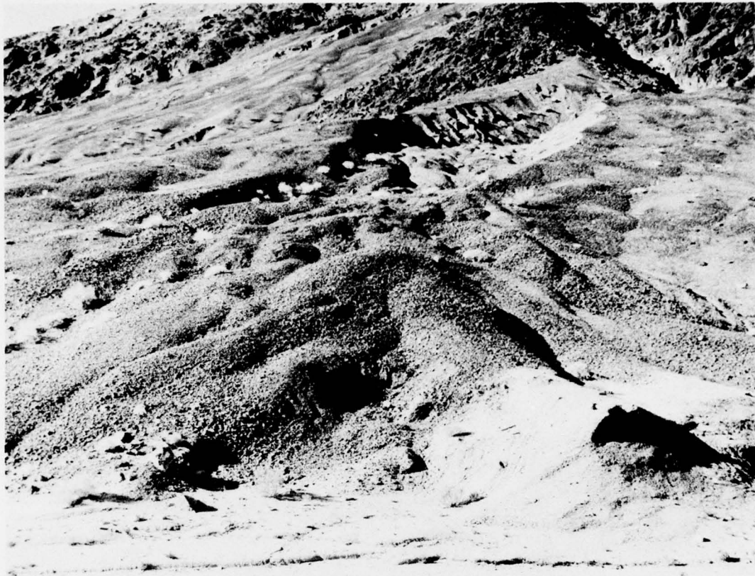
Figure 7 Alluvial fan formed by sieve deposition, Eureka Valley, California. a Hummocky topography formed by sieve-deposit lobes. The slope is 16^\circ along the medial radial line, and is 20' in the area of older and smoother fan surface to the right of the fanhead trench.
