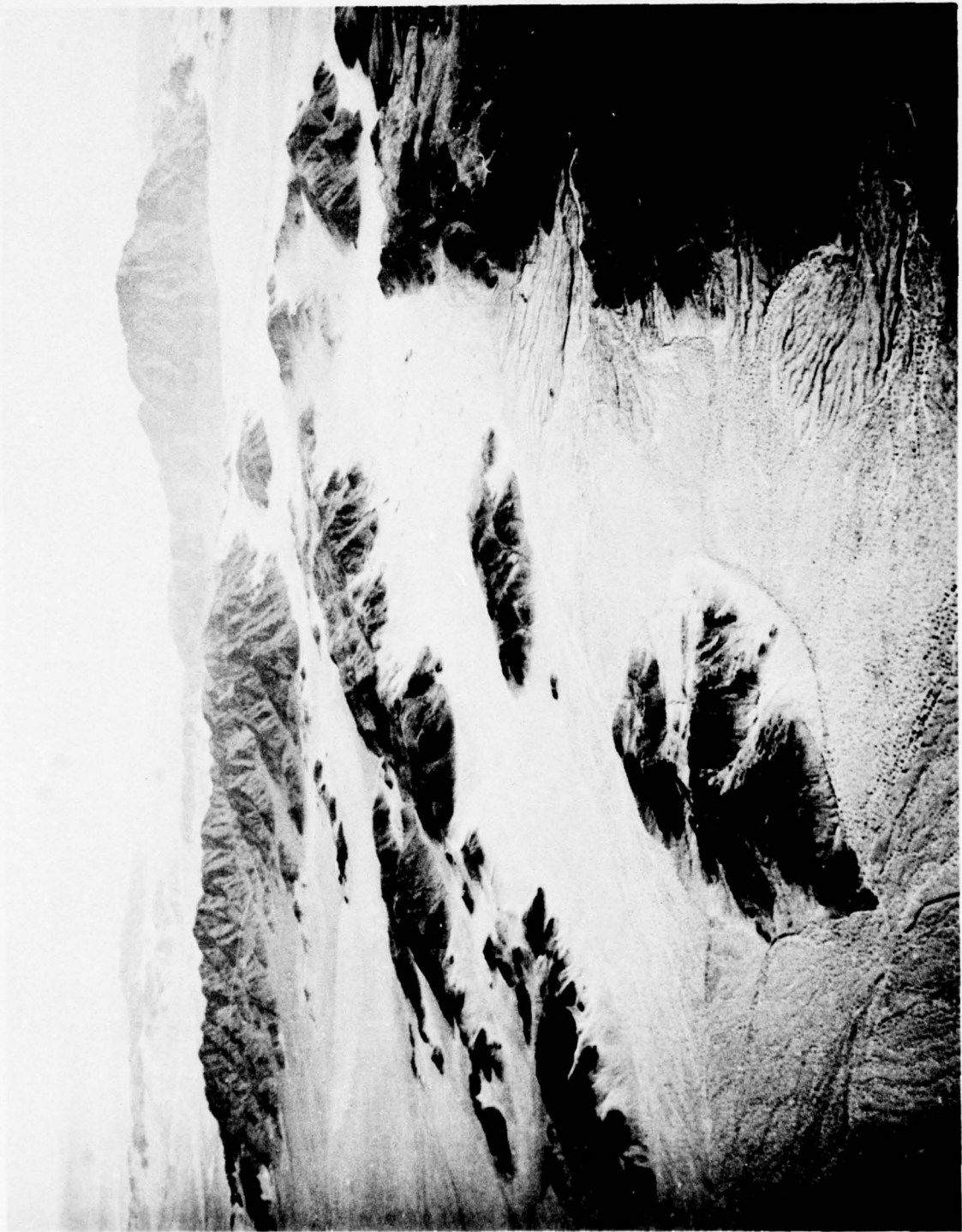
Figure 6. Class 3 terrain southeast of the Tiefert Mountains. Soda Mountains are in the background.
