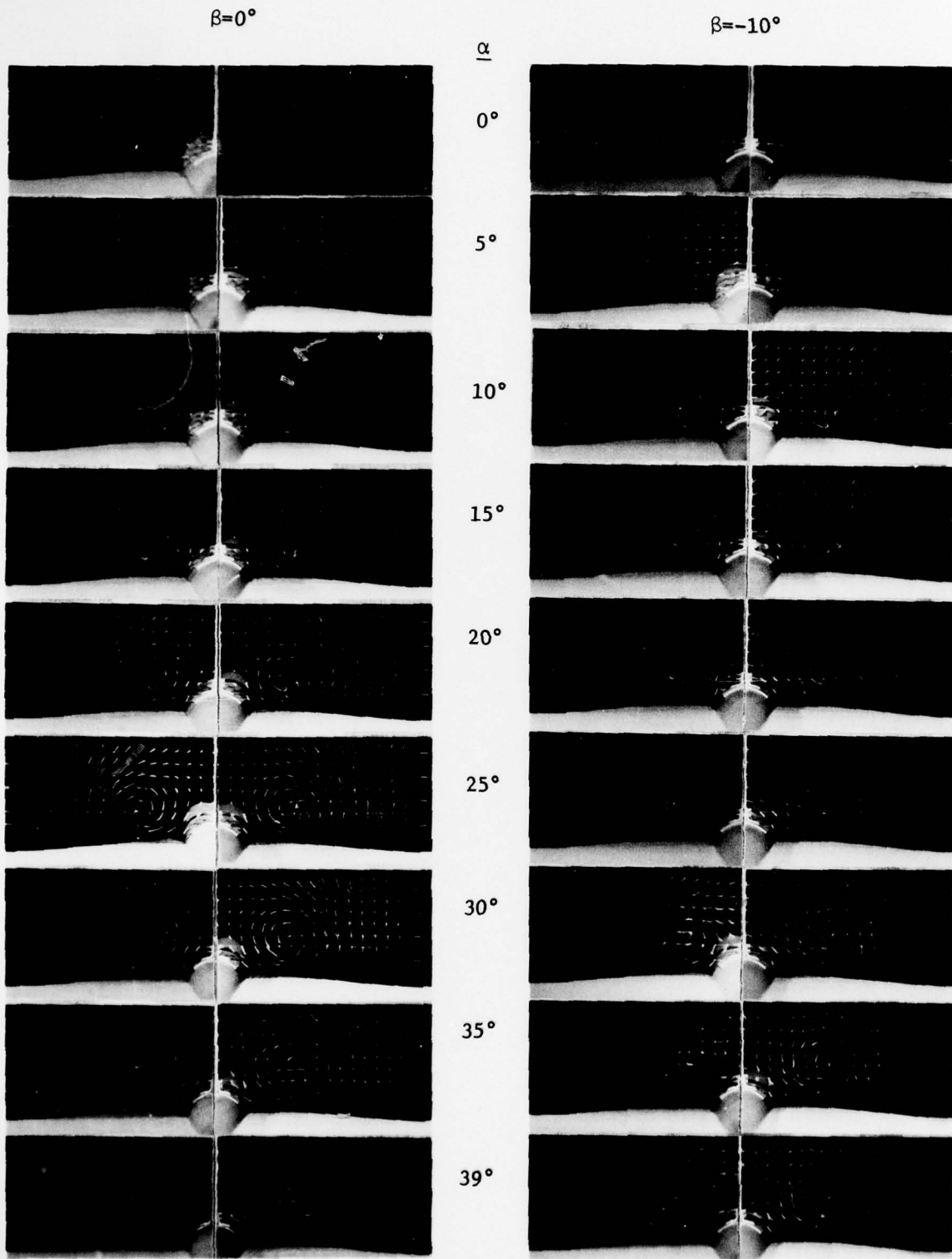
Figure A.1a - Baseline 75^\circ LEX, High Wing Configuration, Grid Position 35
