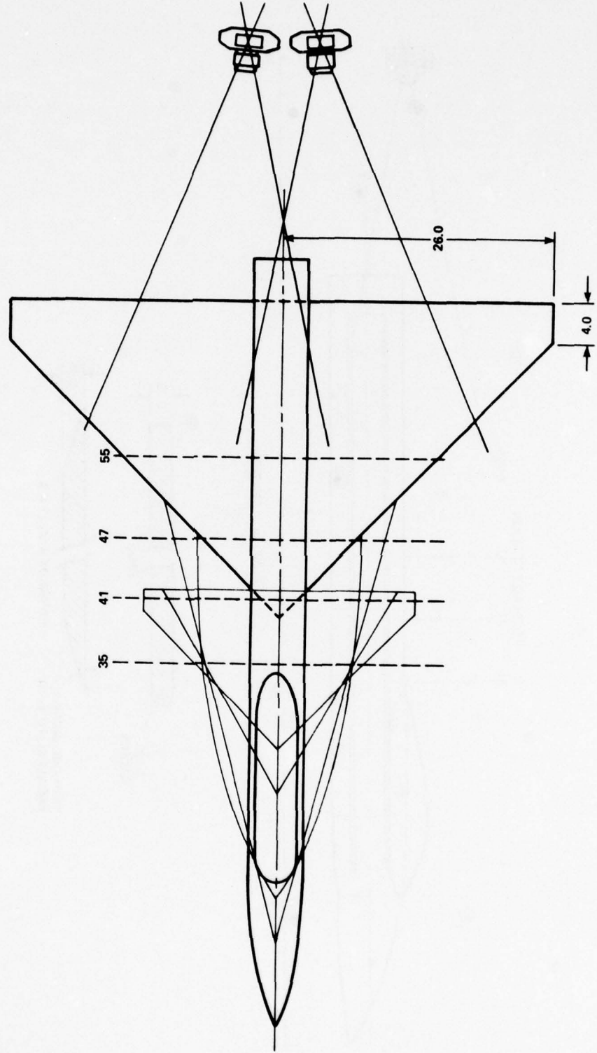
Figure 1 - Three Views of Model (Dimensions are in inches)
