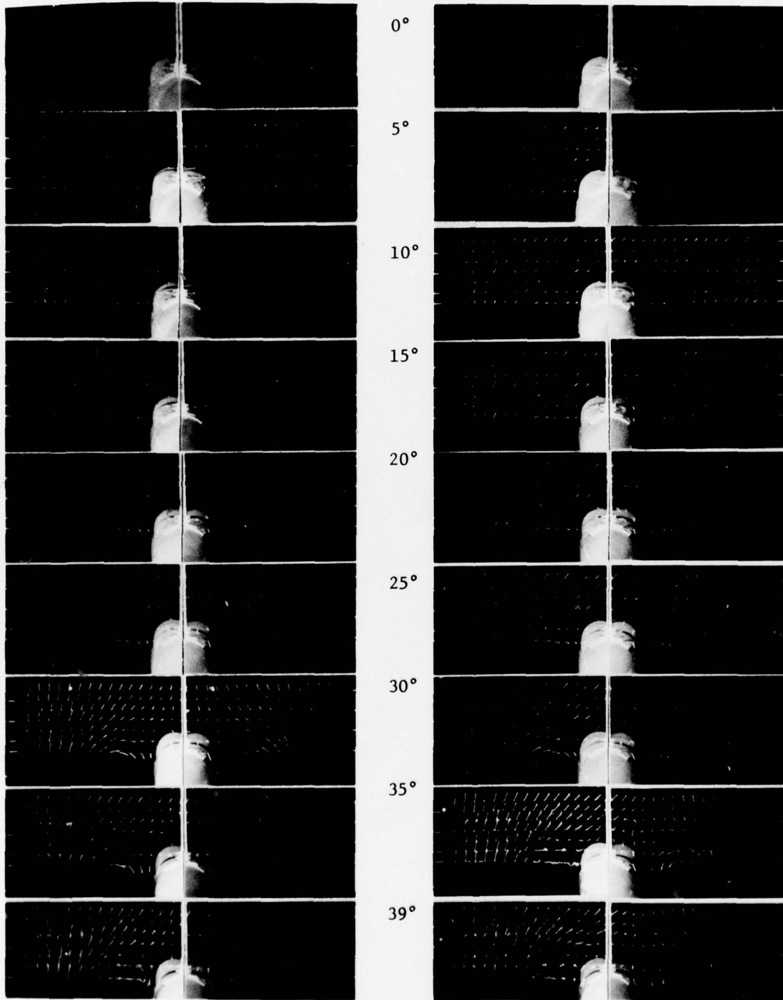
Figure A.5a - 75^\circ LEX, Low Wing Configuration, Grid Position 35
