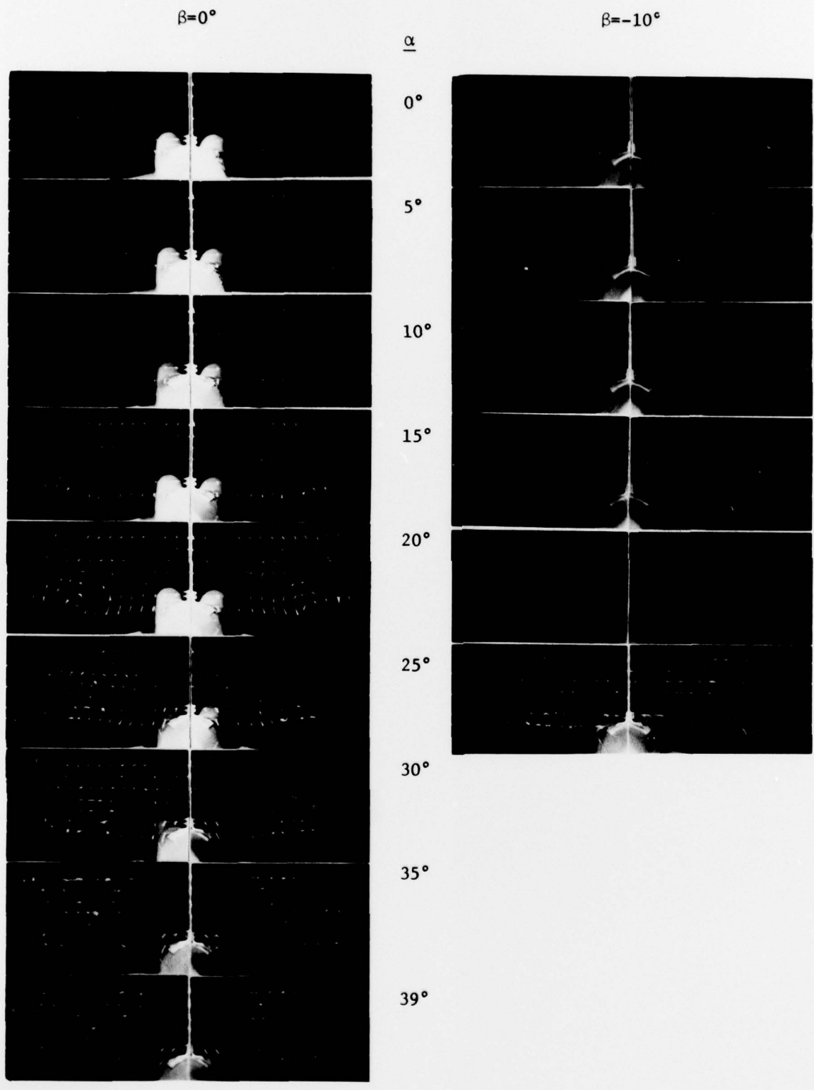
Figure A.5d - 75° LEX, Low Wing Configuration, Grid Position 55
