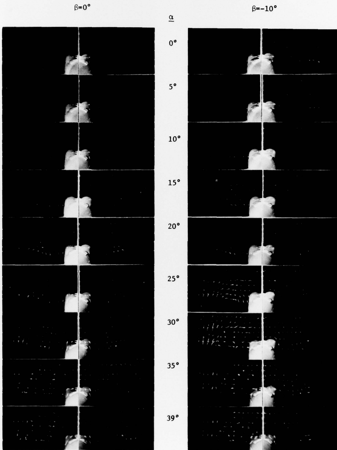
Figure A.5c - 75° LEX, Low Wing Configuration, Grid Position 47
