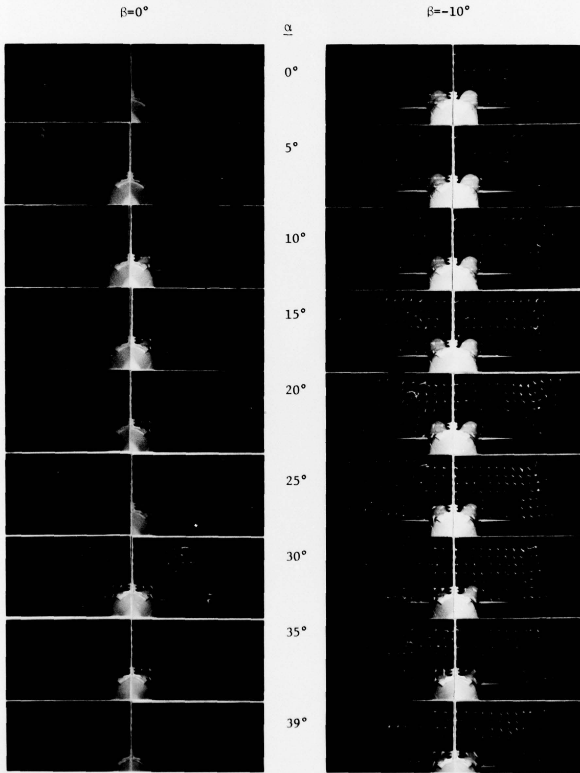
Figure A.6d - 60° Close Coupled Canard Configuration, Grid Position 55
