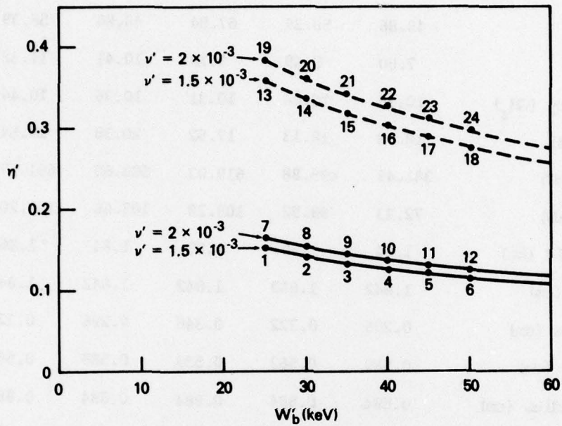
Fig. 1 - Beam frame efficiency \eta' versus beam energy W'_b . Solid curves are for X' = 1 and dashed curves are for X' = X'_h .
