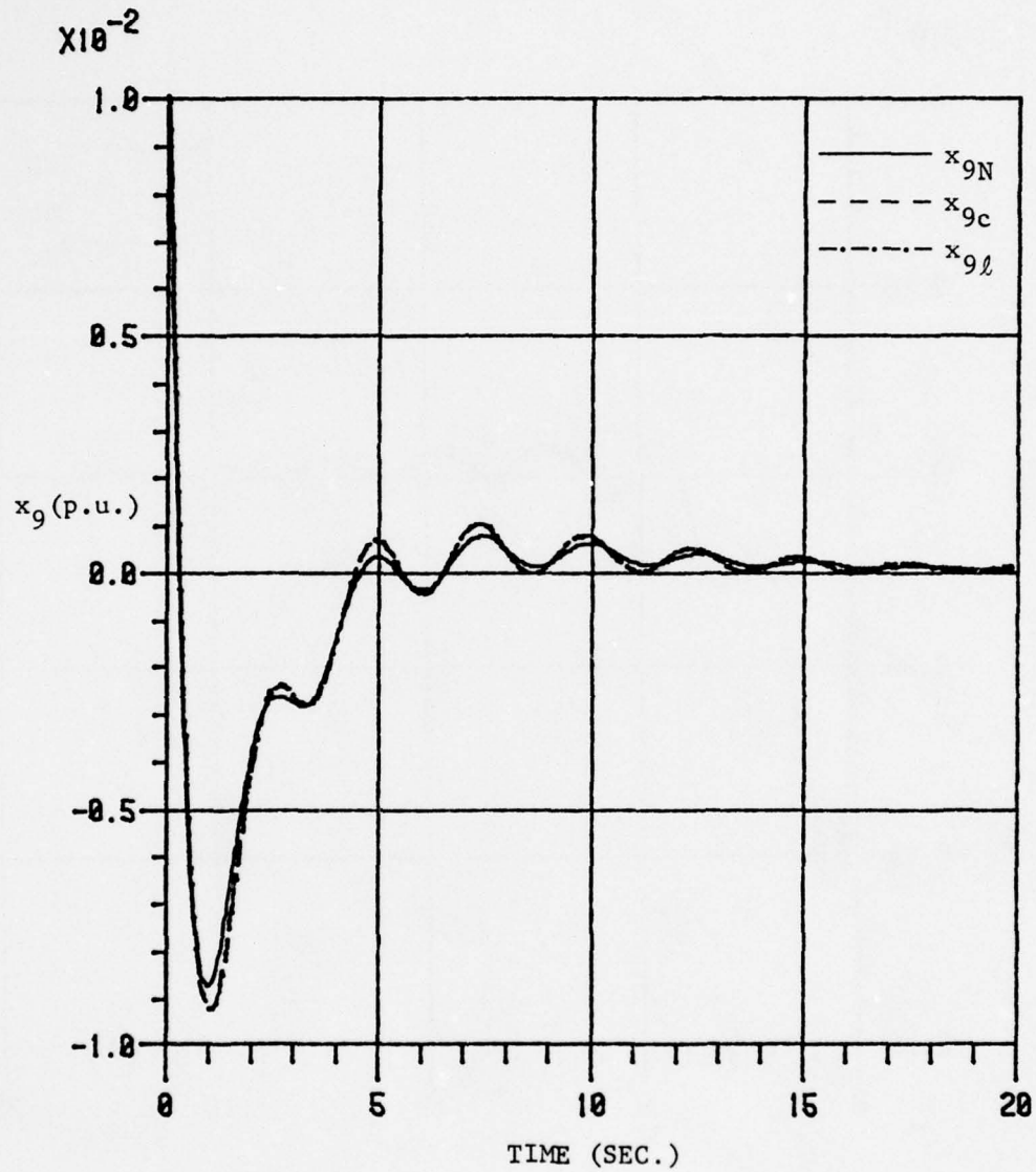
Figure 4.9. Closed-loop state variation for turbine two output power variation for Nash, composite and lower order control application.
