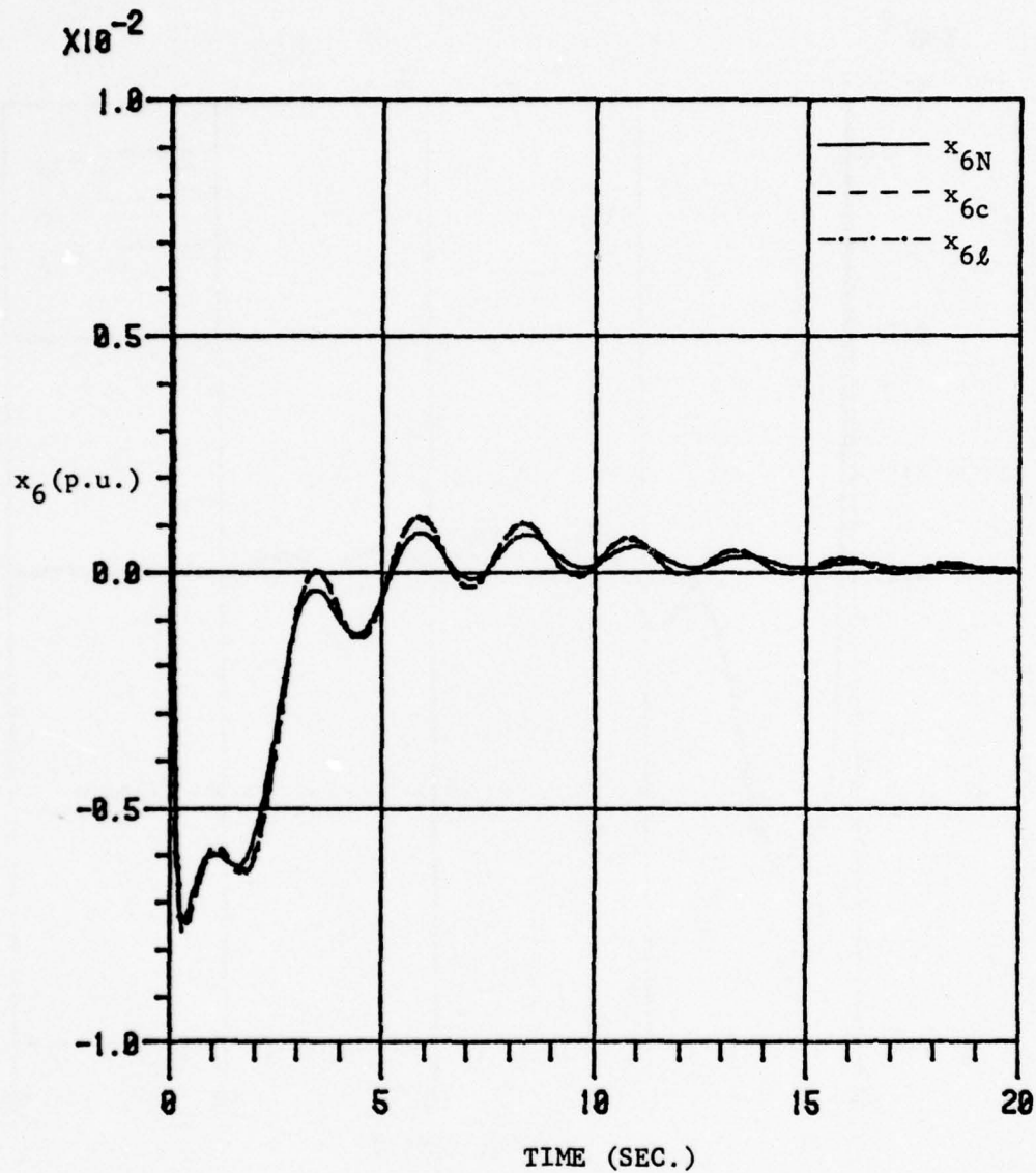
Figure 4.6. Closed-loop state trajectories for turbine one valve position variation for Nash, composite and lower order control application.
