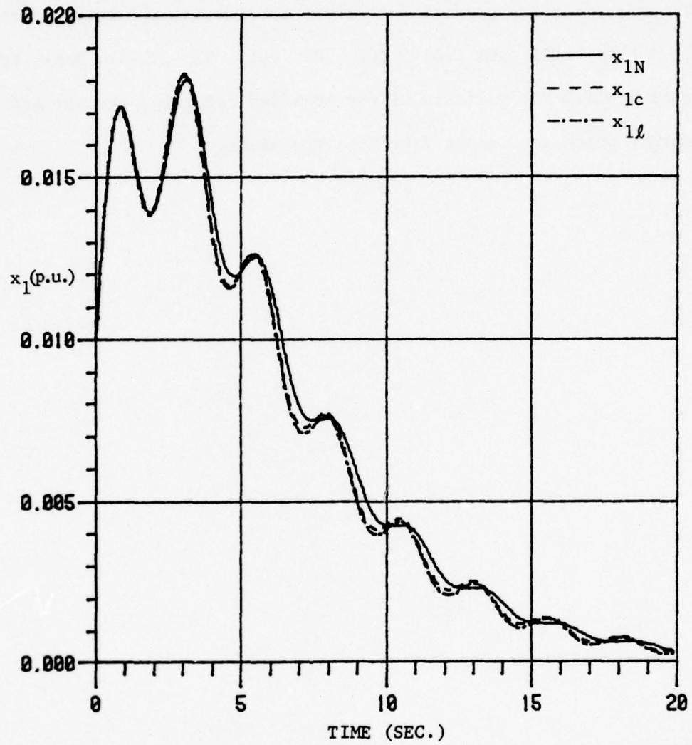
Figure 4.1. Closed-loop state trajectories for the integral of the area control error for area 1 for Nash, composite and lower order control applications.
