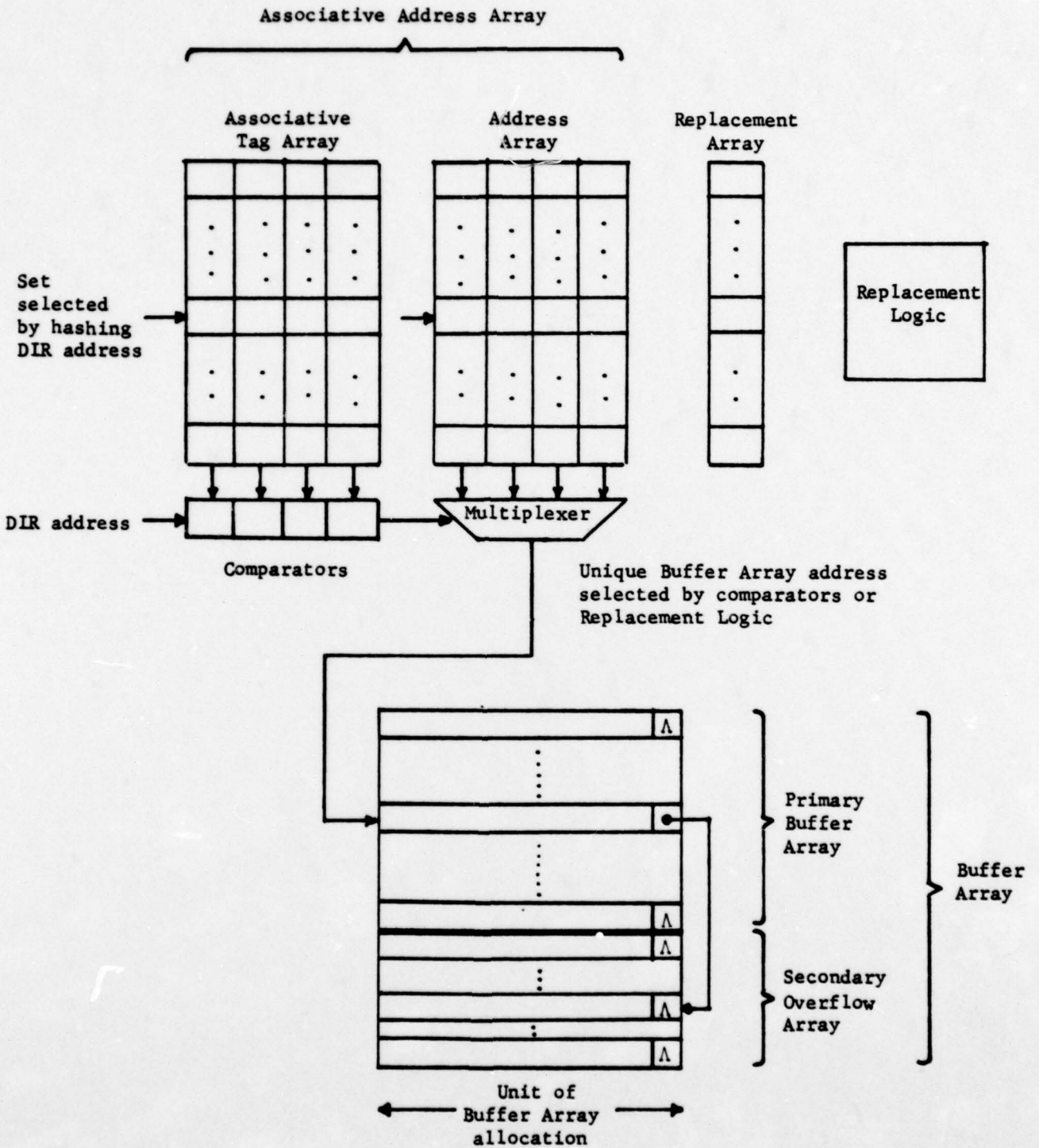
Figure 2. Organization of the Dynamic Translation Buffer.
